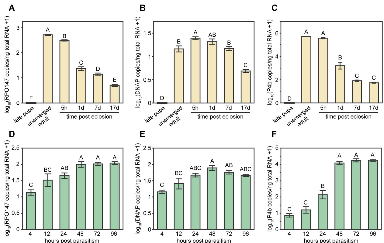
Fig 4. DIEPV gene expression profiles for selection of RNA-seq timepoints. Expression of DIEPV genes measured with RT-qPCR in (A–C) female wasp venom glands from late pupa to 17-day-old adult and (D–F) parasitized flies from 4–96 hours post parasitism (hpp). Profiled DIEPV genes encode (A,D) the 147kDa RNA polymerase subunit RPO147, (B,E) the DNA polymerase DNAP, and (C,F) the structural protein P4b. Each bar represents the mean \log_{10} transformed cDNA copy number per ng total RNA averaged from 6 biological replicates. Error bars represent one standard error above and below the mean, and the letter(s) above each bar indicates statistically distinct mean values from Tukey's HSD tests. Data in (A–C) were modified from Coffman et al. 2020 [34].
