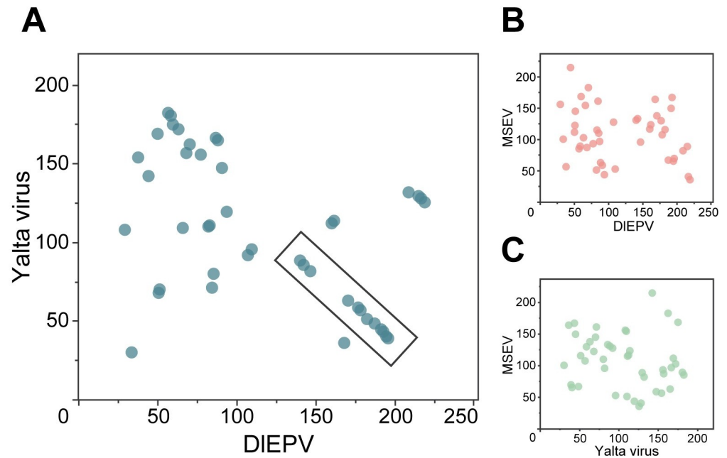
Fig 3. Core gene synteny further supports the close relationship between DIEPV and Yalta virus. Dot plots show the relative genomic location of the 44 poxvirus core genes shared between the DIEPV and Yalta virus genomes when compared to (A) one another, or (B-C) when either is compared to MSEV. Each dot represents a homologous core gene, and axes indicate the genomic position in kilobases. Box in panel A highlights a highly syntenic region between DIEPV and Yalta virus core genes.
