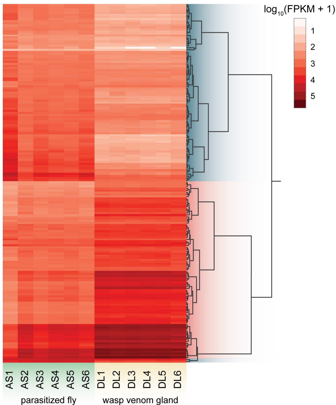
Fig 5. DIEPV shows widespread differential expression during replication in D. longicaudata wasps compared to A. suspensa flies. Heatmap showing significantly ( \text{FDR } q < 0.05 ) differentially expressed DIEPV genes in wasp and fly tissue. Each row represents a DIEPV gene, and each column represents that gene's expression in each of the 12 RNA samples. Expression is depicted as the \log_{10} transformed FPKM value. Columns AS1-6 correspond to the 6 parasitized fly RNA replicates, and DL1-6 correspond to the 6 wasp venom gland replicates. Rows were clustered using the Ward method based on similarity in gene expression pattern across the 12 samples: DIEPV genes that were significantly downregulated in wasp tissue are highlighted in blue, and genes that were significantly upregulated in wasp tissue are highlighted in pink.
