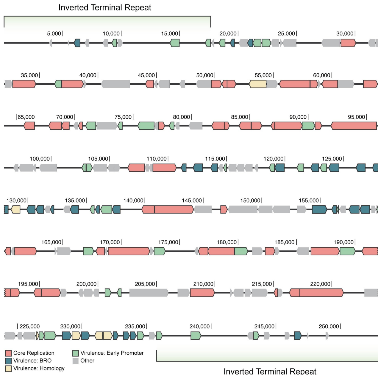
Fig 1. Linear map of the DIEPV genome. Each arrow indicates the genomic position of a DIEPV ORF, and the direction of the arrow corresponds to its strand orientation. Arrows are colored based on the putative functional category of each ORF as defined in the legend at the bottom of the map. Core Replication refers to the 45 poxvirus core genes identified in the DIEPV genome. Virulence: BRO refers to the 27 DIEPV BRO genes, Virulence: Homology indicates the 6 ORFs with similarity to known virulence genes, and Virulence: Early Promoter are the additional 34 putative virulence genes based on the presence of the conserved EPV early promoter sequence and no other assigned function.
