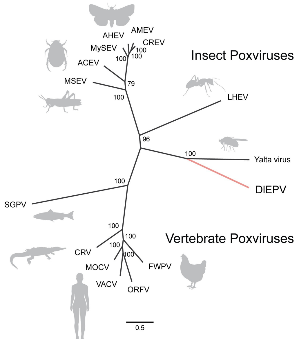
Fig 2. Poxvirus core gene phylogeny demonstrates that the fly-infesting Yalta virus is the closest known relative of DIEPV. Phylogenetic tree constructed from a maximum likelihood analysis using the concatenated amino acid multiple sequence alignment from 16 conserved poxvirus core genes. Node support (%) was inferred with 1,000 bootstrap iterations. Insect and vertebrate poxvirus orthologs used to build the phylogeny are indicated in S3 Table . Genome abbreviations are as defined in the Results section, and accessions are included in the Materials and Methods section.
