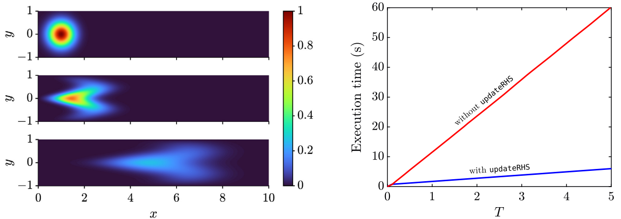
Fig. 5.5. (Left) Snapshots of the solution to the convection-diffusion equation (5.4) at times t=0 , t=1 , and t=5 , computed using ultraSEM in space and backward Euler in time. (Right) The execution time required to simulate (5.4) over the time span [0, T] , by either reconstructing the operators from scratch at each time step (red) or updating the particular solution using updateRHS (blue).
