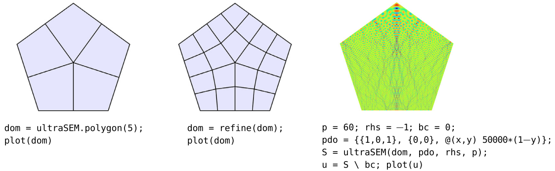
Fig. 4.2. A simple example of the syntax in ultraSEM . A pentagonal domain (with side length 1.2) is meshed into five quadrilaterals (left) and uniformly refined (center). The gravity Helmholtz equation \nabla^2 u + 50000(1-y)u = -1 with zero Dirichlet boundary conditions is then solved on the mesh using polynomials of degree 60 on each element (right).
