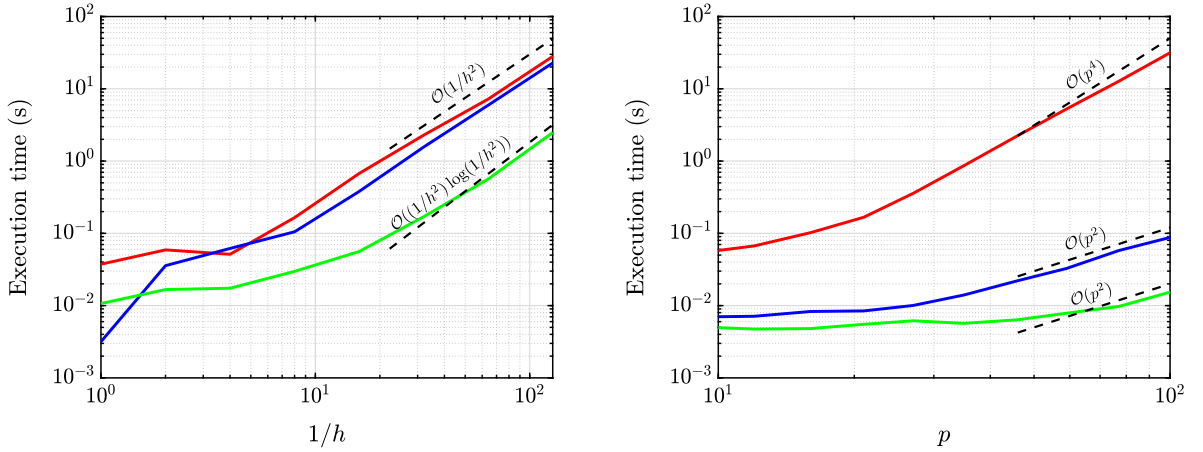
Fig. 5.1. Execution time (in seconds) for ultraSEM over a range of mesh sizes (left) and polynomial orders (right). Timings are depicted for the local build stage (red), global build stage (blue), and solve stage (green), when solving the PDE \nabla^2 u + \sin(xy)u = f on the domain \Omega = [0, 1]^2 with spatially varying right-hand side and spatially varying Dirichlet boundary conditions. On the left, we successively refine a Cartesian mesh while keeping the polynomial order fixed at p = 4 . On the right, we use a 4 \times 4 Cartesian mesh while successively increasing the polynomial order.
