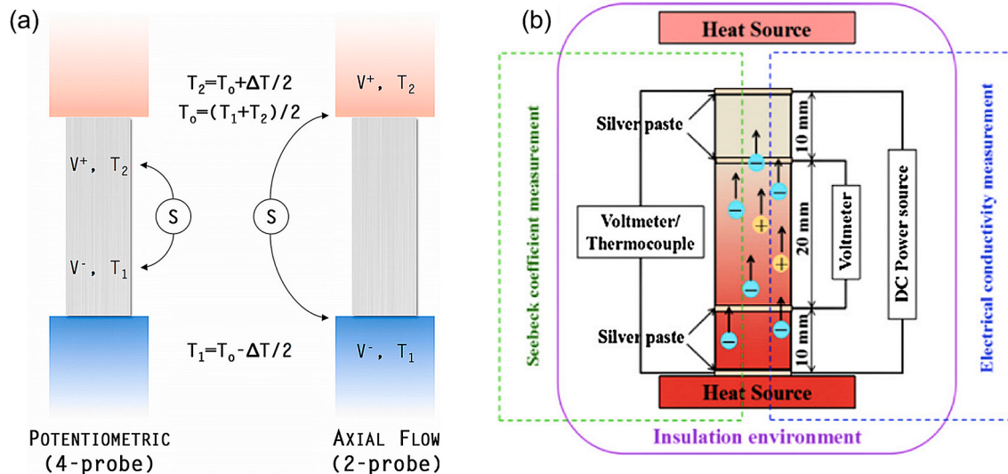
Fig. 7. (a) Potentiometric and axial flow methods for Seebeck coefficient measurements (sourced from Ref. [99]), and (b) an example of Seebeck measurement for TE cement (sourced from Ref. [57]).
