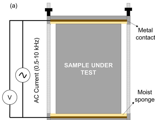
Fig. 2. (a) Uniaxial method and (b) four-probe method for electrical resistivity measurement (reproduced from Ref. [62]).
