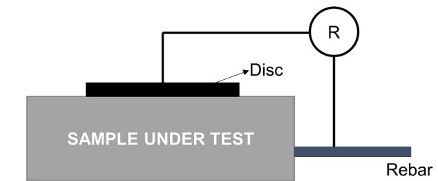
Fig. 3. Surface Disc method for electrical resistivity measurement (reproduced from Ref. [63]).
