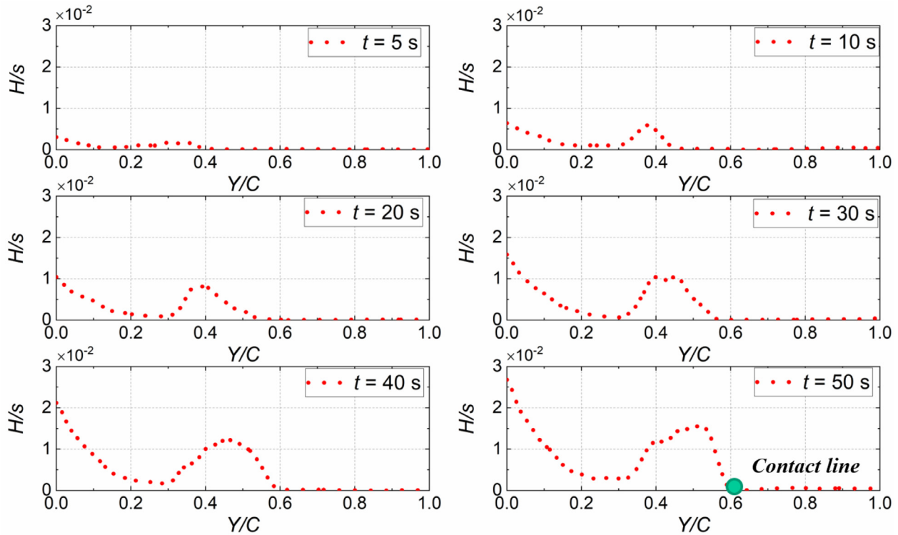
Fig. 8. Time evolutions of the water/ice thickness over the airfoil surface along the streamwise direction when V_\infty = 15 m/s and AoA = 5^\circ .
