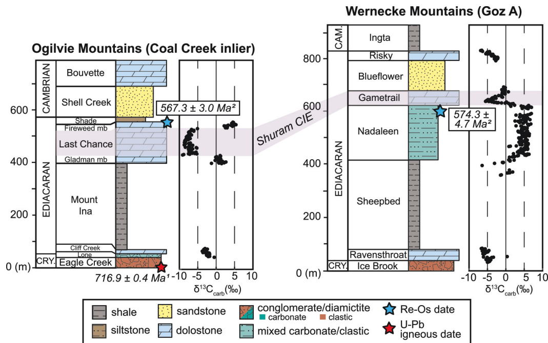
Fig. 11. Newly formalized Ediacaran–Cambrian units of the Coal Creek inlier shown with correlative Ediacaran–Cambrian strata of the Goz A region of the Wernecke Mountains; \delta^{13}\text{C}_{\text{carb}} data shown for all carbonate units with the location of the Shuram carbon isotope excursion (CIE) highlighted between the two locations (modified after Macdonald et al. 2013 and Rooney et al. 2020). 1 Macdonald et al. 2013, 2 Rooney et al. 2020. [Color online.]
