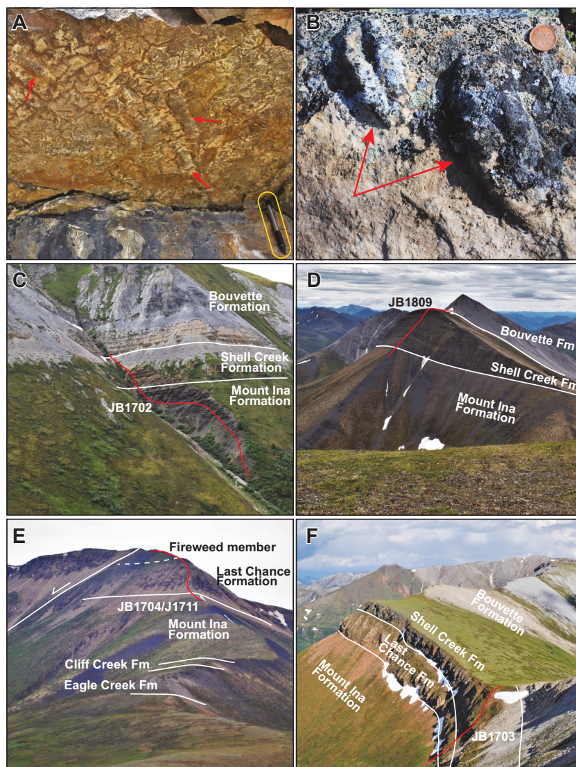
Fig. 6. (A) Base of a sandstone bed in the Shell Creek Formation with abundant complex trace fossils, including Cruziana (red arrows), Planolites , and other indeterminate ichnogenera; pencil in yellow is 13 cm long. (B) Rusophycus trace fossils on a float block from the Shell Creek Formation; coin is 1.8 cm in diameter. (C) Measured section JB1702 in the northern part of the study area where proximal facies of the Shell Creek Formation sit unconformably on the Mount Ina Formation. (D) Measured section JB1809 in the western part of the study area where distal facies of the Shell Creek Formation rest unconformably on the Mount Ina Formation. (E) Measured sections JB1704/J1711 of the Last Chance Formation overlying the type section of the Mount Ina Formation (F838, Macdonald et al. 2013). (F) Measured section JB1703 where the Shell Creek Formation sits unconformably on the Last Chance Formation. [Color online.]
