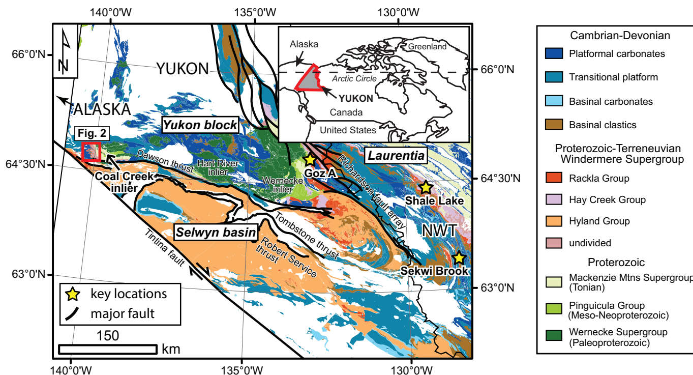
Fig. 1. Simplified geological map of Proterozoic–Paleozoic strata in northwestern Canada with major structural and paleogeographic elements labeled accordingly. The study location is outlined with a red box. Map created using ESRI ArcGIS version 10.7.1 and assembled from Colpron et al. (2016). [Color online.]
