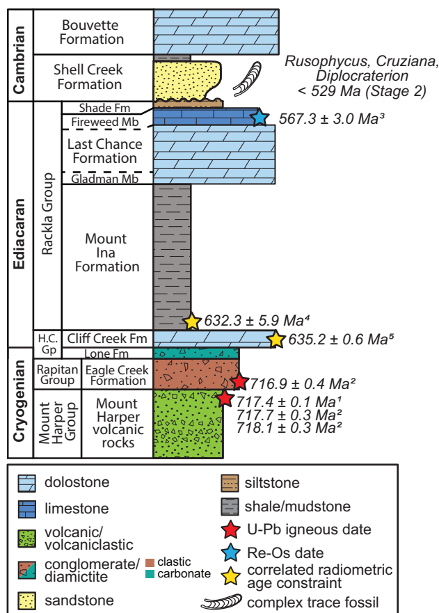
Fig. 2. Generalized stratigraphic column of Cryogenian–Cambrian strata in the Coal Creek inlier of west-central Yukon ( 1 Macdonald et al. 2018, 2 Macdonald et al. 2010, 3 Rooney et al. 2020, 4 Rooney et al. 2015, 5 Condon et al. 2005). [Color online.]
