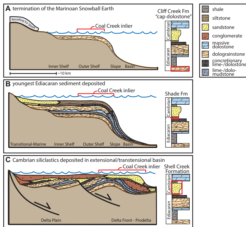
Fig. 12. Schematic model for Ediacaran–Cambrian basin evolution of the Coal Creek inlier. Note stratigraphic thicknesses are not to scale and facies distributions are inferred outside of the “Coal Creek inlier” extent (shown with red bar). Tilting of strata in panel C is exaggerated for illustration purposes. (A) Basal Ediacaran Cliff Creek Formation “cap dolostone” is deposited during postglacial transgression within an outer shelf setting. (B) Upper Ediacaran fine-grained siliciclastic rocks and concretionary carbonate of the Last Chance and Shade formations are deposited in an outer shelf to upper slope setting. (C) Syn-tectonic coarse- to fine-grained siliciclastic rocks of the Shell Creek Formation are deposited in a wave-influenced deltaic environment within a transtensional or extensional basin following block rotation and uplift that produced the angular “sub-Shell Creek” unconformity. [Color online.]
