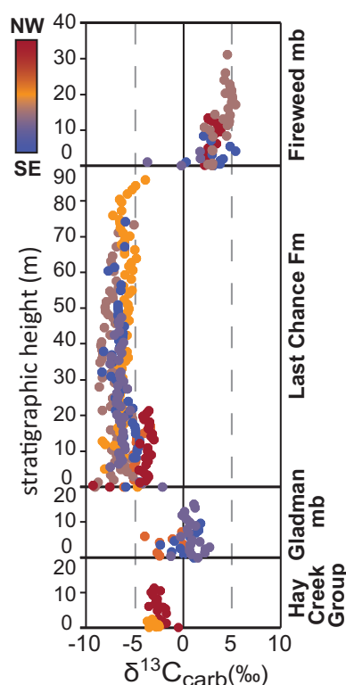
Fig. 10. Compilation of all \delta^{13}\text{C}_{\text{carb}} data from the Lone, Cliff Creek, and Last Chance formations measured for this study with data colored by relative location in the study area. No spatial trend is obvious in the Hay Creek Group and Gladman or Fireweed members of the Last Chance Formation, but there is a ca. 5‰ gradient in the most depleted values of the Last Chance Formation between the northwestern (J1710) and southeastern (JB1704) stratigraphic sections. These highly depleted \delta^{13}\text{C}_{\text{carb}} values in the Last Chance Formation are correlated with the globally recognized Shuram carbon isotope excursion. [Color online.]
