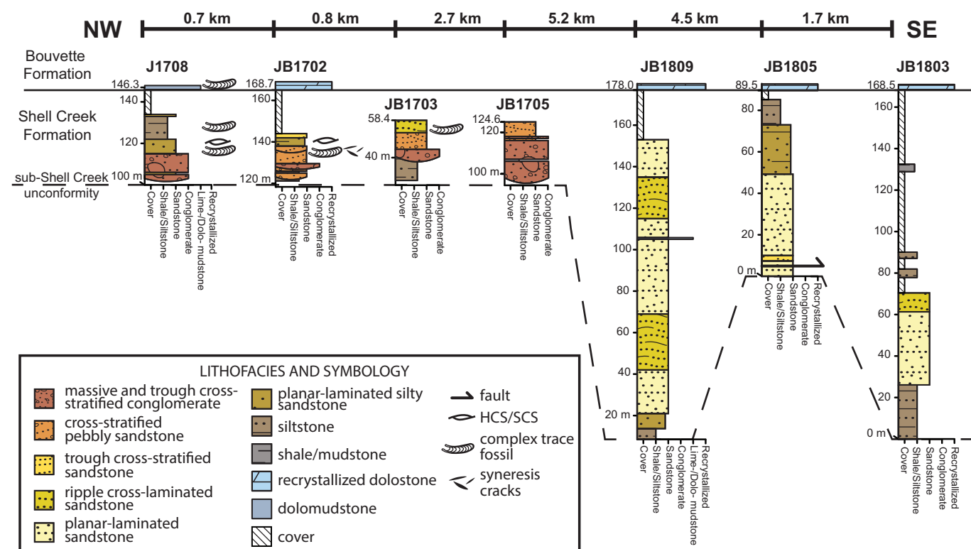
Fig. 9. Stratigraphic fence diagram of the Bouvette and Shell Creek formations above the sub-Shell Creek unconformity. The Shell Creek Formation increases in thickness by roughly a factor of three from ca. 40 m in the northwestern part of the study area to ca. 165 m in the southeastern part of the study area. This change in thickness is accompanied by a shift in lithofacies from conglomerate- and sandstone-dominated strata in the northwest to fine-grained sandstone- and siltstone-dominated strata in the southeast. HCS/SCS, hummocky and swaley cross-stratification. [Color online.]
