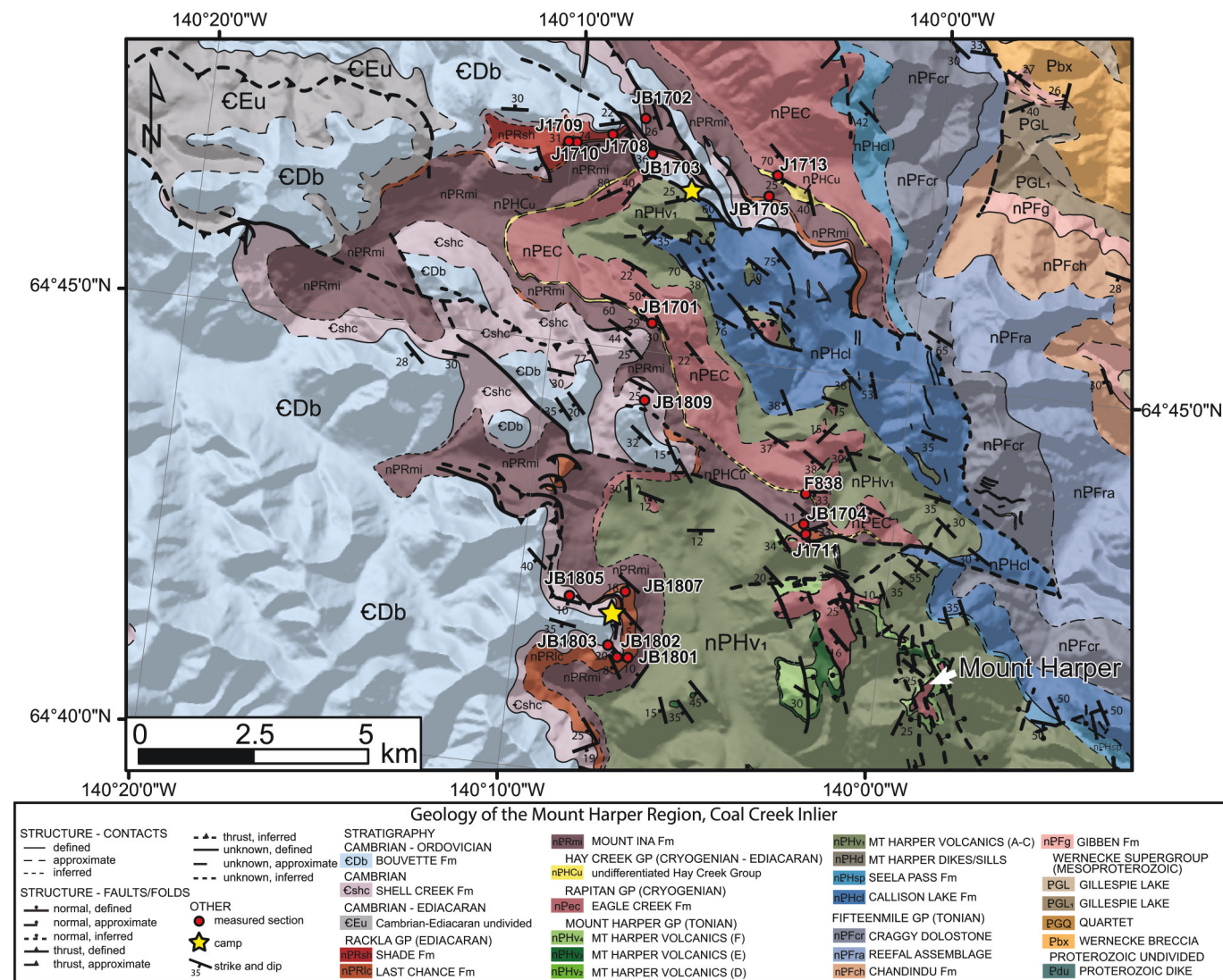
Fig. 3. Geological map of the Mount Harper Region, Coal Creek inlier, Yukon, showing measured stratigraphic sections and camp locations for this study. Map created using ESRI ArcGIS version 10.7.1 and is modified from Strauss et al. (2014). Shaded relief elevation data courtesy of Natural Resources Canada. [Color online.]
