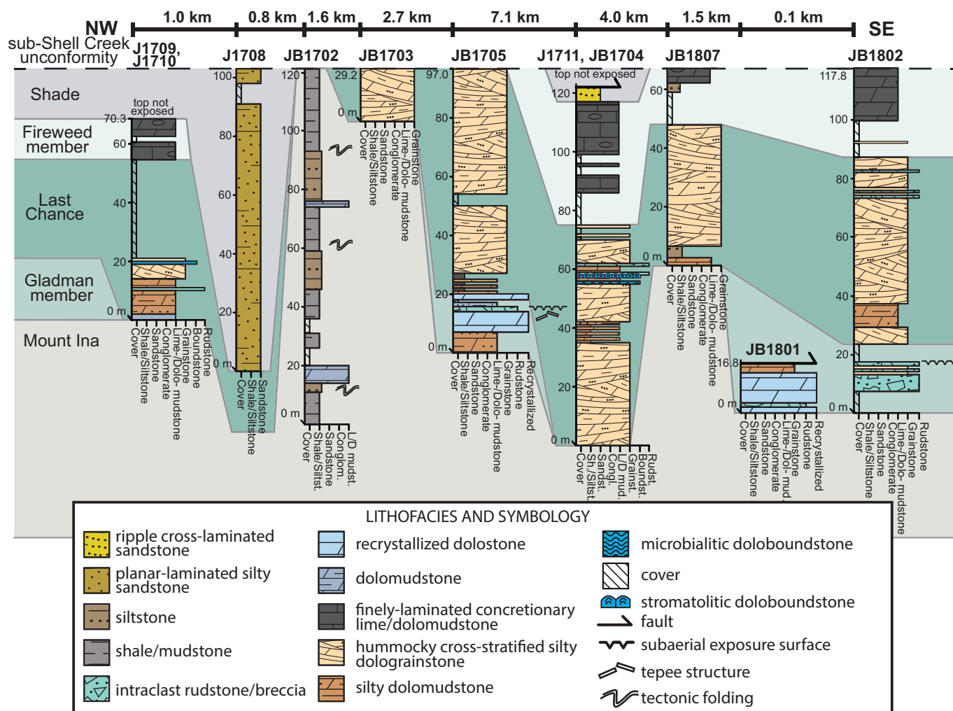
Fig. 7. Stratigraphic fence diagram of the Shade, Last Chance, and Mount Ina formations beneath the sub-Shell Creek unconformity. At least ca. 190 m of strata is truncated by the sub-Shell Creek unconformity at section JB1702, while preservation of the majority of the Ediacaran succession occurs at section JB1802. Broadly, the sub-Shell Creek unconformity incises more strata to the northwest compared with the southeast in the study area. [Color online.]
