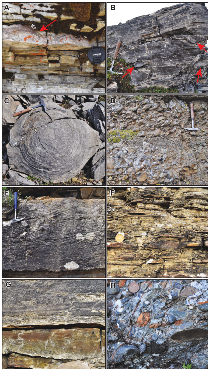
Fig. 8. (A) Hummocky cross-stratified silty dolograinstone interbedded with a single bed of stromatolitic doloboundstone (red arrow) in the upper Last Chance Formation (camera lens cap is 6 cm in diameter). (B) Finely laminated dolomudstone with lozenge-shaped concretions (red arrows) in the Fireweed member of the Last Chance Formation; hammer is 33 cm long. (C) Plan view of a large carbonate concretion within the Fireweed member; hammer is 33 cm long. (D) Crudely stratified polymict cobble conglomerate with imbricated clasts interbedded with siltstone of the Shell Creek Formation; hammer is 33 cm long. (E) Trough cross-stratified sandstone interbedded with recessive siltstone of the Shell Creek Formation; hammer is 33 cm long. (F) Planar and cross-laminated fine-grained sandstone with local starved ripples in the Shell Creek Formation; coin is 2.5 cm in diameter. (G) Planar laminated and trough cross-stratified pebble conglomerate and sandstone of the Shell Creek Formation; pencil is 13 cm long. (H) Polymict conglomerate of the Shell Creek Formation; coin is 1.8 cm in diameter. [Color online.]
