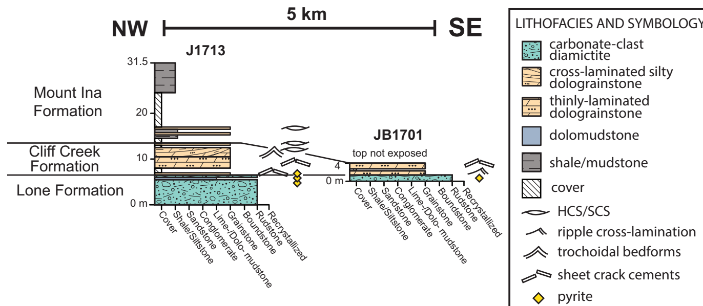
Fig. 4. Stratigraphic fence diagram of the Lone, Cliff Creek, and basal Mount Ina formations. Thin exposures of the Lone Formation were documented in both sections, while the interbedded nature of the Lone and Cliff Creek formations was only documented at the type section (J1713). In both measured sections, dolostone is eventually succeeded by black shale of the Mount Ina Formation, but this transition is only well exposed at section J1713. HCS/SCS, hummocky and swaley cross-stratification. [Color online.]
