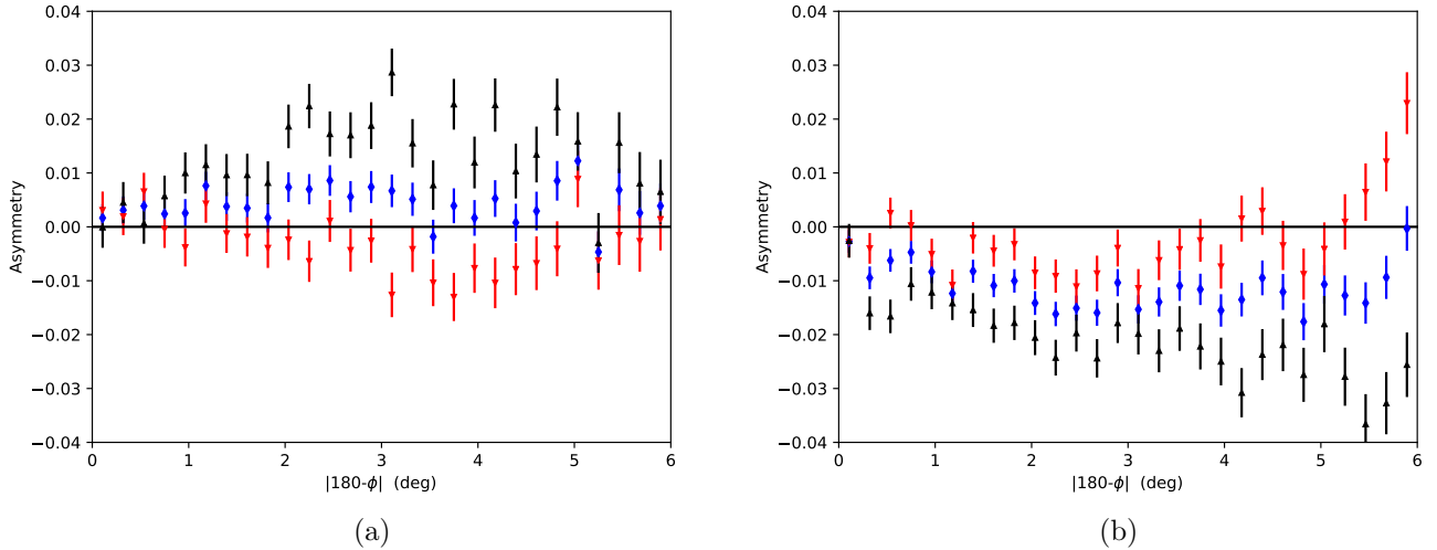
Figure 2. (a) The axial asymmetry for R \in [0.8975, 0.9600]R_0 . (b) The axial asymmetry for R \in [0.9600, 1.0225]R_0 . The blue diamonds are the aggregate axial asymmetry and the black and red triangles are for the northern ( z > 0 ) and southern ( z < 0 ) halves respectively. The sign flip in the aggregate asymmetry is clearly visible here, which we attribute to the bar’s OLR. In addition, the vertical structure changes just beyond the OLR, with a north-left correlation for R < R_{\text{OLR}} and a north-right correlation for R > R_{\text{OLR}} .
