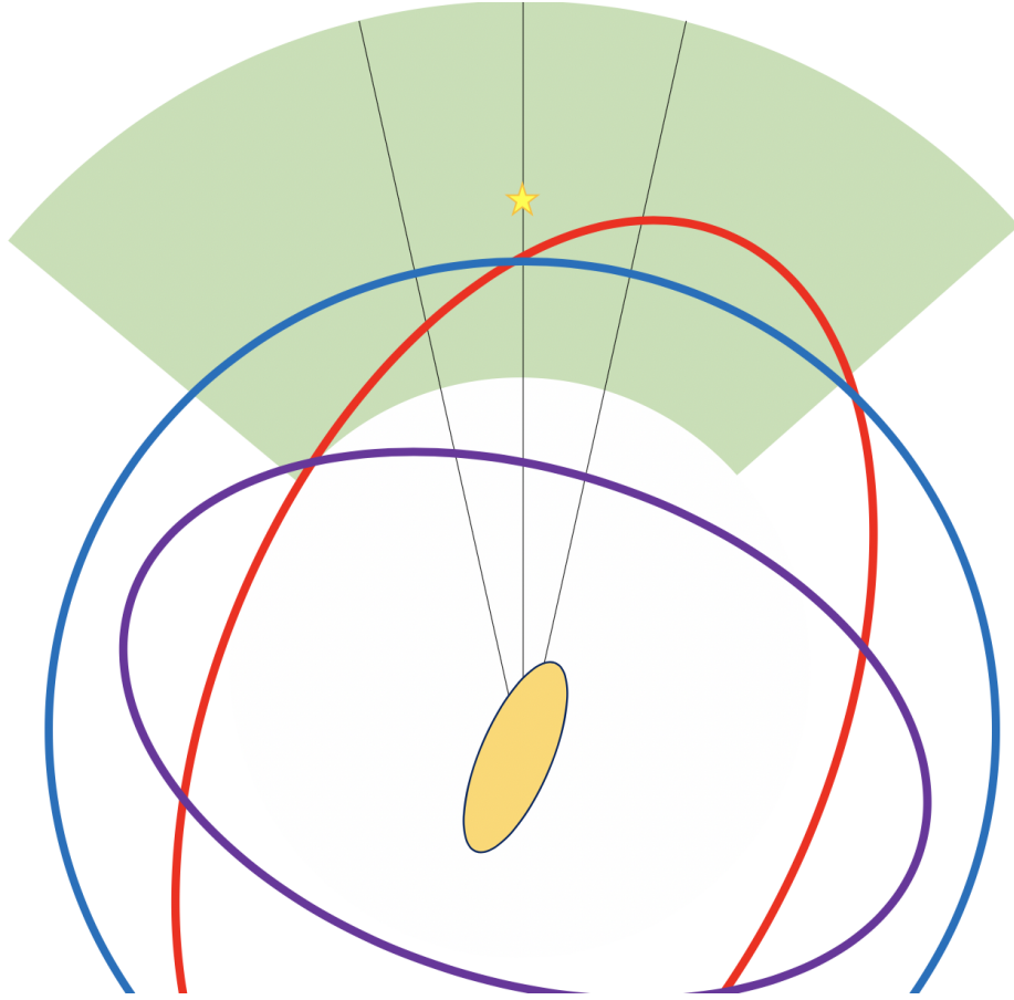
Figure 1. A schematic depiction of the orbital alignments due to the bar in the OLR region. The blue circle is the orbital radius of the OLR, the purple ellipse is an orbit interior to the OLR, and the red ellipse is an orbit exterior to the OLR. The green annular wedge region is our sample’s in-plane footprint, with a star signifying the sun’s position, and the yellow ellipse is the Galactic bar. Stellar orbits tend to align parallel (perpendicular) to the bar when the orbit is just outside (inside) the Outer Lindblad resonant radius. The geometry has been greatly exaggerated and we have shown closed orbits only, in order to illustrate the small effect we have found
