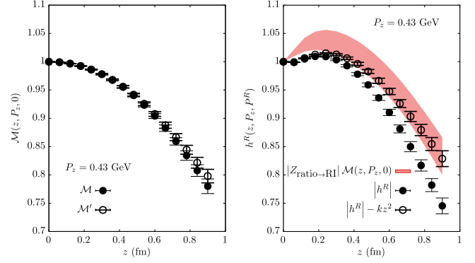
FIG. 14. The effect of higher-twist term kz^2 on the pion matrix element at fixed small P_z = 0.43 \text{ GeV} is discussed. The left panel compares the usual ratio, \mathcal{M}(z, P_z, P_z^0 = 0) , and the ratio \mathcal{M}' derived from RI-MOM matrix element after the subtraction of kz^2 [see Eq. (33)]. The right panel compares the actual RI-MOM matrix element and the RI-MOM matrix element with kz^2 subtraction with the result expected by applying the conversion factor Z_{\text{ratio} \rightarrow \text{RI}} to the ratio \mathcal{M} [see Eq. (34)].
