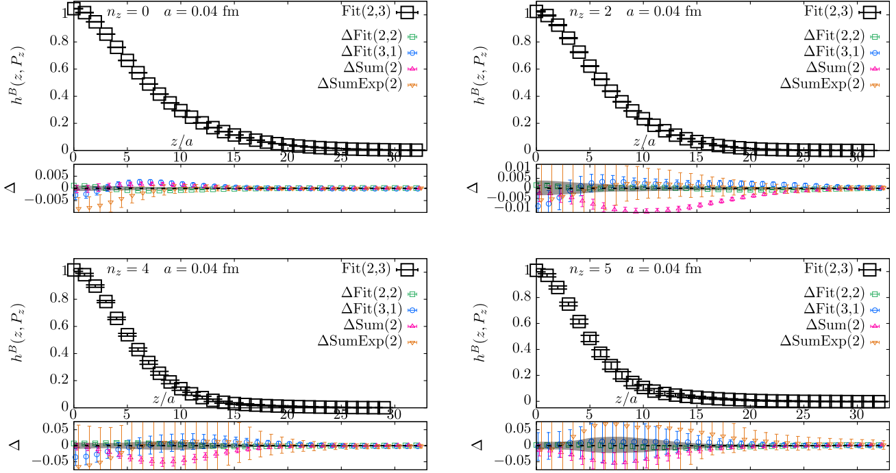
FIG. 8. The bare matrix elements h^B(z, P_z) from excited state extrapolations are shown as a function of z/a for the a = 0.04 fm ensemble. The results from n_z = 0, 2, 4 and 5 are shown in the top-left, top-right, bottom-left, and bottom-right are shown. The top part of each panel shows the z/a dependence using two-state extrapolation Fit(2,3) using t_s/a = 9, 12, 15 and 18 . The bottom part of each panel shows the deviation, \Delta , of the different extrapolation methods as explained in Fig. 7. Deviations of results from Sum(2) from 2- and 3-state fit results are seen. But we find that corrected sum SumExp(2) is consistent with the fit results. This is a result of the observation in Fig. 6.
