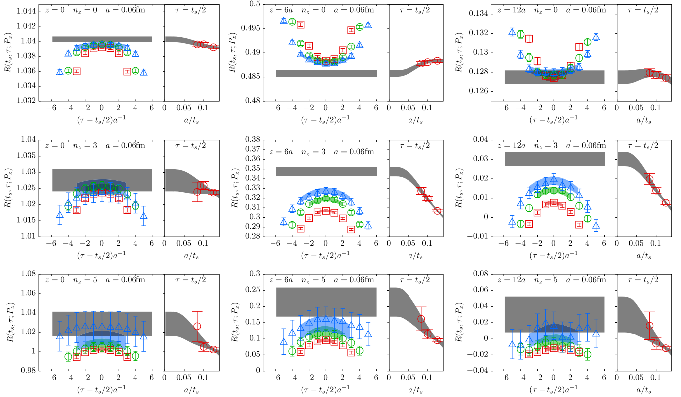
FIG. 4. The source-sink t_s and operator insertion \tau dependence of the ratio R(t_s, \tau; z, P_z) , at fixed z and P_z = 2\pi n_z/L are shown for the lattice spacing a = 0.06 fm. The top-rows are for n_z = 0 , middle ones for n_z = 3 and bottom ones for n_z = 5 . The left panels are for z = 0 , middle panels for z = 6a and right ones for z = 12a respectively. Each plot has left and right sub-panels. In the left sub-panels, the t_s - \tau/2 dependence is shown at t_s = 8a (red squares), 10a (green circles), and 12a (blue triangles). The corresponding colored bands are the 1 - \sigma error bands from Fit(2,3) (see text). On the right subpanels, the extrapolation (grey band) to t_s \rightarrow \infty is shown as a function of a/t_s at fixed \tau = t_s/2 .
