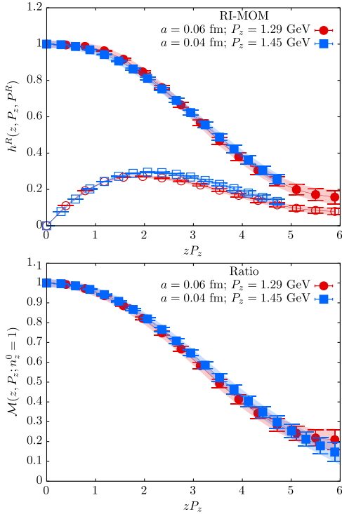
FIG. 12. Comparison of renormalized matrix elements at two lattice spacings a = 0.06 fm (red circles) and 0.04 fm (blue squares) plotted as a function of \nu = zP_z . The top panel uses RI-MOM renormalization scheme. The real and imaginary parts of the renormalized RI-MOM matrix element are shown as closed and open symbols. The bottom panel uses ratio scheme with n_z^0 = 1 . The variation of data by \pm 2\% is shown as the red and blue bands.
