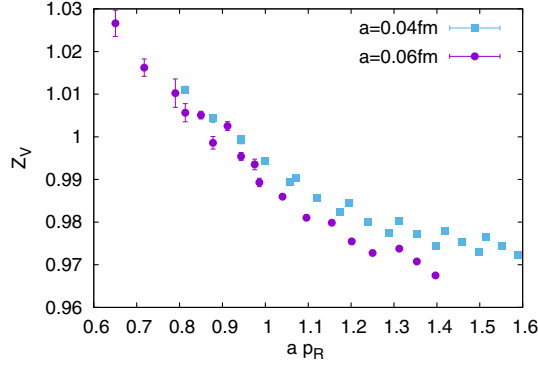
FIG. 30. The vector current renormalization factor Z_V as function of p_R in lattice units.
