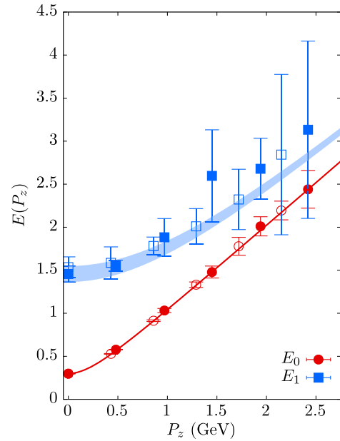
FIG. 3. The energy of the ground state ( E_0 ) and the first excited state ( E_1 ) are shown as a function of P_z . The results from a = 0.04 fm are shown as filled symbols and those from a = 0.06 fm as the open symbols. The results shown in the plot for E_0 were obtained from an unconstrained two-state fit, while E_1 were obtained by fixing E_0 to its dispersion values.
