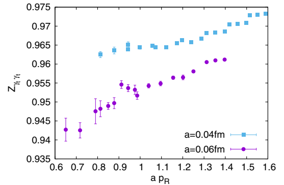
FIG. 32. The renormalization factor Z_{\gamma_i\gamma_i} as function of p_R in lattice units.
