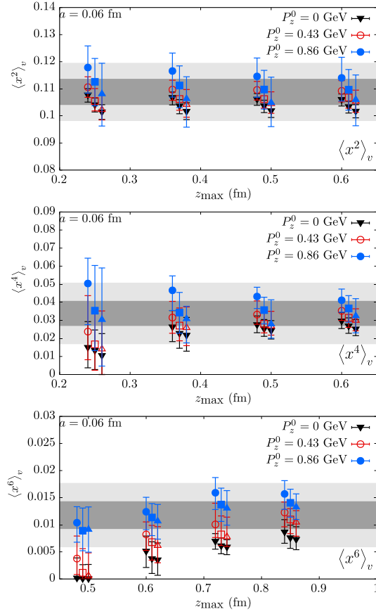
FIG. 36. Plot shows the first three even moments obtained on a = 0.06 fm lattice in a model independent manner as described in Sec. VII. The description of the three plots is similar to that in Fig. 17, Fig. 18, and Fig. 19. In addition to the two values of P_z^0 \neq 0 , this plot includes P_z^0 = 0 reference scale for the ratio.
