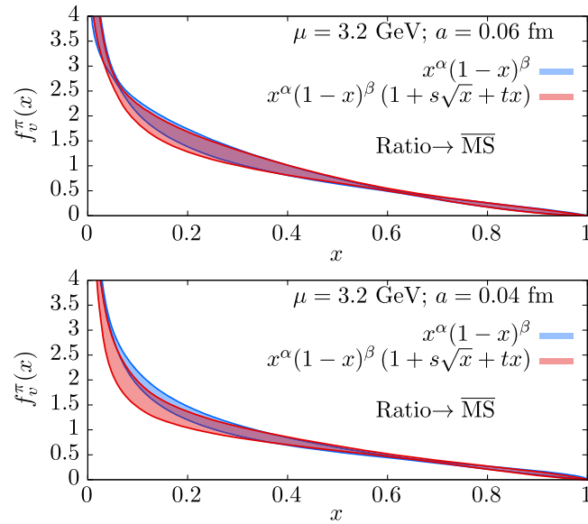
FIG. 24. Comparison of PDF as extracted using a simple two-parameter x^\alpha(1-x)^\beta ansatz and from a four-parameter x^\alpha(1-x)^\beta(1+s\sqrt{x}+tx) ansatz.
