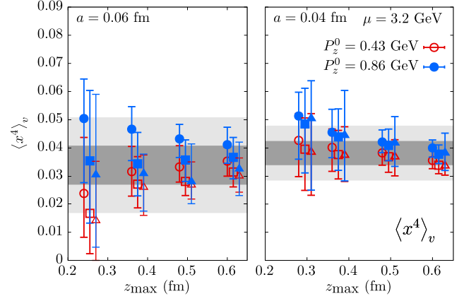
FIG. 18. \langle x^4 \rangle from combined fits of the rational polynomial function in zP_z to \mathcal{M}(z, zP_z, P_z^0) for the data z \in [z_{\min}, z_{\max}] . The description of the points are the same in Fig. 17.
