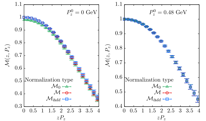
FIG. 11. Quantifying the residual systematic effects after significant statistical error reduction by the process of normalizing z = 0 matrix element to 1 [see Eq. (17) and Eq. (19)]. The plot compares the different normalization types, \mathcal{M} and \mathcal{M}_{\text{add}} , and the matrix element without any imposed normalization \mathcal{M}_0 . In the above plot, we show results for the a = 0.04 fm ensemble.
