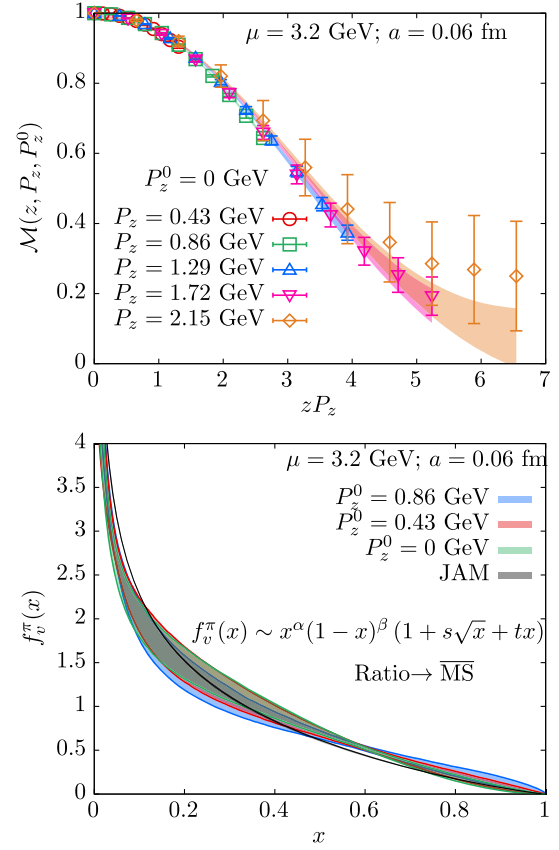
FIG. 37. The plot is on the 4-parameter PDF ansatz fits to the P_z^0 = 0 ratio data on a = 0.06 fm lattice. The top panel shows the ratio data a function of P_z z along with the fits. The bottom panel shows the PDF extracted from P_z^0 = 0 ratio with other ratio data at nonzero P_z^0 discussed in the main text. The description of the plots are similar to the ones in Fig. 21 and Fig. 22.
