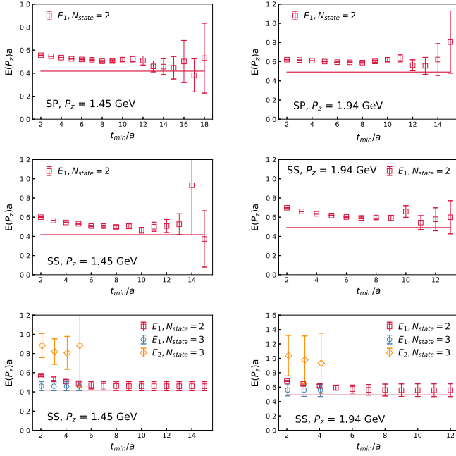
FIG. 2. The dependence of the fitted values of energy levels on the fit range [t_{\min}, 32a] is shown. The top-left and top-right panels show this dependence for the first excited level E_1 as obtained from two-state fits to SP correlator at P_z = 1.45 GeV and P_z = 1.94 GeV respectively. Similar results using SS correlator are shown in the two middle panels. The results for E_1 and E_2 obtained using three-state fits to the SS correlator (with prior on E_0 and E_1 ) are shown in the two bottom panels.
