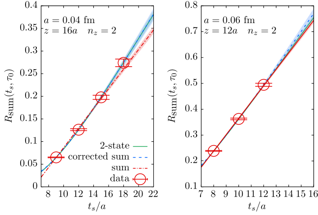
FIG. 6. An example for summation method, \text{Sum}(\tau_0) , that uses only insertion points \tau > \tau_0 = 2a are shown as a function of t_s/a at fixed z and P_z . The left panel is at a = 0.04 fm with z = 16a and n_z = 2 . The right panel is at a = 0.06 fm with z = 12a and n_z = 2 . In each panel, the red circles are the lattice data. In addition, there are three different curves—the red one is the straight line summation fit to the data, the blue one is the corrected summation fit \text{SumExp} that includes \exp[-(E_1 - E_0)t_s] correction, and the green one is the expected summation curve from the two-state fit \text{Fit}(2,3) .
