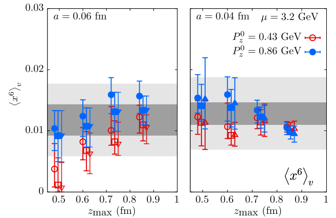
FIG. 19. \langle x^6 \rangle from combined fits of the rational polynomial function in zP_z to \mathcal{M}(z, zP_z, P_z^0) for the data z \in [z_{\min}, z_{\max}] using priors \langle x^2 \rangle_v and \langle x^4 \rangle_v . The dependence of \langle x^6 \rangle on z_{\max} is shown. At each z_{\max} , values from z_{\min} = a, 2a and 3a are shown.
