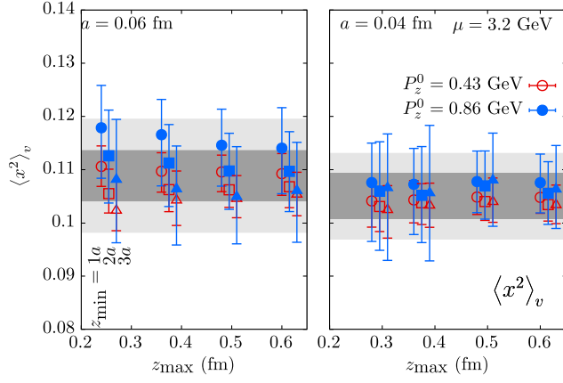
FIG. 17. \langle x^2 \rangle from combined fits of the rational polynomial function in zP_z to \mathcal{M}(z, zP_z, P_z^0) for the data z \in [z_{\min}, z_{\max}] . The dependence of \langle x^2 \rangle on z_{\max} is shown. For each z_{\max} , values from three different z_{\min} are shown. The results for a = 0.06 fm and 0.04 fm are shown in the left and right panels. The grey bands are the estimates—the inner band includes only statistical error, and outer one includes both statistical and systematic error (see text).
