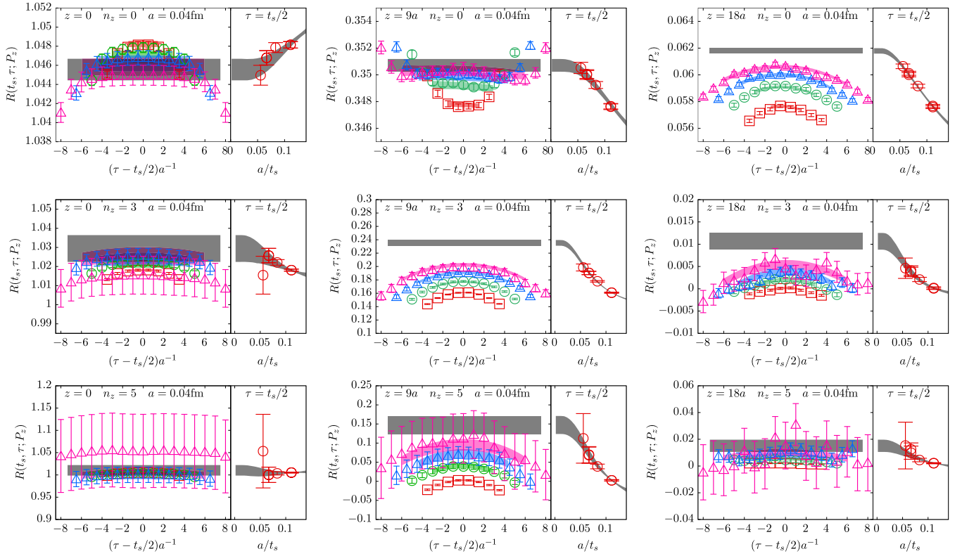
FIG. 5. The source-sink t_s and operator insertion \tau dependence of the ratio R(t_s, \tau; z, P_z) , at fixed z and P_z = 2\pi n_z/L are shown for the lattice spacing a = 0.04 fm. The top-rows are for n_z = 0 , middle ones for n_z = 3 and bottom ones for n_z = 5 . The left panels are for z = 0 , middle panels for z = 9a and right ones for z = 18a respectively. Each plot has left and right sub-panels. In the left sub-panels, the t_s - \tau/2 dependence is shown at t_s = 9a (red squares), 12a (green circles), 15a (blue triangles) and 18a (pink inverted-triangles). The corresponding colored bands are the 1 - \sigma error bands from Fit(2,3) (see text). On the right sub-panels, the extrapolation (grey band) to t_s \rightarrow \infty is shown as a function of a/t_s at fixed \tau = t_s/2 .
