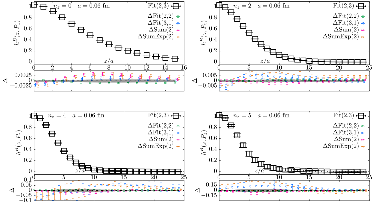
FIG. 7. The bare matrix elements h^B(z, P_z) from excited state extrapolations are shown as a function of z/a for the a = 0.06 fm ensemble. The results from n_z = 0, 2, 4 and 5 are shown in the top-left, top-right, bottom-left, and bottom-right are shown. The top part of each panel shows the z/a dependence using two-state extrapolation \text{Fit}(2,3) using t_s/a = 8, 10 and 12 . The bottom part of each panel shows the deviation, \Delta , of the different extrapolation methods \text{Fit}(2,2) , \text{Fit}(3,1) , \text{Sum}(2) , \text{SumExp}(3) from the method \text{Fit}(2,3) . The scatter of these differences from 0 (shown by dashed line) characterizes the robustness of the extrapolation.
