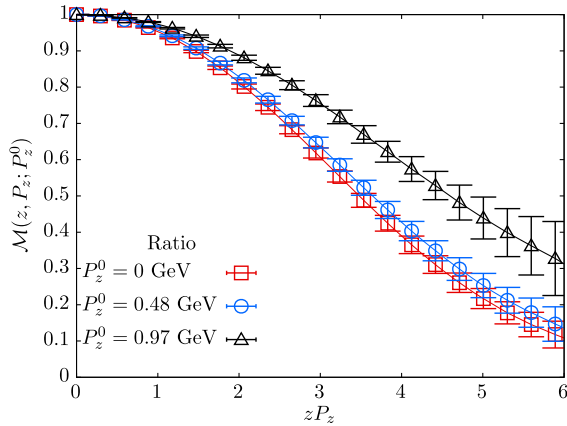
FIG. 10. Comparison of renormalized matrix elements at fixed P_z = 1.45 GeV in the ratio scheme with generalized nonzero values of the reference momentum P_z^0 . The different colored symbols correspond to different P_z^0 = 0, 0.48 and 0.97 GeV. The effect of changing P_z^0 is significant, but it does not cause a big difference in signal-to-noise ratio at smaller z that we are interested in. It is the expectation that matrix elements with P_z, P_z^0 > \{\Lambda_{\text{QCD}}, m_\pi\} suffer from lesser higher-twist contamination.
