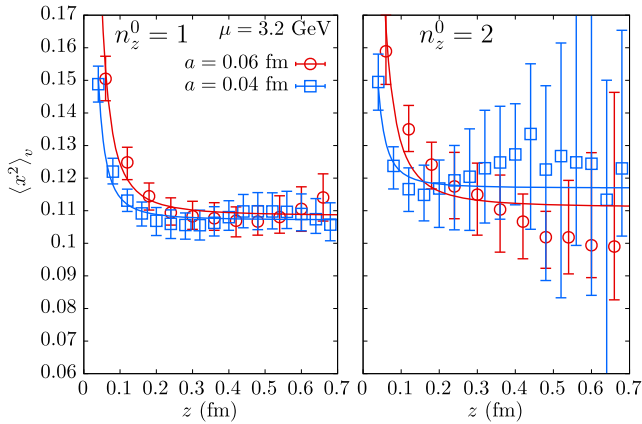
FIG. 16. The z dependence of \langle x^2 \rangle obtained by fitting rational polynomial functions in zP_z to matrix elements \mathcal{M}(z, P_z, P_z^0) at different fixed values of z , with P_z^0 = 2\pi n_z^0/L . The left panel shows results as obtained with n_z^0 = 1 and the right panel for n_z^0 = 2 . In each case, the red and blue points correspond to a = 0.06 fm and 0.04 fm lattice spacings. The curves are fits to a functional form \langle x^2 \rangle + 2r(z/a)^{-2} to capture possible (aP_z)^2 corrections (refer text).
