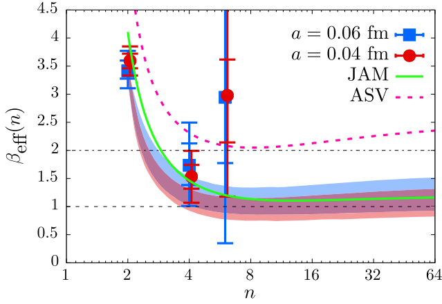
FIG. 27. The plot shows the effective large- x exponent \beta_{\text{eff}}(n) as a function of n . The data points are obtained by using values of moments \langle x^n \rangle_v obtained from the model independent combined fits. The smaller error bar is only the statistical error and larger error bar is statistical plus systematic error. The red and blue points are the results using our a = 0.06 fm and 0.04 fm respectively. The red and blue bands are the expectation for the behavior of \beta_{\text{eff}}(n) as obtained from the model-dependent fits to the pion matrix elements. The green curve is the expectation using the JAM data [79] and the purple dashed curve is obtained using the ASV analysis [35].
