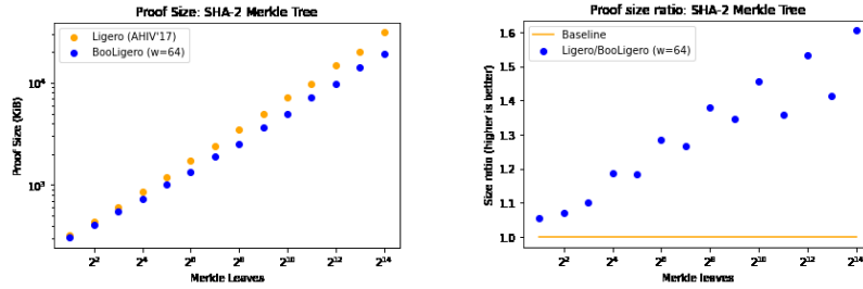
Fig. 6: BooLigerio and Ligerio absolute and relative proof sizes for SHA-2 Merkle trees
