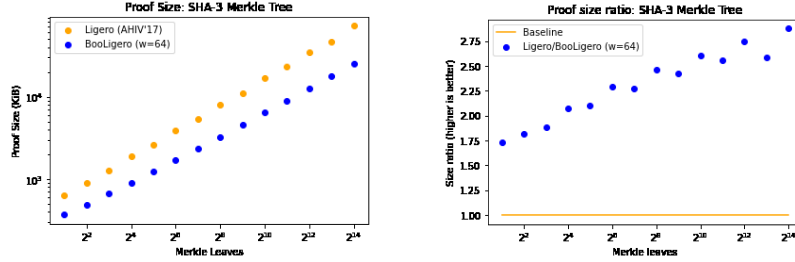
Fig. 5: BooLigero and Ligero absolute and relative proof sizes for SHA-3 Merkle trees
