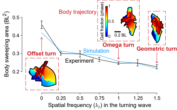
Fig. 5: The area swept by the body for the turning gaits with varied turning wave spatial frequency k_t . The results are normalized by the robot body length squared ( BL^2 ). Error bars indicate the standard deviation. The time evolution of robot's configurations executing the designed gaits over a period are shown in the red dashed boxes, where the gait fraction is indicated by colors from the beginning (blue) to the end (red). The geometric turn has the lowest swept area due to the fact that its net rotation is also low. The omega turn has the smallest swept area per degree angular displacement achieved over the cycle.
