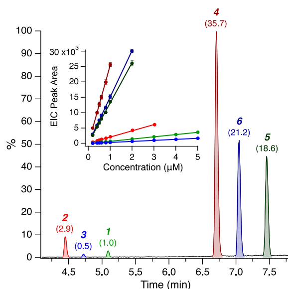
Figure 2. UPLC/(-)ESI-Q-TOF-MS BPI chromatogram of an equimolar (1.00 \mu\text{M} ) aqueous solution of carboxylic acids 1–3 and dimer esters 4–6. (–)ESI efficiencies, normalized to that of cis -pinonic acid (1), are given in parentheses. (Inset) Weighted ( 1/X ), linear ( R^2 > 0.998 ) calibration curves, generated from triplicate measurements ( 1\sigma ) of equimolar aqueous solutions of carboxylic acids 1–3 and dimer esters 4–6 spanning a concentration range from 0.200 to 5.00 \mu\text{M} .
