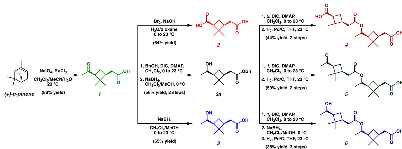
Scheme 1. Synthesis of Carboxylic Acids 1–3 and Dimer Esters 4–6 from Commercially Available (+)- \alpha -Pinene a
