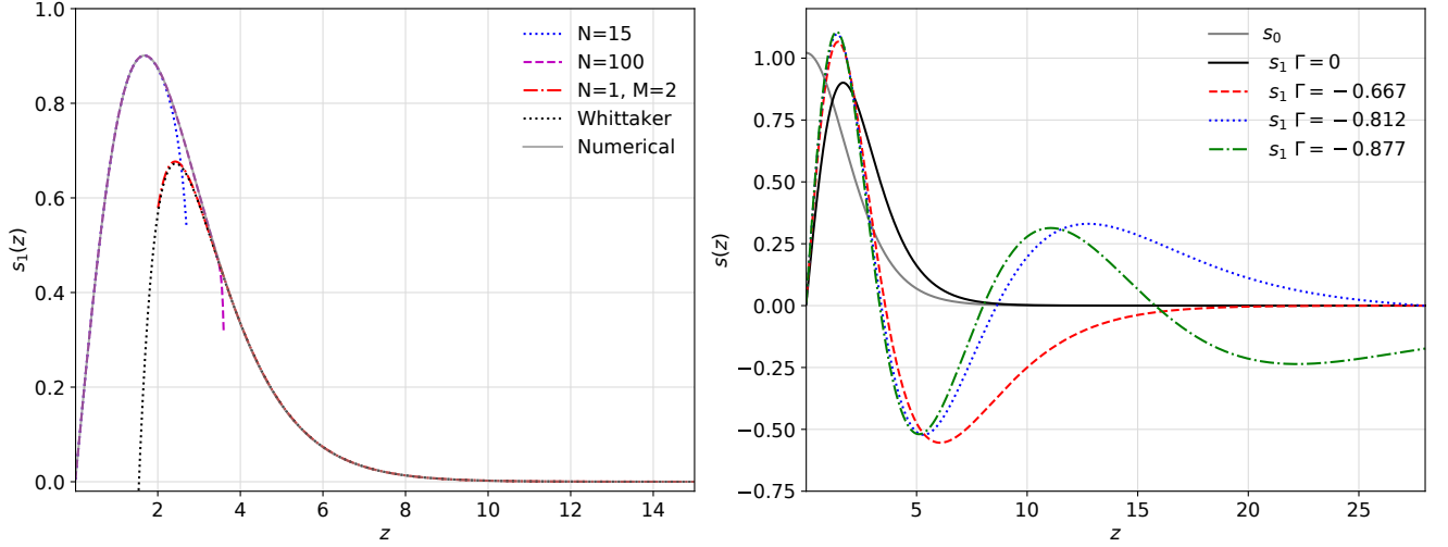
FIG. 1. One-state solution. Left: The numerical solution (solid gray) and truncated series expansion at small radius (dotted blue and dashed magenta) and large radii (dot-dashed red) as well as the analytic Whittaker approximation (dotted black) for the wavefunction of a rotating perturbation with \ell = 1 and \Gamma = 0 . Right: Numerical solution for the wavefunction of a rotating perturbation with \ell = 1 and \Gamma = 0 (black), \Gamma = -0.667 (dashed red), \Gamma = -0.812 (dotted blue) and \Gamma = -0.877 (dot-dashed green). The non-rotating ground state wavefunction is shown for comparisons (gray solid).
