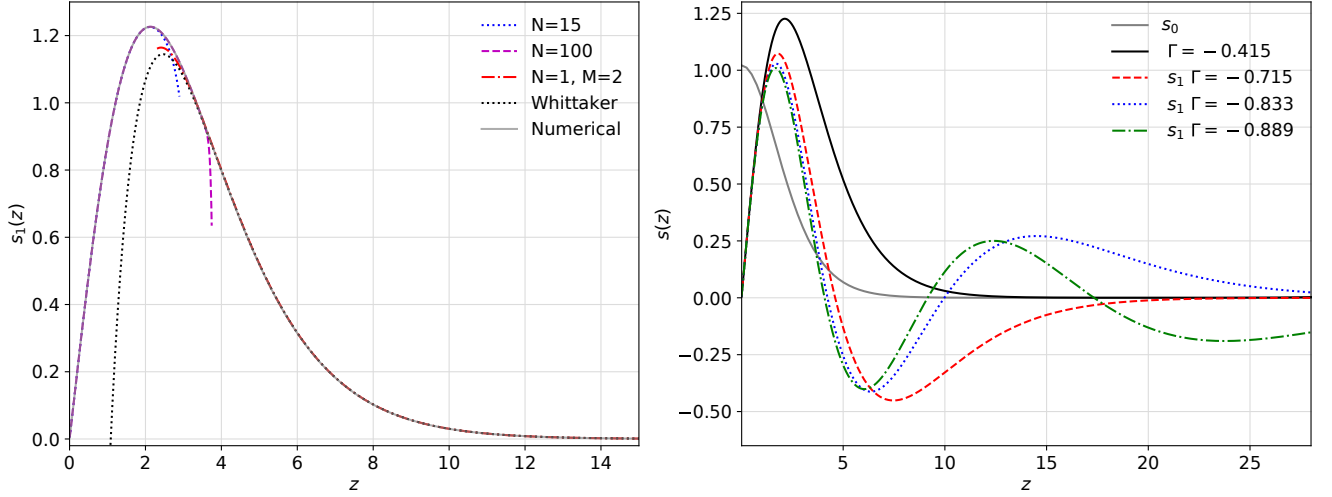
FIG. 2. Two-state solution. Left: The numerical solution (solid gray) and truncated series expansion of at small radius (dotted blue and dashed magenta) and large radii (dot-dashed red) as well as analytic Whittaker approximation (dotted black) for the wavefunction of a rotating perturbation with \ell = 1 and \Gamma = -0.415 in the two-state ansatz. Right: Numerical solution for the wavefunction of a rotating perturbation with \ell = 1 and \Gamma = -0.415 (black), \Gamma = -0.715 (dashed red), \Gamma = -0.833 (dotted blue) and \Gamma = -0.889 (dot-dashed green). The non-rotating ground state wavefunction is shown for comparisons (gray solid).
