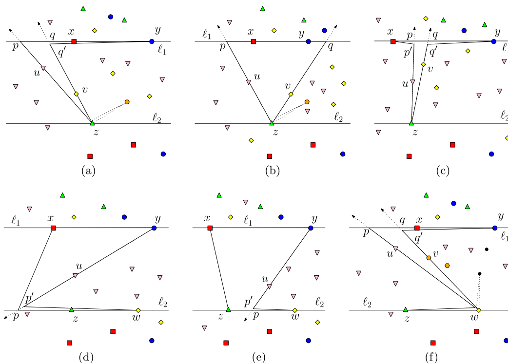
Fig. 8. Illustrating the proof of Proposition 10.
