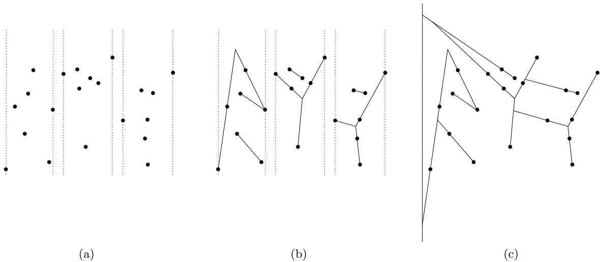
Fig. 10. Part (a): Dividing the n points into groups of size 7. Part (b): Applying Lemma 12 to each group. Part (c): Joining all trees to a vertical segment.
