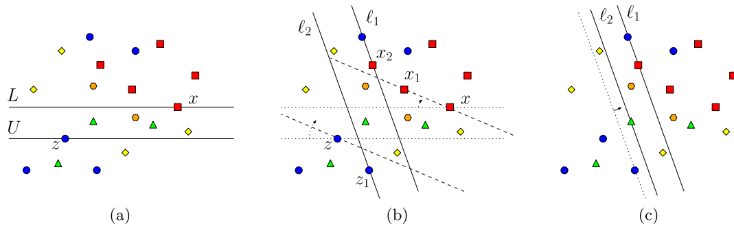
Fig. 3. Illustrating the proof of Lemma 6. The points of S_1 and S_3 are drawn as red squares and blue circles, respectively.
