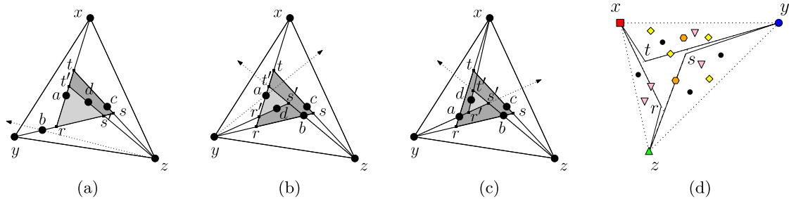
Fig. 6. (a)–(c) Building a new expedient triangle \Delta r's't' from the expedient triangle \Delta rst , when replacing c by d . (d) A perfect rainbow hexagon for six of the colors. (For interpretation of the references to colour in this figure legend, the reader is referred to the web version of this article.)
