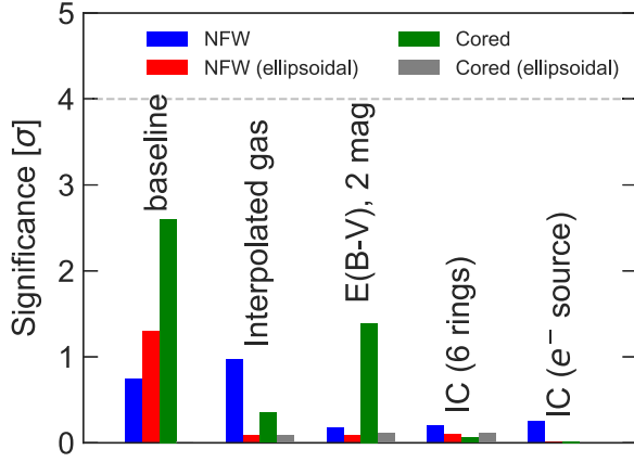
FIG. 4. Summary of the detection significance (in sigma units) for each of the DM templates considered in this work (see Fig. 3 and Table I). The baseline background model (Table II) includes the hydrodynamic gas maps and 3D IC maps (four rings). For the alternative backgrounds models, we switched to the dust residual maps with different interstellar extinction E(B-V) magnitude cut (2 magnitude) 3D IC maps (divided in six rings), and 2D IC map containing a central source of e^- [39], except in the case of the traditional interpolated gas maps which were paired with the IC maps broken in six rings. When evaluating the significance of the DM templates, the nuclear bulge and boxy bulge maps were included in the fits. The horizontal gray line shows the usual 4\sigma detection threshold.
