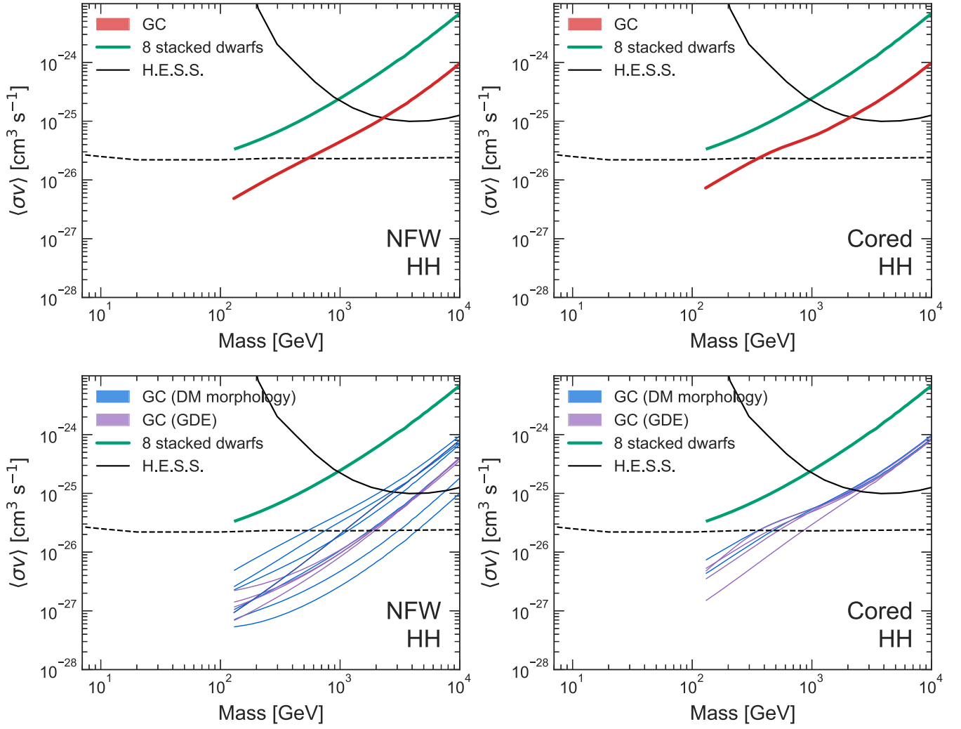
FIG. 16. The least constraining upper limits for annihilation through Higgs boson among all of the considered variations around NFW- \gamma (top left) and around the cored profile (top right). The bottom panels show the upper limits for each individual variation of the DM morphology and GDE around the NFW profile (bottom left) and the cored profile (bottom right).
