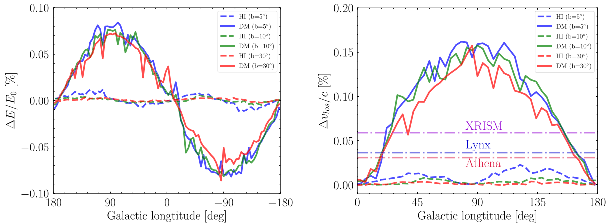
FIG. 2. Left panel: The relative line shift \Delta E/E_0 versus Galactic longitude l at Galactic latitude b = 5^\circ, 10^\circ , and 30^\circ . Solid lines denote DM shift while dashed lines are for HI gas shift. Direct comparison between these two cases shows that at l \sim 90^\circ the Doppler shift from DM can be clearly distinguished from the astrophysical one. Right panel: the separation of two emission lines as given in Eq. (4) observed around l = 0^\circ at fixed b = 5^\circ, 10^\circ , and 30^\circ . The horizontal dash-dotted lines show the expected energy resolution ( 1\sigma , not FWHM) of future x-ray telescopes at 3.5 keV. Though the separation, \Delta v_{\text{los}}/c , is within a factor of \sim 2 of the nominal energy resolution, we estimate that the centroids of the DM versus gas lines may be separated at > 5\sigma with XRISM exposures of 3.9 to 15 Ms, Athena exposures of 10 to 52 ks, and Lynx exposures of 23 to 110 ks, whether a very aggressive or a much more conservative estimate of the expected background is considered; see Table I.
