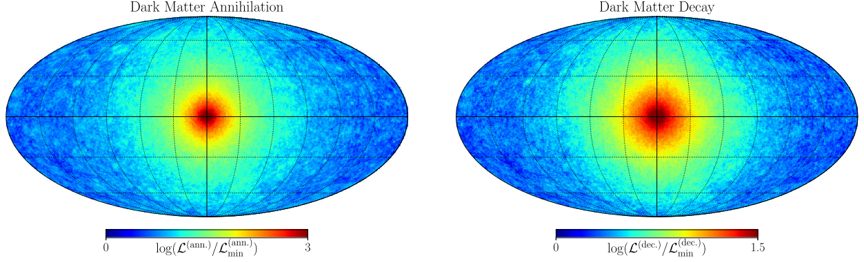
FIG. 4. Left panel: The Galactic DM annihilation luminosity distribution from an observer at the Sun position (at R_\odot = 8.2 kpc) in the FIRE-2 m12i simulation. Right: The analogous Galactic DM luminosity map for the case of DM decay. See text for more details on the full-sky prediction of DM luminosity from FIRE-2.
