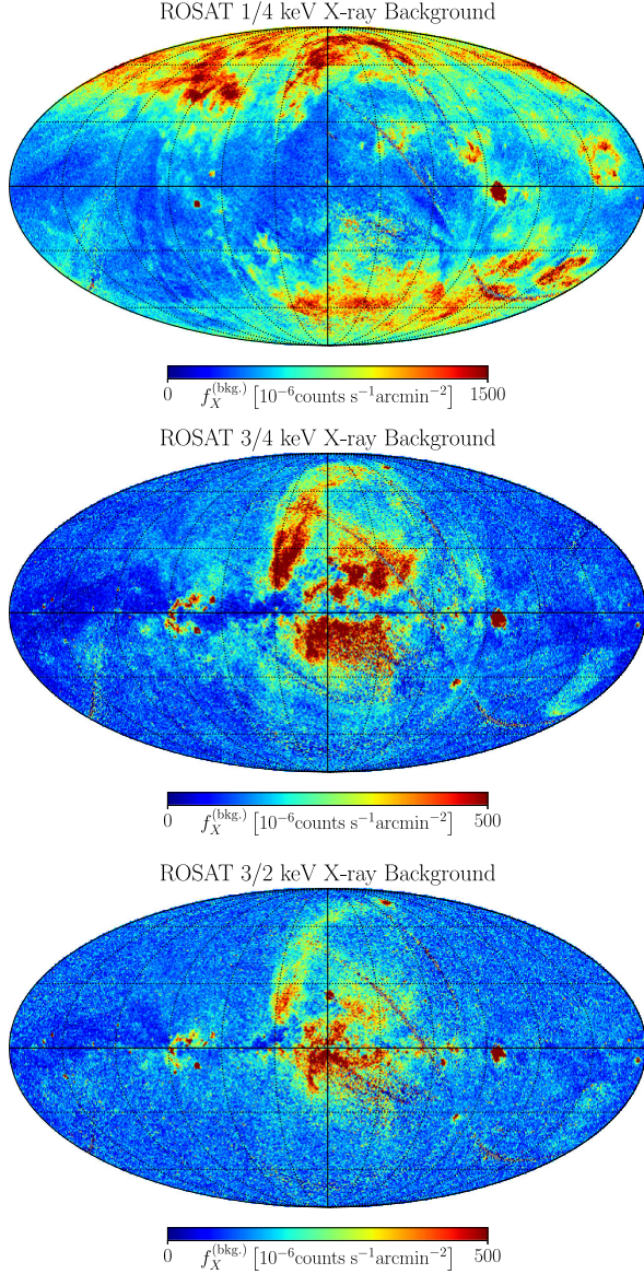
FIG. 5. The ROSAT 1/4 (upper), 3/4 (middle), and 3/2 (bottom) keV x-ray background map reproduced from Ref. [115] with same angular resolution ( \sim 0.2^\circ ) and unit of flux ( 10^{-6} \text{ counts s}^{-1} \text{ arcmin}^{-2} ) as provided in the data.
