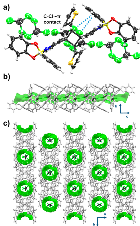
Figure 4. X-ray structure of the diboron adduct 2(\text{pbe}) \cdot (4\text{p}2\text{tcb}) \cdot \text{CHCl}_3 : (a) ORTEP view and \text{C} \cdots \text{Cl} \cdots \pi contacts with \text{CHCl}_3 solvate molecules; (b) channel occupied by chloroform; (c) adjacent channels in the ab plane.
