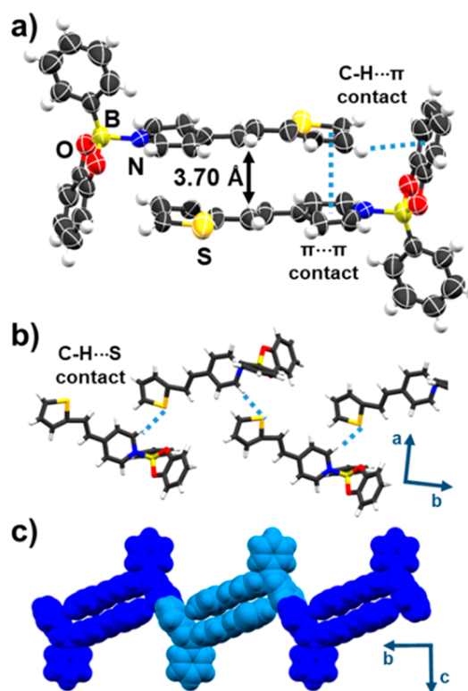
Figure 2. X-ray structure of adduct ( pbe )·( pte ): (a) ORTEP view; (b) herringbone arrangement; (c) dimeric assemblies.
