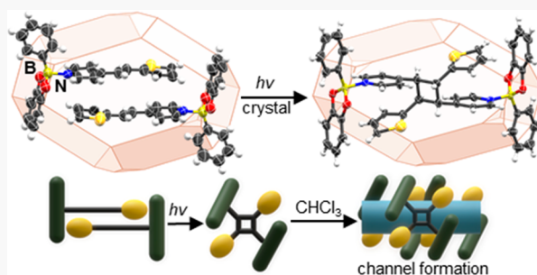
Scheme 1. (a) SCSC [2 + 2] Photodimerization of ( pbe )·( pte ) to 2(pbe)·(4p2tcb) and (b) Change in Boron Coordination Modes from Monotopic to Ditopic and Channel Formation
