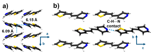
Figure 1. X-ray structure thiophene pte : (a) herringbone arrangement; (b) hydrogen-bonded layers.
