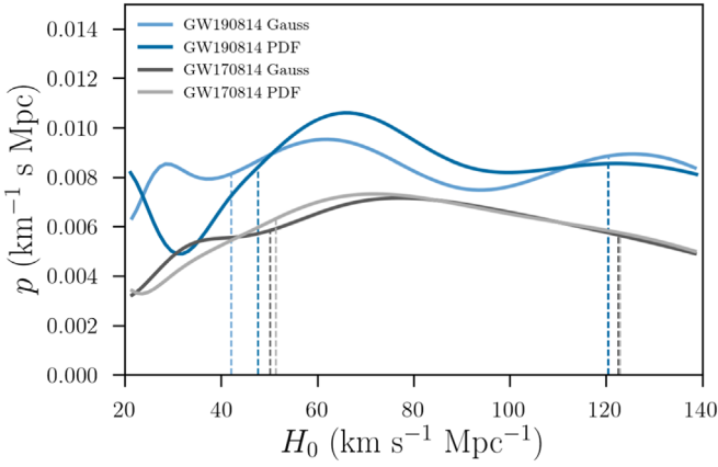
Figure 2. Hubble constant posterior distributions for GW190814 (blue curves) and GW170814 (gray curves), comparing results using the Gaussian redshift PDF versus the full PDFs. The latter case does not depend on the choice of redshift cut, as long as this contains the range of z supported by the H_0 prior. The 68% HDI of all PDFs is shown by the dashed lines. Posteriors have been rescaled for visualization purposes. The sky map used here for GW190814 is the LALInference map released in 2019 August.
