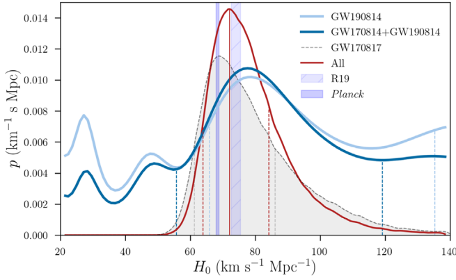
Figure 3. Hubble constant posterior distribution for GW190814 obtained by marginalizing over \sim 1800 possible host galaxies from DES (light blue line). The dark blue curve represents the posterior obtained by the combination of GW190814 and GW170814 using DES galaxies. The maximum a posteriori and its 68% CI for the combined result is H_0 = 78^{+57}_{-13} km s ^{-1} Mpc ^{-1} using a flat prior in the range [20,140] km s ^{-1} Mpc ^{-1} . The posterior obtained by Nicolaou et al. (2020) for the bright standard siren event GW170817, associated to one galaxy, is shown in gray. A combination of the two dark sirens considered in this work with GW170817 is shown in red and gives H_0 = 72.0^{+12}_{-8.2} km s ^{-1} Mpc ^{-1} . The addition of the dark sirens provides a \sim 18\% improvement to the 68% CI from GW170817 alone. The maximum a posteriori is represented by the solid vertical line. Posteriors have been rescaled for visualization purposes. The 68% CI of all PDFs is shown by the dashed lines. The GW190814 sky map used for this plot is the latest map released by the LVC in 2020 July. Constraints from Planck (Planck Collaboration et al. 2018) and Riess et al. (2019) (R19) at 1\sigma are shown in purple boxes.
