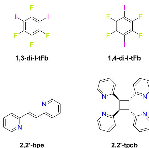
Scheme 1. Components for cocrystals.
