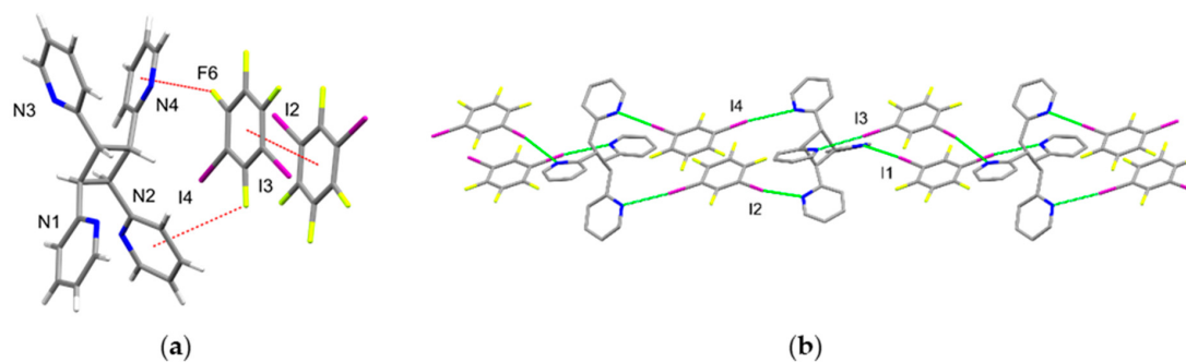
Figure 2. Perspectives of 2(1,3-di-I-tFb)·(2,2'-tpcb): (a) asymmetric unit highlighting \pi \cdots \pi and \pi \cdots F forces (cyclobutane disorder omitted for clarity) and (b) 1D chains (H atoms omitted for clarity).
