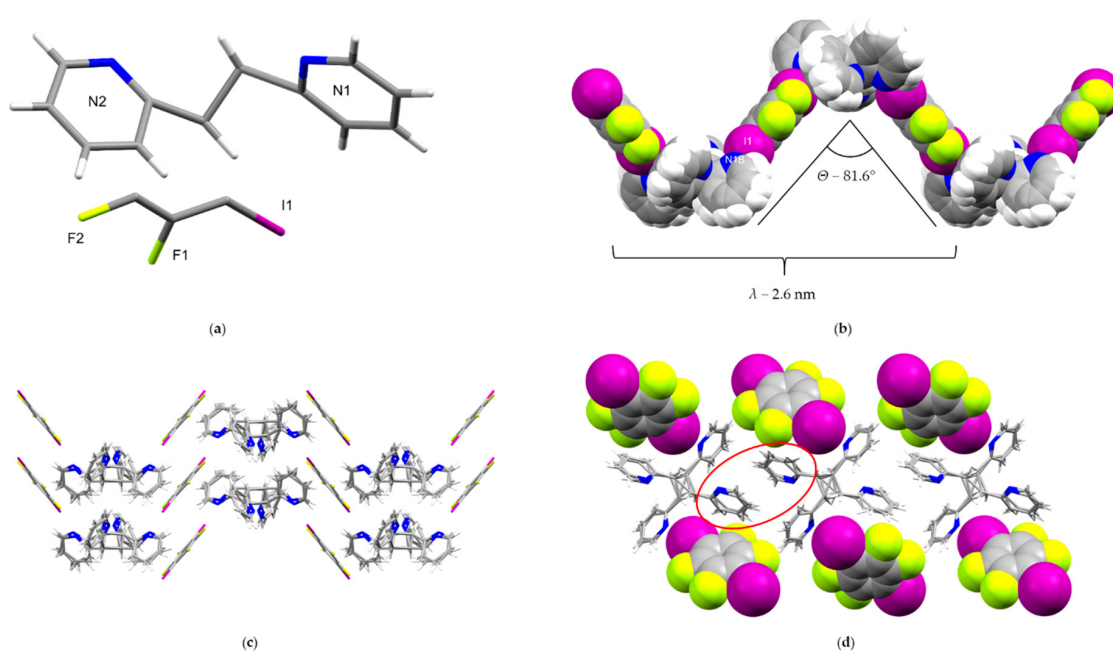
Figure 4. Perspectives of (1,4-di-I-tFb):(2,2'-tpcb): (a) asymmetric unit (cyclobutane disorder omitted for clarity); (b) infinite zig-zag chains (space-filling, view along c); (c) herringbone pattern resulting from interactions between zig-zag chains; and (d) 1D chains of 2,2'-tpcb generated along the crystallographic c -axis, highlighting offset, face-to-face \pi \cdots \pi forces.
