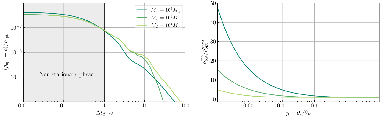
FIG. 12. On the left, we plot the relative difference between the optimal SNR of a lensed GW (solving the diffraction integral) and the matched filter SNR using a stationary phase approximation (SPA) lensed waveform as a template. We fix the GW orbital frequency ( \omega/2\pi = 257 Hz) and vary the source-lens alignment ( y \in [10^{-4}, 10] ) to get different time delays between the type I and II images \Delta t_d . We present the results for different lens masses satisfying the geometric optics approximation, t_M \cdot \omega > 1 . On the right, we compare optimal SNR computed using the SPA for the signal with the optimal SNR for the true wave optics signal as a function of y . The rest of the binary and lens parameters correspond to q = 1 , z_s = 0.5 , z_L = 0.1 , \theta = 0.3 , \phi = 0.4 , \psi = 1.5 , \iota = \pi/3 , and \chi_{\text{eff}} = \chi_p = e = 0 .
