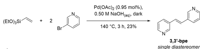
Figure 7 Synthesis of 3,3'-bpe via Pd-catalyzed Hiyama–Heck cross-coupling.
