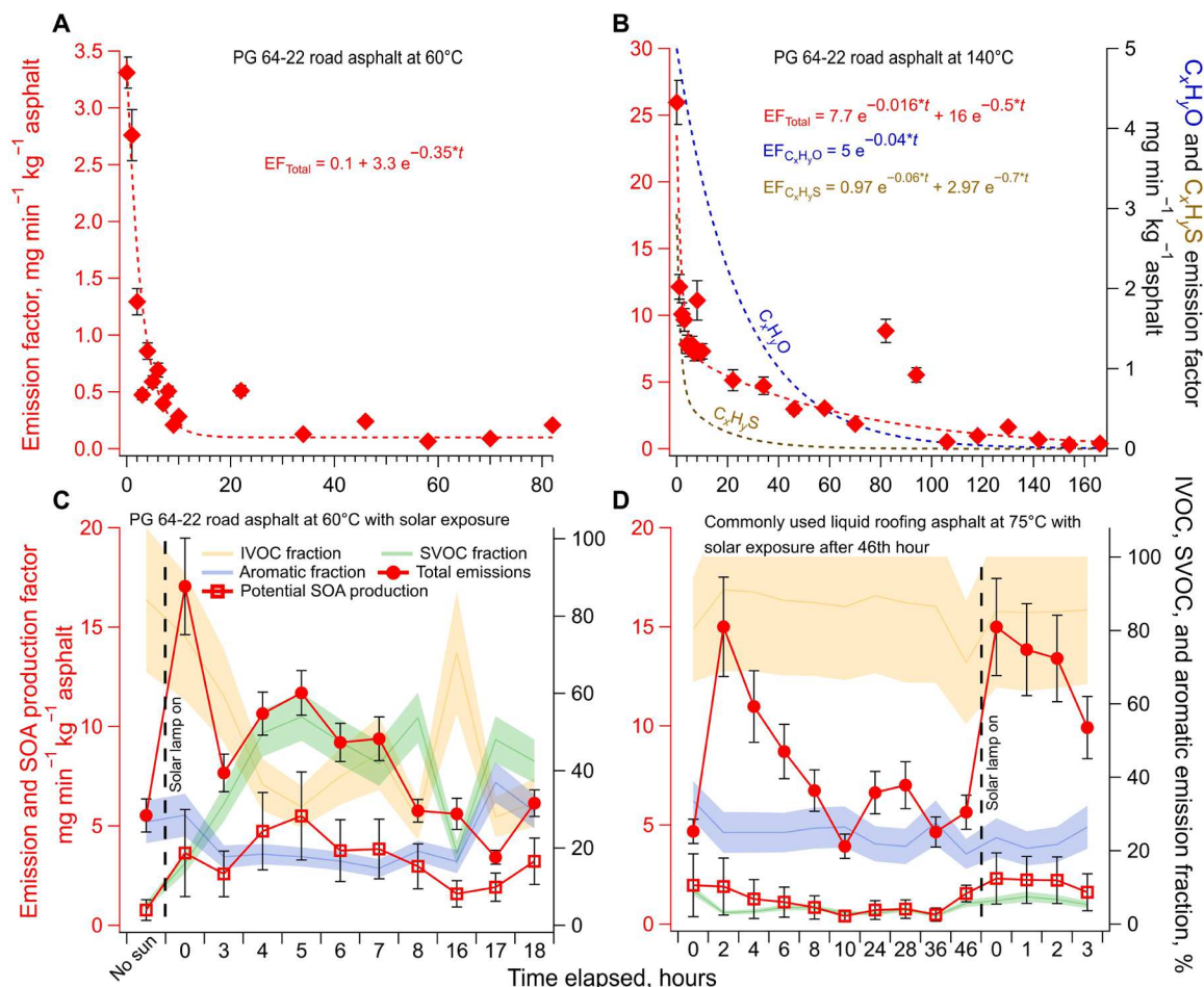
Fig. 3. Changes in temperature-related emissions over prolonged heating and large emission enhancements with solar exposure. (A and B) Variation in total gas-phase emission factors over time from commonly used PG 64-22 road asphalt as observed in laboratory experiments simulating (A) in-use temperatures (60°C) and (B) paving temperatures (140°C). Individual markers for the C_xH_yS and C_xH_yO fitted decay curves in (B) are shown in fig. S7, including for 60°C where heteroatom-containing emissions were minor and did not exhibit a clear decaying trend. Additional details including SDs on equations in (A) and (B) can also be found in fig. S7. (C and D) Emission enhancements due to solar exposure shown with total gas-phase emission factors (solid circles) and SOA production factors (hollow squares) over time for (C) PG 64-22 road asphalt under solar exposure at 60°C and (D) commonly used liquid roofing asphalt under solar exposure at 75°C. The orange, green, and blue curves in both panels show the IVOC, SVOC, and aromatic fractions of the total emissions, respectively, and are shown as a function of discrete time points on the x axes. The error bars and error bands indicate SD in emission factors and SOA production factors, respectively. Emissions from liquid roofing asphalt exclude any potential contributions from Stoddard solvent off-gassing.
