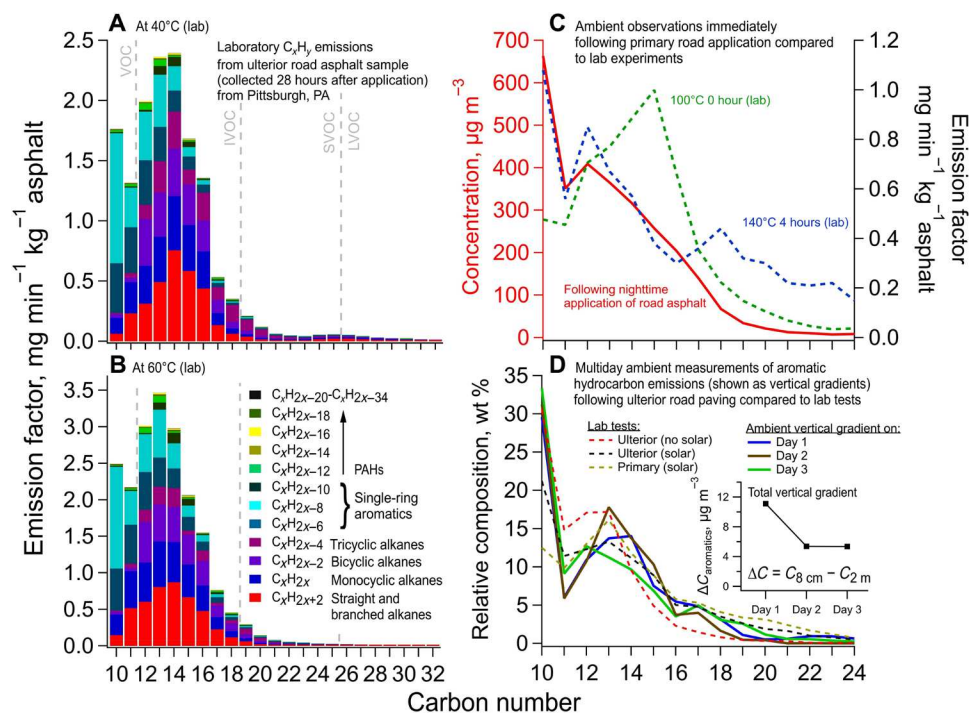
Fig. 5. Consistent results from other asphalt samples and ambient measurements. (A and B) Chemical speciation of complex gas-phase hydrocarbon emissions from ultrior (i.e., minor) road asphalt collected from Pittsburgh, PA, during laboratory tests at (A) 40°C and (B) 60°C. In both cases, hydrocarbons made up over 95% of the total emissions. (C and D) Confirmatory ambient measurements following road asphalt application demonstrate similar emissions (shown as a function of carbon number) for (C) primary roadway asphalt immediately following application in New Haven, CT (detailed composition in fig. S9) and (D) over 3 days of measurements at an ultrior roadway in Pittsburgh, PA, both compared to laboratory experiments. To evaluate continued vertical fluxes (i.e., emissions) over 3 days, the main plot in (D) shows the aromatic vertical concentration differentials at 8 cm versus 2 m (i.e., Conc. at 8 cm – Conc. at 2 m) via simultaneous adsorbent tube collection at the 2 heights. Single-ring aromatics and PAHs are shown here to remove biogenic interferences, but supporting vertical gradient data via GC-TOF and GC-EI-MS for alkanes, aromatics, and PAHs can be found in figs. S9 and S10. The inset in (D) shows the sum of vertical concentration differential for aromatic compounds. The field results from the 3 days show good agreement with laboratory data, including SVOC enhancements with solar exposure.
