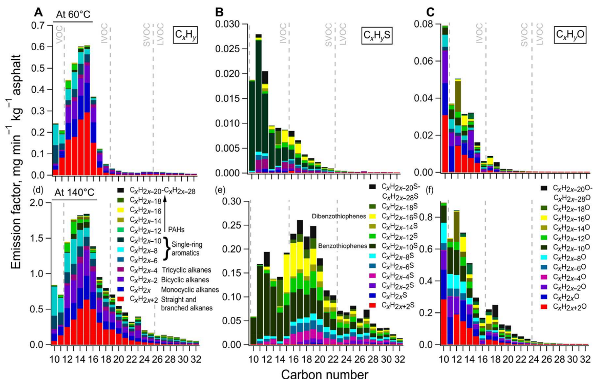
Fig. 2. Detailed chemical composition of hydrocarbons and functionalized organic compound emissions. Laboratory test results of the chemical composition of gas-phase complex mixture emissions from PG 64-22 road asphalt at typical in-use ( 60^\circ\text{C} ) and paving ( 140^\circ\text{C} ) temperatures. The emission factors and volatility distributions are shown in (A) and (D) for the hydrocarbon ( \text{C}_x\text{H}_y ) emissions, (B) and (E) for sulfur-containing compound ( \text{C}_x\text{H}_y\text{S} ) emissions, and (C) and (F) for oxygen-containing compound ( \text{C}_x\text{H}_y\text{O} ) emissions. The legend indicates distribution of molecular structures within each carbon number bin ranging from n -alkanes to PAHs. The trace signals on PAHs with formulas \text{C}_x\text{H}_{2x-20} to \text{C}_x\text{H}_{2x-28} (and corresponding heteroatom-containing formulas) are lumped together and labeled in black.
