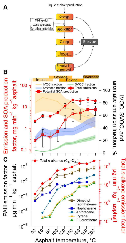
Fig. 1. Asphalt's life cycle and temperature-dependent emissions. (A) Different stages in asphalt's life cycle with potential to emit reactive organic gases into the atmosphere. (B) Temperature dependence of total gas-phase emissions from asphalt, ranging from in-use (40° to 60°C) and storage (80° to 140°C) to paving and overheating (120° to 200°C) temperature conditions (filled circles). The corresponding potential SOA that could be produced is also shown (hollow squares). The orange, green, and blue curves show the IVOC, SVOC, and aromatic fractions of the total emissions, respectively. The error bars indicate SD of the emission and SOA production factors, and the error bands indicate the SD in the volatility fractions. (C) Variation in the emission factors of select hazardous PAHs and total n -alkanes ( C_{10} – C_{32} ) with applied temperature.
