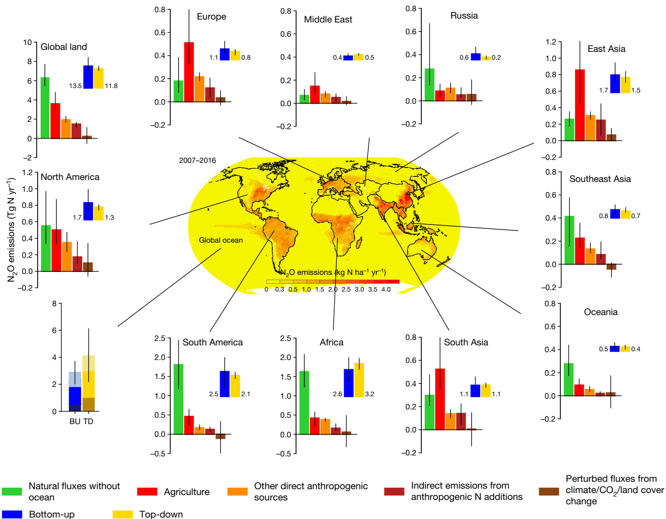
Fig. 2 | Regional \text{N}_2\text{O} sources in the decade 2007–2016. The Earth's ice-free land is partitioned into ten regions: North America, South America, Europe, Middle East, Africa, Russia, East Asia, South Asia, Southeast Asia and Oceania. Each subplot shows the emissions from five sub-sectors using bottom-up approaches, followed by the sum of these five categories using bottom-up approaches (blue) and the estimates from top-down approaches (yellow). Bottom-up and top-down estimates of ocean emissions are shown at the
