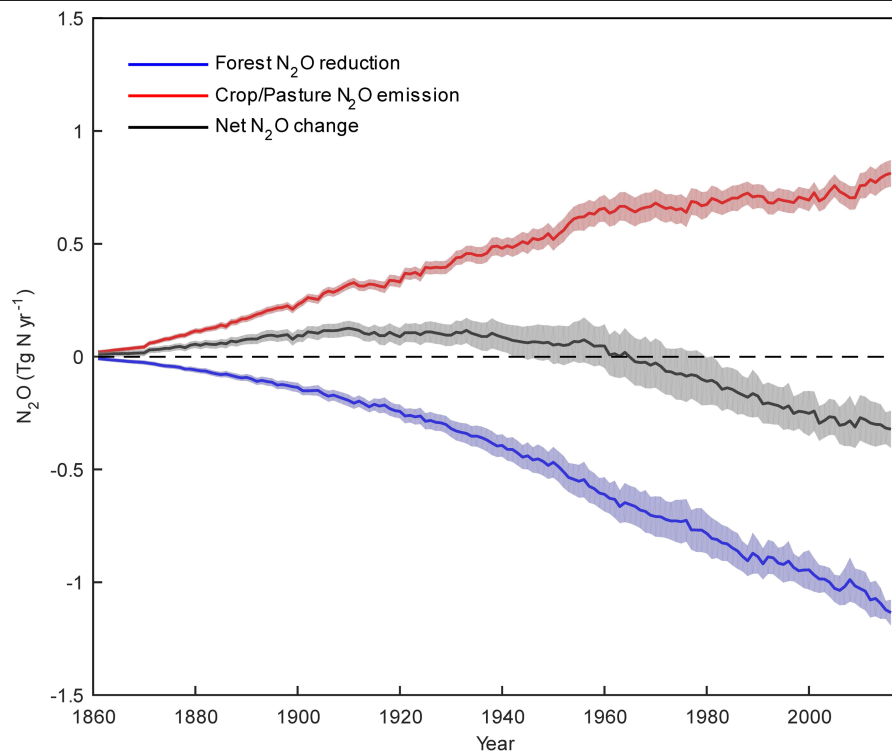
Extended Data Fig. 7 | Global \text{N}_2\text{O} dynamics due to land cover changes. The blue line represents the mean forest \text{N}_2\text{O} reduction caused by the long-term effect of reduced mature forest area (that is, deforestation) and shaded areas show minimum and maximum estimates; the red line represents the mean \text{N}_2\text{O} emission from the post-deforestation pulse effect (that is, crop/pasture \text{N}_2\text{O}
