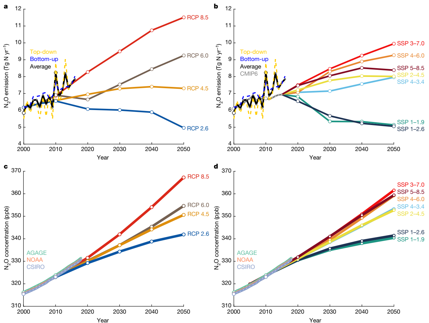
Fig. 4 | Historical and projected global anthropogenic N_2O emissions and concentrations. a–d , Global anthropogenic N_2O emissions ( a , b ) and concentrations ( c , d ) compared to the four RCPs in the IPCC assessment report 5 ( a , c ; ref. 2 ) and the new marker scenarios based on the SSPs used in CMIP6 ( b , d ; ref. 48 ). The historical emissions data are represented as the mean of the bottom-up and top-down estimates of anthropogenic N_2O emissions, whereas the historical atmospheric concentration data are from the three available
