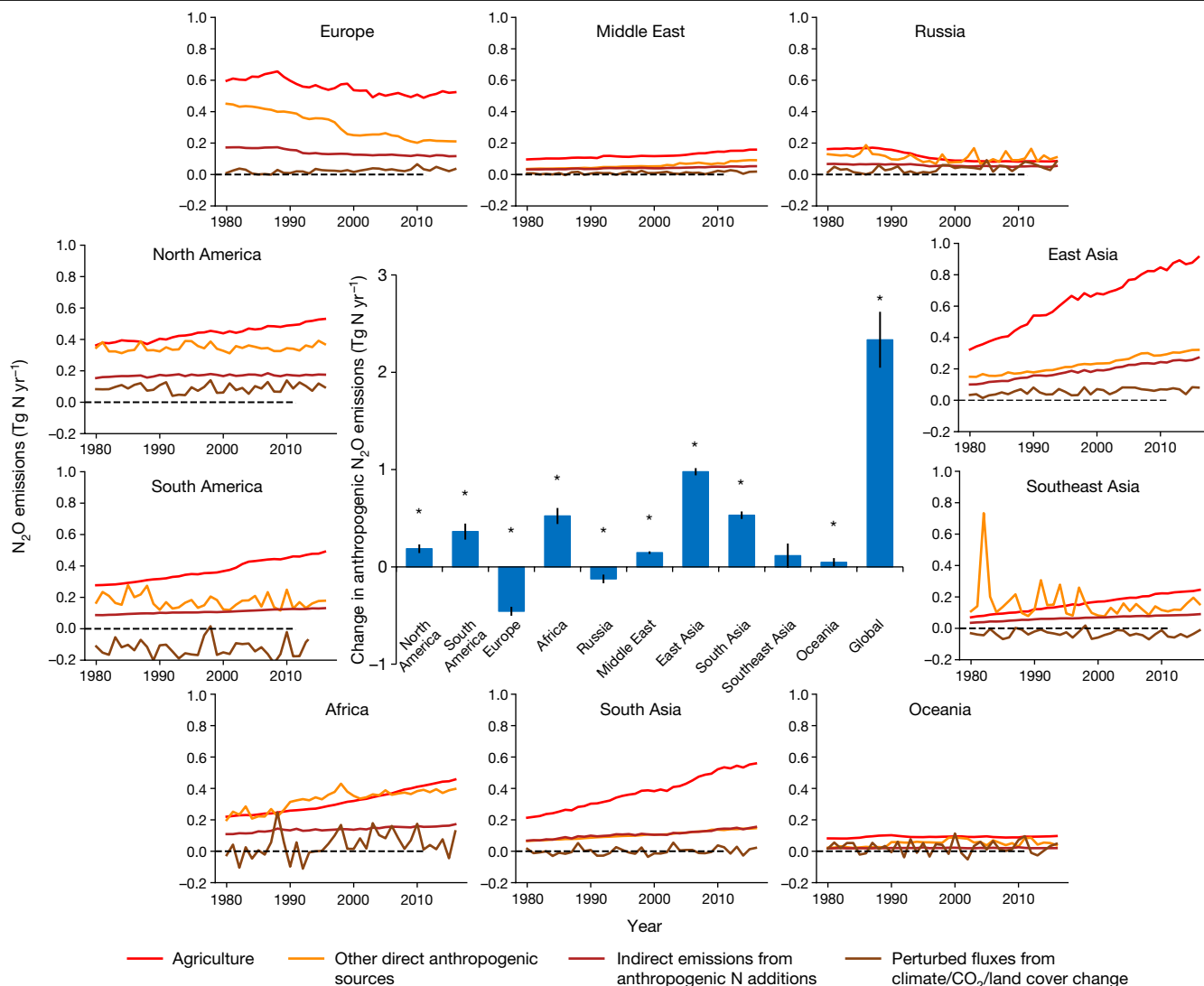
Fig. 3 | Ensembles of regional anthropogenic \text{N}_2\text{O} emissions over the period 1980–2016. The bar chart in the centre shows the accumulated changes in regional and global \text{N}_2\text{O} emissions during the study period of 1980–2016. Error bars indicate the 95% confidence interval for the average of accumulated changes. The Mann–Kendall test was performed to examine a monotonic increasing or decreasing trend in the estimated ensemble \text{N}_2\text{O} emissions
