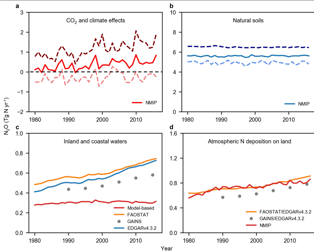
Extended Data Fig. 6 | Global N 2 O emissions from natural soils, inland and coastal waters and due to change in climate, atmospheric CO 2 and nitrogen deposition. a , Changes in global soil N 2 O fluxes due to changing CO 2 and climate. b , Global natural soil N 2 O emissions without consideration of land use change (for example, deforestation) and without consideration of indirect anthropogenic effects via global change (that is, climate, increased CO 2 and atmospheric nitrogen deposition). The estimates are based on NMIP estimates during 1980–2016 including six process-based land biosphere models. Here, we also subtracted the difference between including and not including emissions from secondary forests (that grow back after pasture or cropland abandonment) as part of natural soil emissions based on NMIP estimates. The
