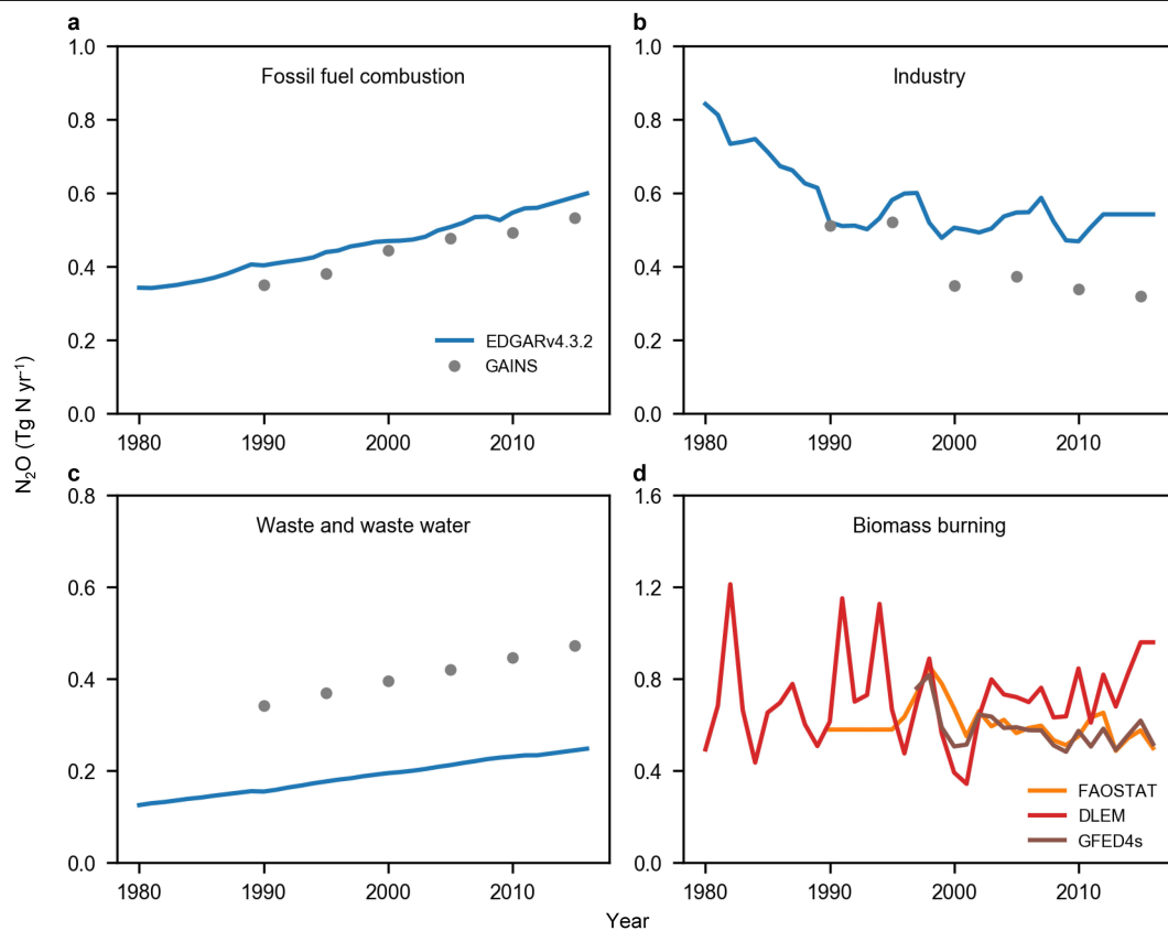
Extended Data Fig. 5 | Global \text{N}_2\text{O} emission from other direct anthropogenic sources. a , Emission from fossil fuel combustion based on EDGAR v4.3.2 and GAINS estimates. b , Emission from industry based on EDGAR
