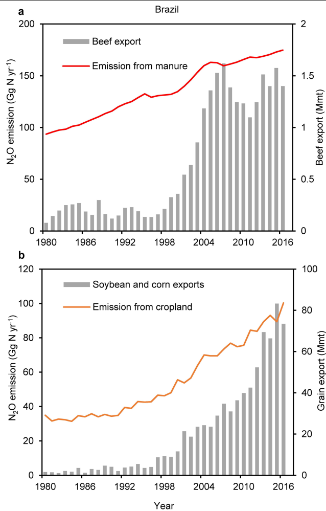
Extended Data Fig. 9 | Direct soil emissions and agricultural product trades in Brazil. a , The red line shows the ensemble direct \text{N}_2\text{O} emissions from livestock manure based on EDGAR v4.3.2, GAINS and FAOSTAT, the sum of ‘manure left on pasture’ and ‘manure management’. The grey columns show the amount of beef exported by Brazil. b , Orange line shows the ensemble direct \text{N}_2\text{O} emissions from croplands due to nitrogen fertilization based on NMIP and SRNM. The grey columns show the amount of soybeans and corn exported by Brazil. Data regarding beef and cereal product exports were adapted from the ABIEC (beef) and FAOSTAT (soybean and corn) databases. \text{Mmt yr}^{-1} represents millions of metric tons per year.
