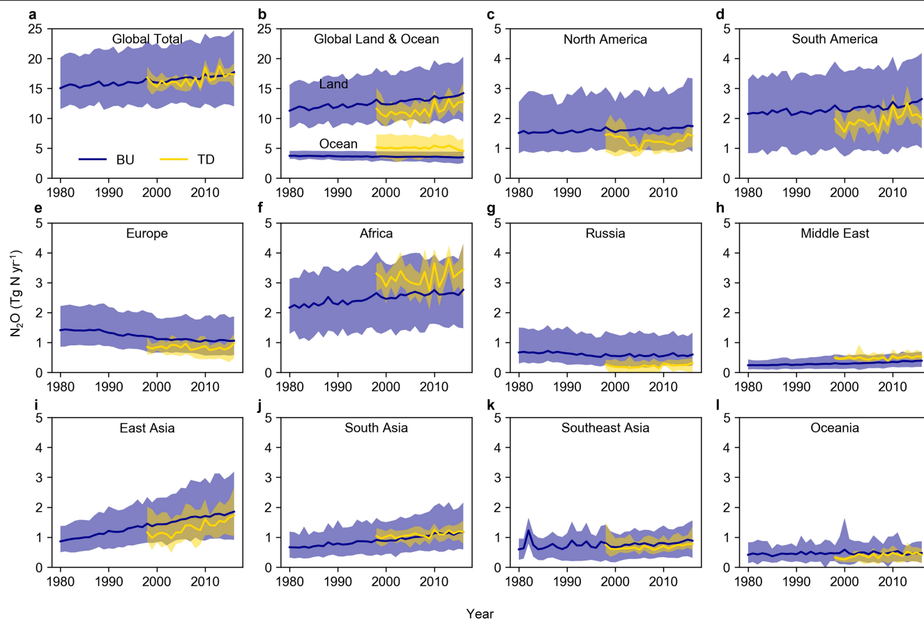
Extended Data Fig. 3 | Comparison of annual total \text{N}_2\text{O} emissions at global and regional scales estimated by bottom-up and top-down approaches. The blue lines represent the mean \text{N}_2\text{O} emission from bottom-up methods and
