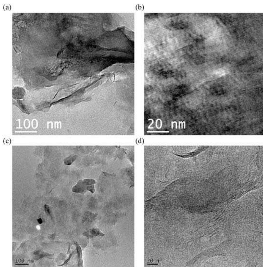
Fig. 4. TEM micrographs of Brazilian clay (a) sodium bentonite (GCGD), (b) expanded view of BSOD, (c) organophilic bentonite (BORG) and (d) expanded view of BORG.
