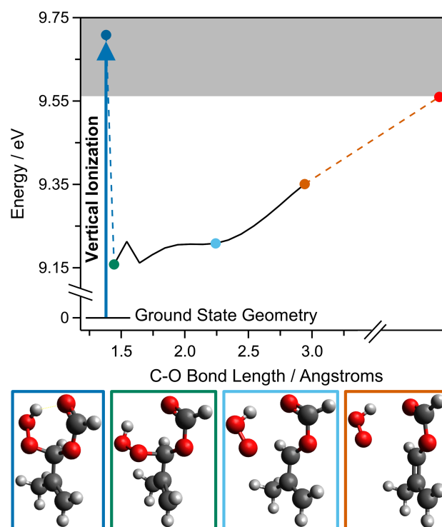
Figure 4. Constrained optimization ( \omega B97XD/6-31+G*) of the C-O bond length associated with \text{HO}_2 dissociation from the HPMAF ion. Significant points included are: Franck-Condon excitation from the equilibrium geometry of the ground state (dark blue), the adiabatic minimum of the ion state (green), an intermediate point along the \text{HO}_2 dissociation coordinate (light blue), separated products in the relaxed optimization (orange), and (red) asymptotic energy for the \text{HO}_2 -loss fragment ion. The grey shaded region illustrates that the \text{HO}_2 + ion co-fragment asymptote is below the calculated vertical ionization energy, suggesting the photoionization process will result in dissociative ionization.
