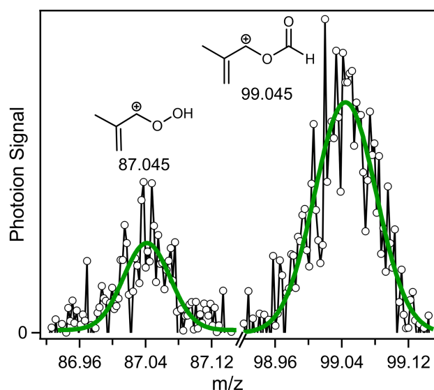
Figure 1. Fragment ions observed in the mass spectrum following reaction of MACR-oxide with formic acid ( 2.6 \times 10^{13} \text{ cm}^{-3} ) using MPIMS. The mass spectrum is obtained by integrating over the full kinetic time window (0–60 ms) and VUV photon energy (9.0–11.0 eV). Gaussian fits to the mass peaks yield exact masses of 87.043 \pm 0.003 and 99.045 \pm 0.002 , consistent with the chemical composition of \text{C}_4\text{H}_7\text{O}_2 (87.045) and \text{C}_5\text{H}_7\text{O}_2 (99.045) corresponding to \text{HCO}_2 -loss and \text{HO}_2 -loss from photoionization of HPMFAF, respectively.
