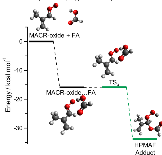
Figure 3. Reaction coordinate showing HPMAF formation from the 1,4-insertion reaction of anti-trans -MACR-oxide with formic acid (FA, green) at the CCSD(T)-F12/cc-pVTZ-F12//B2PLYP-D3/cc-pVTZ level of theory including estimated CCSDT(Q) corrections.
