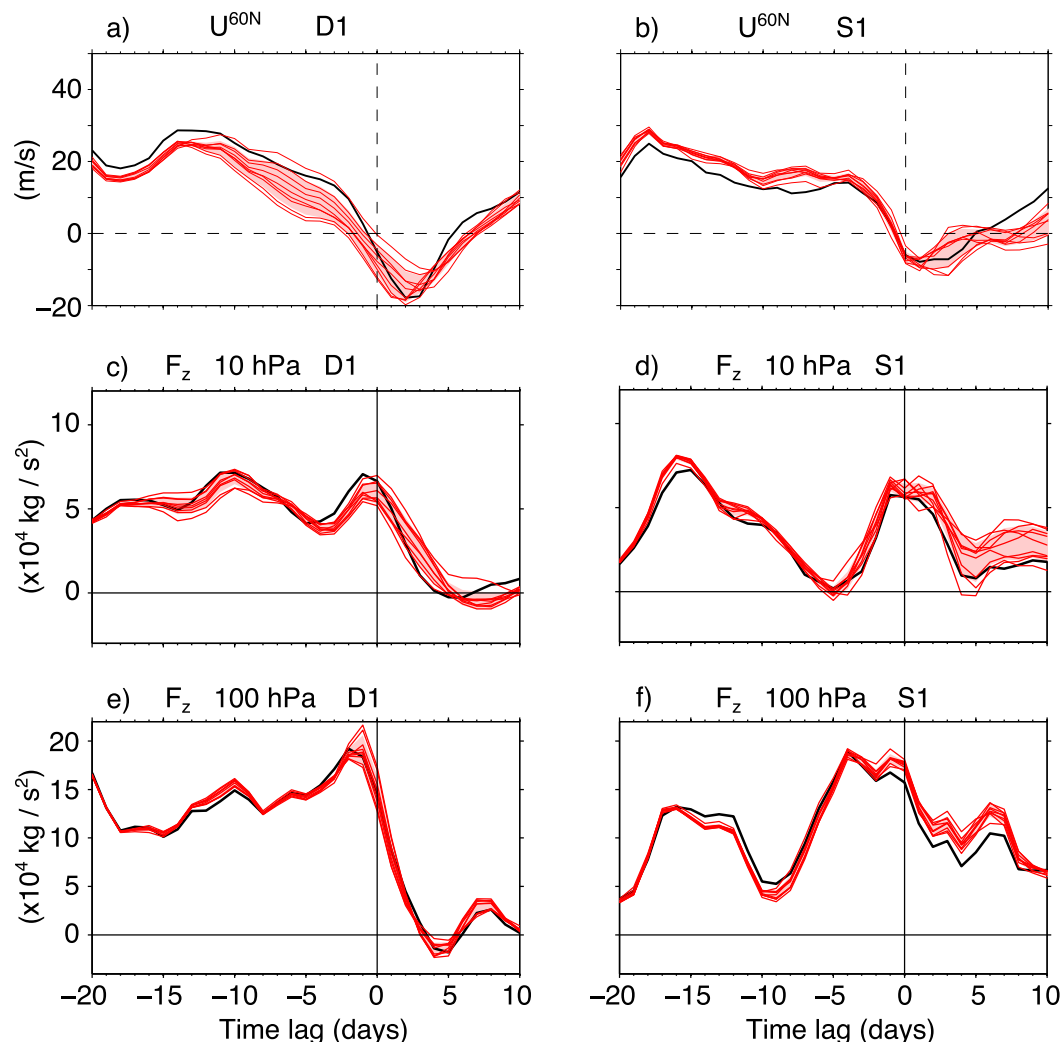
FIG. 14. (top) Zonal-mean zonal wind at 60^{\circ}\text{N} and 10 hPa for (a) CTL-D1 and (b) CTL-S1 (black lines), and the corresponding experiments that do not lead to the SSW when nudging up to 10 km (see Figs. 2b and 6b), but rising the nudging region up to 18 km (red lines). (c)–(f) As in (a) and (b), but showing the corresponding F_z time series at (middle) 10 and (bottom) 100 hPa.
