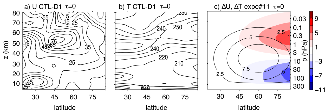
FIG. 1. Initial zonal-mean profiles of (a) zonal wind ( \text{m s}^{-1} ) and (b) temperature (K) in the displacement event analyzed in section 3a (CTL-D1). (c) Zonal-mean perturbations to the initial conditions of zonal wind (contours; \text{m s}^{-1} ) and temperature (shading; K) for experiment 11. See text and Table 1 for details.
