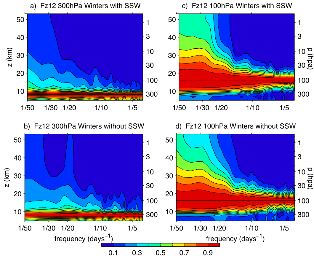
FIG. 15. Coherence squared between the October–March time series of F_z ( s = 1 and 2 ) averaged over 45^{\circ} – 75^{\circ} N at (a),(b) 300 and (c),(d) 100 hPa, and the corresponding time series at all altitudes, for (a),(c) winters with SSW and (b),(d) winters without SSWs.
