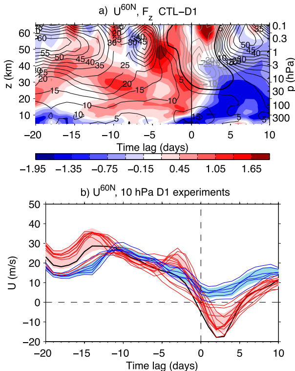
FIG. 2. (a) Time–height evolution of the zonal-mean wind (contours) at 60°N, and the standardized anomalies of the EP flux vertical component (shading) averaged over 45°–75°N, for CTL-D1. Contour interval is 5 \text{ m s}^{-1} , with the zero-wind line in bold; F_z units are multiples of 1\sigma , with a 0.3\sigma interval starting at \pm 0.15\sigma . (b) Zonal-mean zonal wind ( \text{m s}^{-1} ) at 60°N and 10 hPa as a function of time lag about the SSW central date in CTL-D1 (thick black line). Light red (blue) shading represents \pm 1\sigma around the mean of experiments with (without) an SSW.
