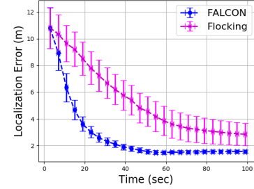
(b) Localization error vs. time
