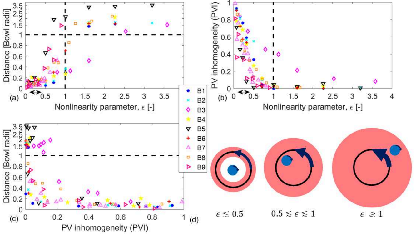
FIG. 5: Regime diagrams for bowl-trapped anticyclone (AC) formation (section 3b). (a) Mean normalized radial position ( D/R_b ) of the emergent anticyclone within the bowl for each free evolution experiment, versus the nonlinearity parameter \epsilon \equiv VH/fH_bL . The radial position r is normalized by bowl radius R_b . Bowl-trapped ACs correspond to D/R_b < 1 . Values D/R_b > 1 are indicative of eddies (including ACs) moving freely across the bathymetry. (b) Position versus the PV inhomogeneity parameter (PVI, equation 6). (c) PVI vs \epsilon . Each different colored marker represents a separate batch of experiments. Within each batch all parameters are kept identical except for the initialization energy E (section 2b). The D/R_b -axis scale is linear (logarithmic) for values below (above) 1. The dashed lines at \epsilon = 1 and at D/R_b = 1 serve as visual aids. In panels (a)–(b), the double-arrow shows the range of \epsilon values estimated to be relevant for the Mann, Lofoten, and Rockall Trough eddies. (d) A schematic illustration of the three regimes described in panels a–c. Note that the states shown are typical but not unique for each regime. For low \epsilon , a trapped AC emerges close to bowl center. For intermediate \epsilon values, a bowl-trapped AC typically emerges, but can occur at some finite bowl-radius, since the intensified slope current (arrow) causes partial or complete PV homogenization (illustrated in red) within the bowl and outside of the AC. For high \epsilon , the eddies are free to move across the slope and are not trapped within the bowl.
