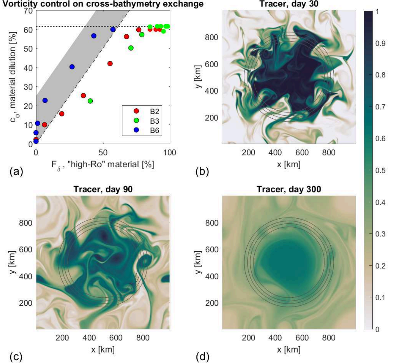
FIG. 9: Contribution of anticyclones originating outside the bowl to the bowl-trapped anticyclone. (a) Anticyclone material fraction originating from outside of bowl ( c_o ), versus F_\delta : the percent of initial material with \delta = H\zeta/fh \geq 1 , i.e., anomalously high Rossby (Ro) number. The fraction c_o is estimated from the late-time tracer concentration c averaged between r = 0 and r = R_b/2 , since initially c = 1 (0) inside (outside) of the slope region, with a transition region on the slope. Experiments in which a trapped anticyclone forms are shown by a black edge to the marker. The horizontal (dotted) line shows the maximal dilution possible in case of homogeneous final state. Different experiment batches (table 1) are denoted by different colors (legend). The diagonal (solid) line shows a hypothetical c_o = F_\delta relation. The amount of bowl anticyclone material in the final state originating from outside the bowl is quite close to the fraction of material with initial \delta \geq 1 . Deviations above the unit line are likely partially due to material originating over the narrow slope region, where 0 < c < 1 at t = 0 . The maximal possible bias due to this effect is shown by the gray area. (b–d) Simulated tracer concentrations at three different times for experiment B2E4. Topographic contours (4100, 4200, 4300, 4400 m depth) are shown in solid lines.
