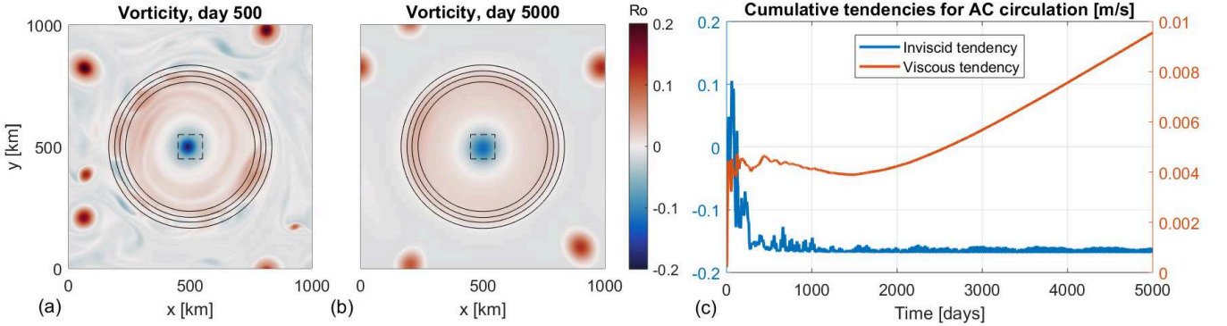
FIG. 7: Long-time evolution of bowl-trapped anticyclone. Panels (a) and (b) show the instantaneous vorticity (in f units) distribution at days 500 and 5000, respectively, for experiment B1E3L . Topographic contours (4100, 4200, 4300, 4400 m depth) are shown in solid lines. The dashed square line in panels a–b shows the line along which circulation tendencies are calculated in panel c. Panel c: time-cumulative inviscid (blue) and viscous (red) circulation tendencies inside the bowl (just outside the anticyclone peak velocity radius, along the dashed lines of panels a–b). The cumulative tendencies are normalized by the perimeter of the dashed square such that they have dimensions of mean velocity, i.e., m/s.
