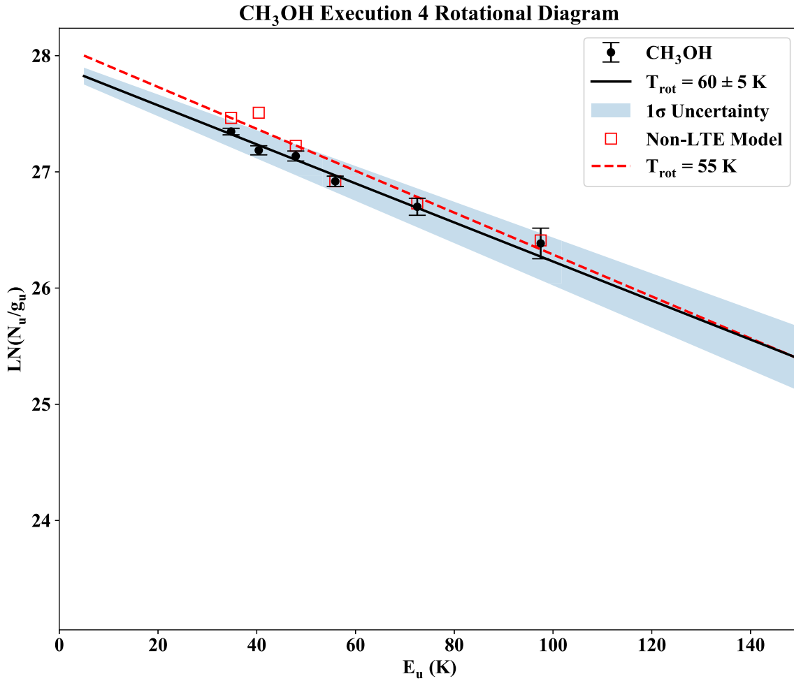
Figure 4. Rotational diagram of the \text{CH}_3\text{OH} 5_0-4_0 A^+ , 5_{-1}-4_{-1} E , 5_0-4_0 E , 5_1-4_1 E , 5_2-4_2 A^+ , and 5_{-3}-4_{-3} E transitions in Wirtanen on UT 2018 December 9 during Execution 4 (black circles, Tables 1 and 2), along with the best-fit line (black, solid), corresponding to T_{\text{rot}} = 60 \pm 5 K, and the 1\sigma uncertainty in the fit (blue shaded area). Also shown is the rotational diagram for a non-LTE model with T_{\text{kin}} = 60 K (red squares) and the best-fit line (red, dashed) corresponding to T_{\text{rot}} = 55 K, illustrating formal agreement between the observations and the model.
