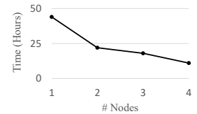
Figure 9: Performance by #nodes (scale 2, 1k, 60 minutes).
