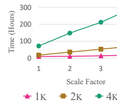
Figure 8: Performance by scale/resolution (4 nodes, 60 minutes)
