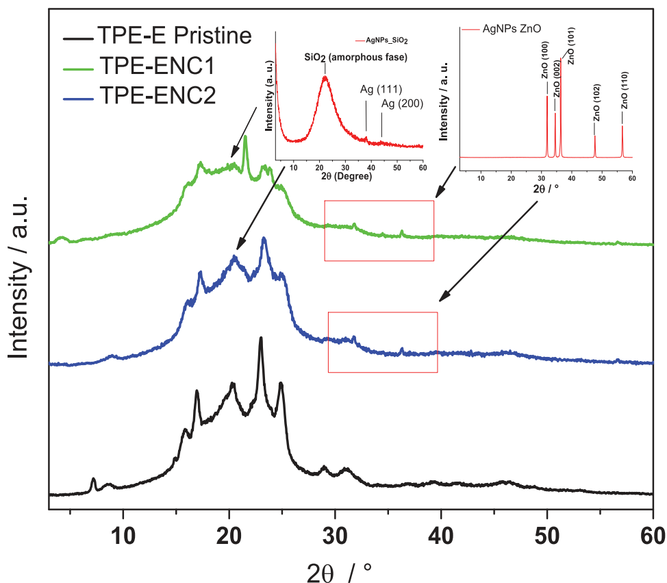
Fig. 8 XRD Diffractograms of films from extrusion of: Pristine TPE-E; TPE-ENC1 and TPE-ENC2 with \text{AgNPs@ZnO/SiO}_2
