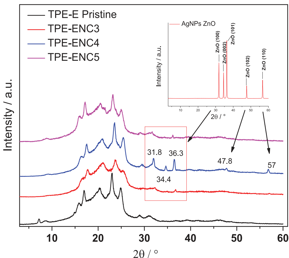
Fig. 9 XRD Diffractograms of films from compression molding of: Pristine TPE- E, TPE-NC3 and the films irradiated at 20 kGy, TPE-ENC4 and 50 kGy, TPE- ENC5
