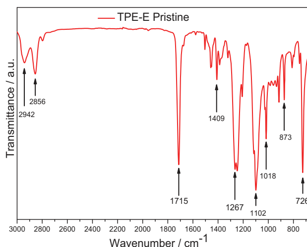
Fig. 3 FTIR-ATR spectra of pristine TPE-E
