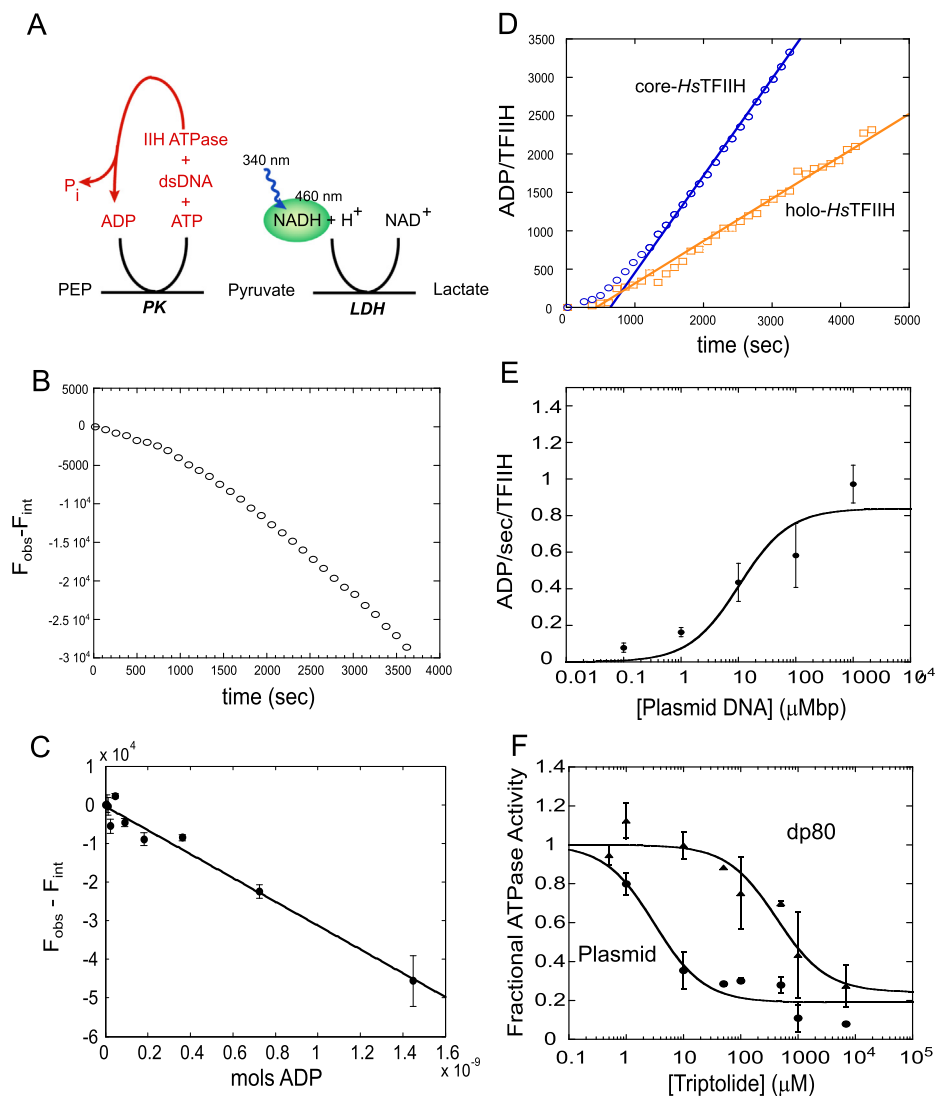
Figure 1. Human TFIIH core ATPase is stimulated by dsDNA and is XBP-dependent. (A) Diagram of the continuous, fluorescent, enzyme-coupled ATPase assay used to measure TFIIH steady-state ATPase activity. TFIIH ATP hydrolysis was monitored by following the oxidation of NADH to NAD through the regeneration of ADP to ATP through the glycolytic enzymes pyruvate kinase and lactate dehydrogenase. NADH fluorescence at 460 nm is quenched upon NADH oxidation to NAD. (B) Observed fluorescence decrease relative to the initial value ( F_{obs} - F_{int} ) time-course of core-HsTFIIH ATPase activity in the presence of 100 \mu M-bp plasmid DNA after subtracting a control-time course of core-HsTFIIH in the absence of DNA. (C) ADP standard curve for converting observed NADH fluorescence to moles of ADP. (D) Representative ATPase time courses for core- and holo-HsTFIIH. The core-HsTFIIH, time course is the same time course in (B) converted to ADP/HsTFIIH using the standard curve in (C) and the moles of HsTFIIH determined by SDS-PAGE as described in Materials and Methods. The slope of a linear fit is the observed rate of ATP hydrolysis. (E) The rate of core-HsTFIIH ATP hydrolysis as a function of plasmid DNA concentration. The trends are fit with the Michaelis-Menten equation (solid line), see Materials and Methods. (F) Triptolide inhibition curves for core-HsTFIIH ATPase in the presence of plasmid (circles) and linear dsDNA (80 bp, triangles).
