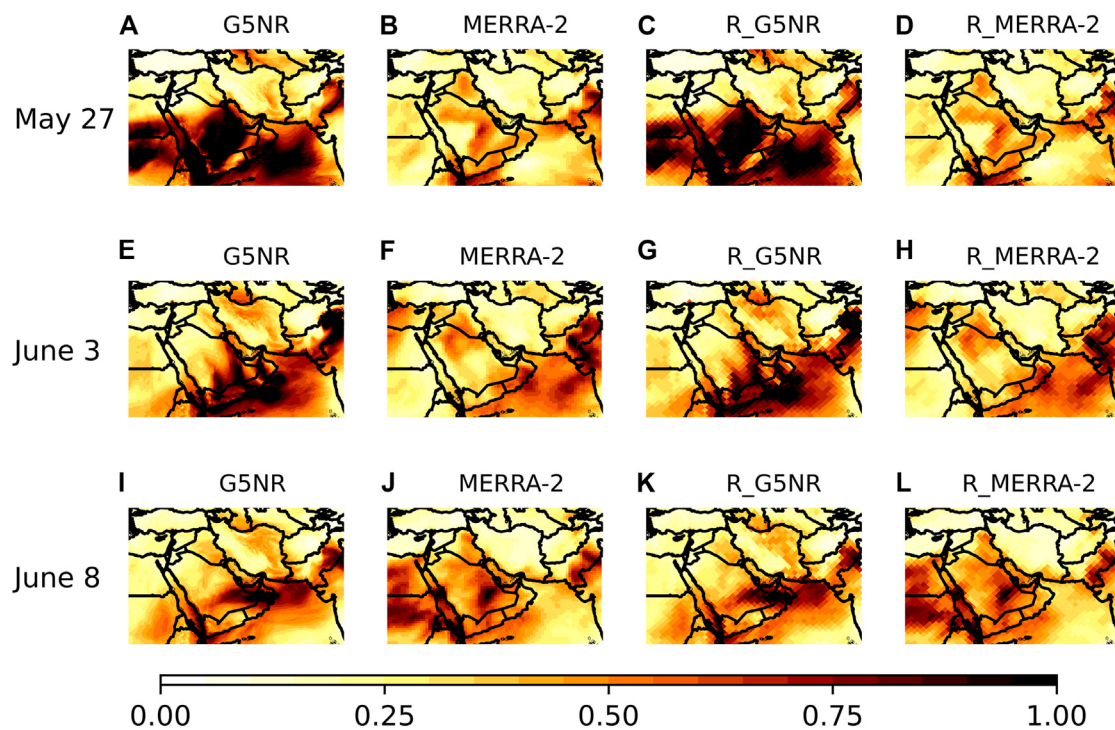
FIGURE 1 | (Top) Daily mean AOD from (A) G5NR and (B) MERRA-2 on May 27th, 2006. (C) and (D) are remapped (A) and (B) into lower-resolution pixels with 102 km grid spacing. (Middle) (E)–(H) are same as (A)–(D), but for June 3rd, 2006. (Bottom) (I)–(L) are same as (A)–(D) but for June 8th, 2006.
