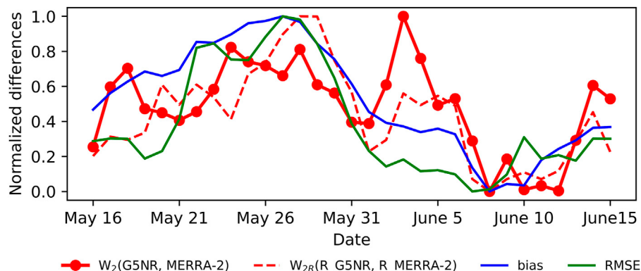
FIGURE 3 | The red solid line represents normalized W_2 between daily AOD maps from G5NR and MERRA-2. Normalized W_{2R} (red dashed line), biases (blue solid line), and RMSEs (green solid line) were calculated between R_G5NR and R_MERRA-2 daily AODs from May 16th, 2006 to June 15th, 2006.
