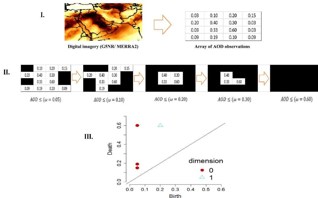
FIGURE 2 | Illustration of cubical complex filtration with its respective summary of topological features. (I) A map of AOD observations, which can also be viewed as a two-dimensional array. (II) Filtration of cubical complexes from the array of AOD observations. Shaded regions constitute two-dimensional elementary cubes (i.e., squares) formed as the similarity scale changes. (III) Persistence diagram reflecting the lifespan of connected components (0-dimensional objects) and holes (1-dimensional objects) seen in II.
