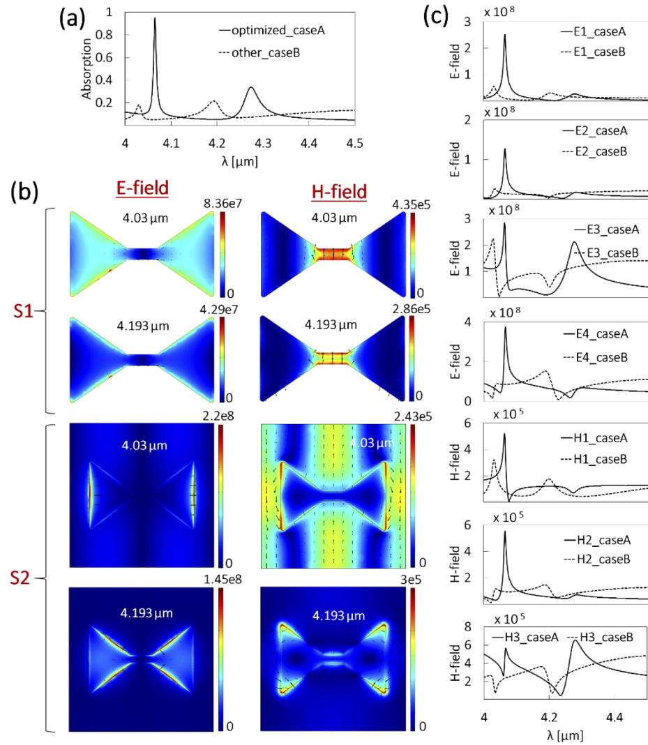
Fig. 5. Fano resonance investigation as a comparison of two geometrical cases of strong (optimized) and weak far-field absorptions. (a) Far-field A-spectra for cases A and B. (b) Near field spatial E-field and H-field at resonances on surface S1 (upper exposed diabolo antenna) and S2 (bottom bowtie aperture antenna) for Case B. (c) Spectral E- and H-field comparison of both cases at EM hotspots.
