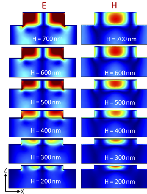
Fig. 8. Effect of varying H of the absorber FEM simulation results showing longitudinal ZX E-field (column 1) and H-field (column 2) distributions as a function of increasing H .
