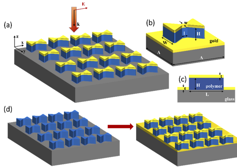
Fig. 1. (a) Schematic of gold coated diabolo array antenna based under x-polarized electric field illumination. (b) Lattice single unit of the array with structural parameters indicated. (c) Vertical cross-section view of the lattice single unit cell showing the meta-surface layer by layer design. Optimized dimensions are lattice periodicity, \Lambda = 4 \mu\text{m} ; thickness of dielectric deposited on glass, H = 600 \text{ nm} ; antenna length, L = 2.5 \mu\text{m} ; antenna width, W = 1.5 \mu\text{m} ; neck length of antenna, l = 600 \text{ nm} ; neck width of antenna, w = 250 \text{ nm} , thickness of gold coating, t = 55 \text{ nm} . (d) Schematic of the two-step fabrication process, a lithography or laser-direct-write process followed by a metallization process.
