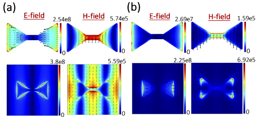
Fig. 3. E-field [V/m] and H-field [A/m] distribution plots and field directions at resonance wavelengths (a) 4.065 \mu\text{m} and (b) 4.277 \mu\text{m} along the transverse XY plane on surfaces S1 (row 1) and S2 (row 2).
