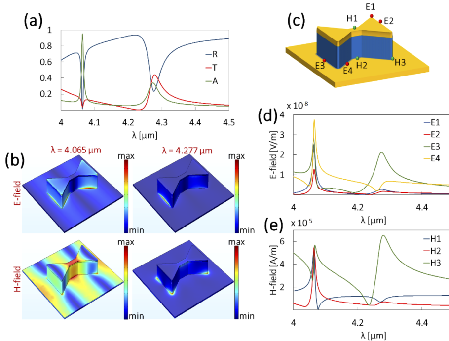
Fig. 2. FEM calculations (a) R, T, A of our MM for x-polarized incident light with resonances at 4.065 \mu\text{m} and 4.277 \mu\text{m} . (b) Perspective views of E-field and H-field spatial distributions at resonances (c) Locations of E- and H-field hotspots (d) Spectral near-field electric field intensities at E-field hotspots (e) Spectral near-field magnetic field intensities at H-field hotspots.
