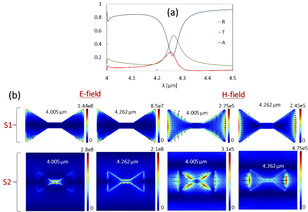
Fig. 6. FEM simulation results (a) R, T, A of our MM for TM polarized incident light with resonances at 4.005 \mu\text{m} and 4.262 \mu\text{m} . (b) Field distribution plots and field directions at resonances along the transverse XY plane on surface S1 [upper exposed diabolo antenna] (row 1) and surface S2 [bottom bowtie aperture antenna] (row 2); E-field [V/m]: H-field [A/m]
