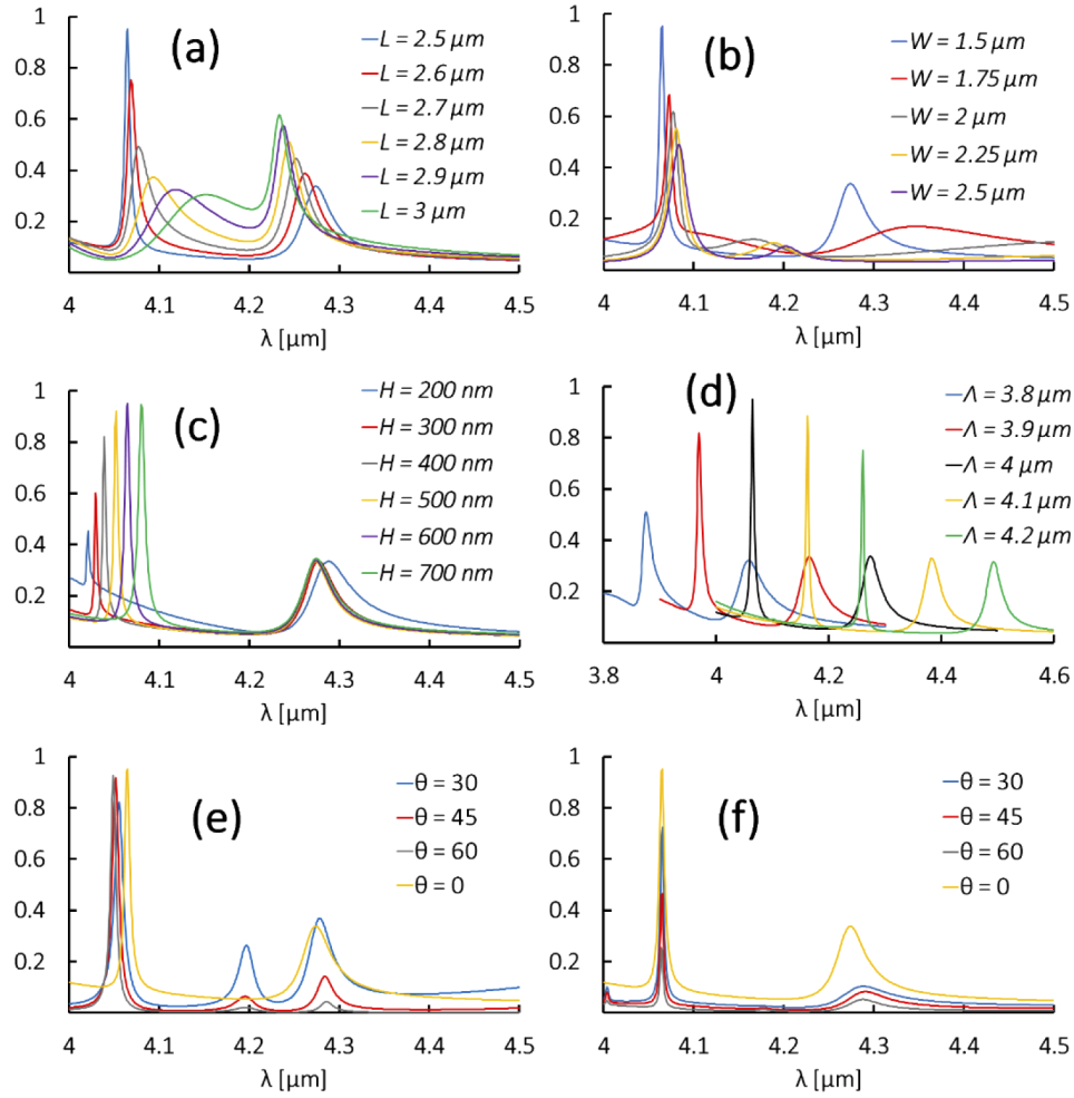
Fig. 4. Far-field A-spectra for variation of (a) L (b) W (c) H (d) \Lambda (e) \theta in XZ plane and (f) \theta in YZ plane.
