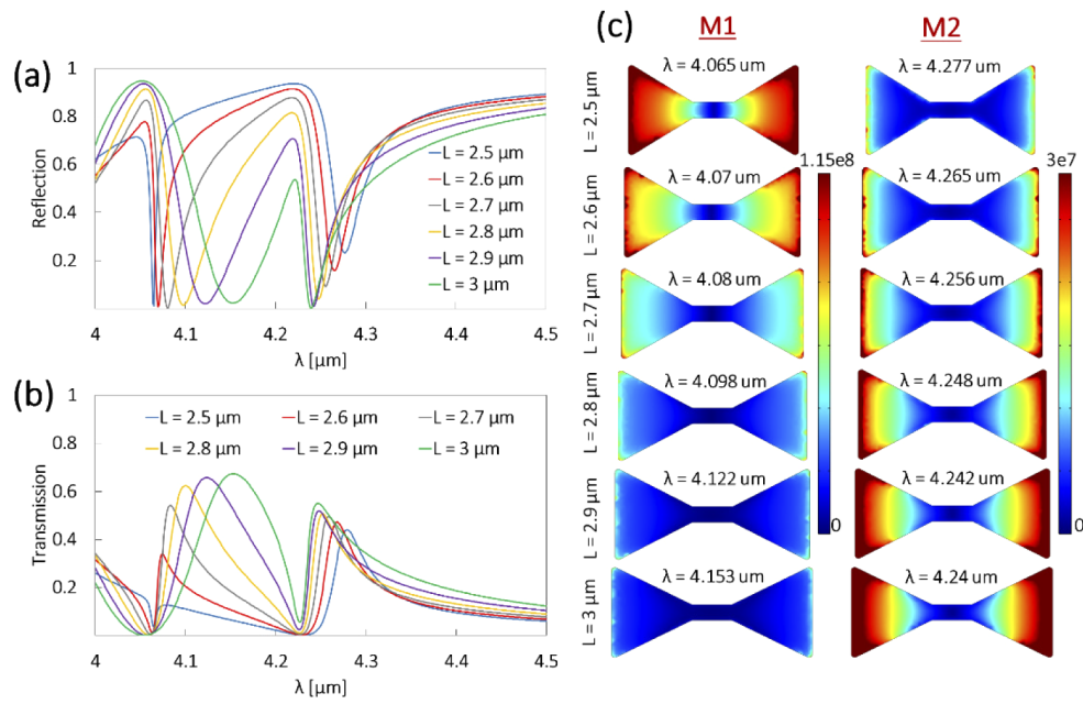
Fig. 7. FEM simulation results (a) R and (b) T spectra for variation of L (c) Surface E-field distribution at S1 for plasmonic state in first band M1 and plasmonic state in second band M2 at the LSP wavelengths corresponding to each L varied.
