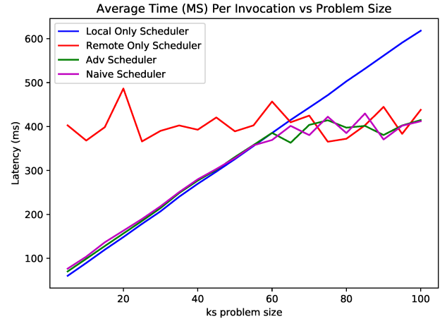
Fig. 11. In this chart is a latency comparison for all four schedulers (local, remote, naive, and adv)
