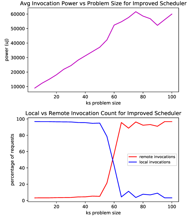
Fig. 10. Top: average invocation power draw as a function of KS problem size for the improved scheduler. Bottom: local invocation count vs remote invocation count selected by the scheduler for each problem size.
