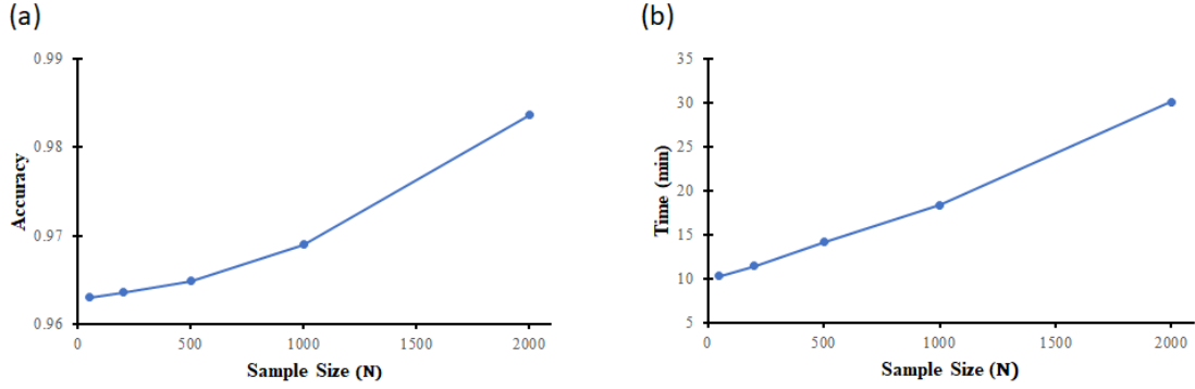
Fig. 2. The effect of number of samples N used for EnDP on the test accuracy and training time for MNIST dataset is presented. (a) Test accuracy increases as N increases. (b) Training time (in minutes) for one epoch as N is increased.
