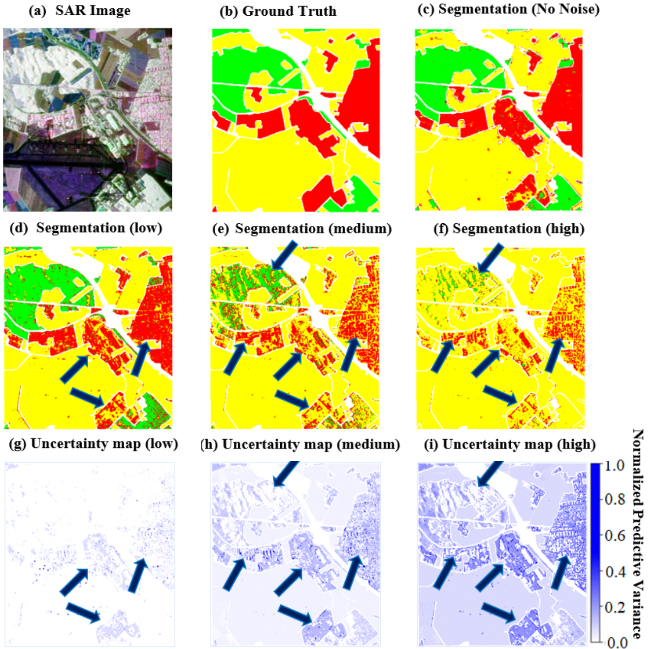
Fig. 13. Oberpfaffenhofen SAR dataset: (a) the original SAR image, (b) the ground truth, (c - f) the predicted segmentation by the proposed exVDP model before and after adding three levels of adversarial noise (low , medium and high), and (g - i) the uncertainty maps of the exVDP model for the three levels of adversarial noise. The class label "open areas", which is the target of the attack, is represented by the yellow color in the ground truth image. The arrows refer to the pixels that are misclassified as "open areas" and to the uncertainty associated with those pixels in the uncertainty maps.
