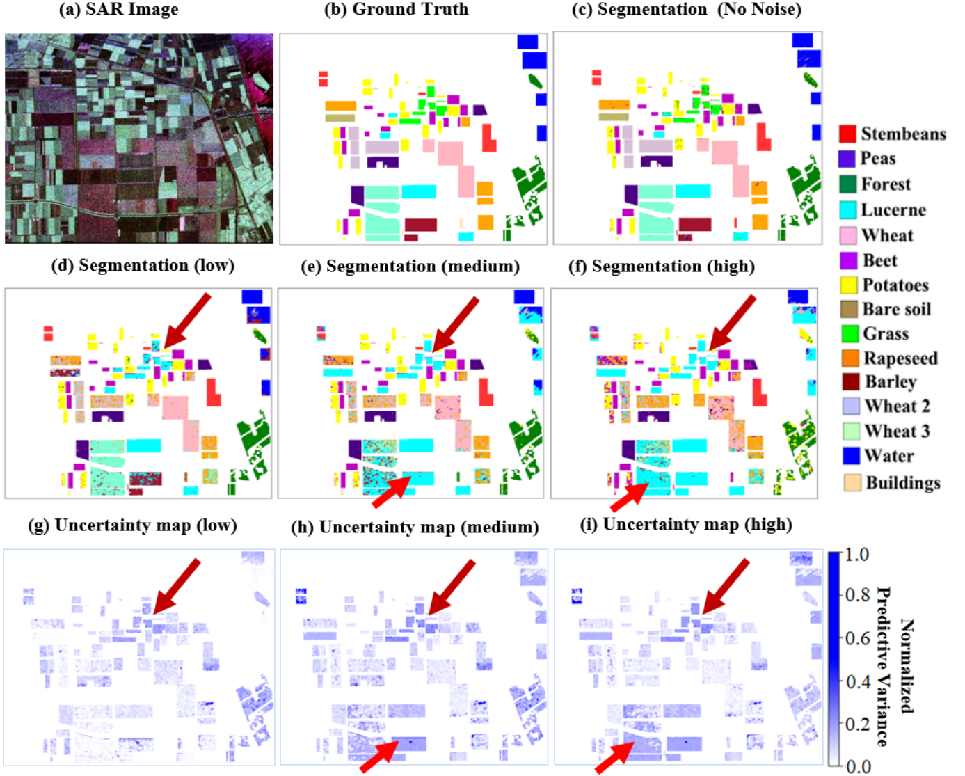
Fig. 12. Flevoland dataset. (a) The original RGB pseudo-color SAR image of Flevoland. (b) The ground truth map of the target scene. (c - f) The predicted segmentation by the proposed exVDP model before and after adding three levels of adversarial noise (low, medium and high). (g - i) The uncertainty maps of the exVDP model for three levels of adversarial noise. The class label "lucerne", which is the target of the attack, is represented by the cyan color in the ground truth. The arrows refer to the pixels that are misclassified as "lucerne" and to the uncertainty associated with those pixels in the uncertainty maps.
