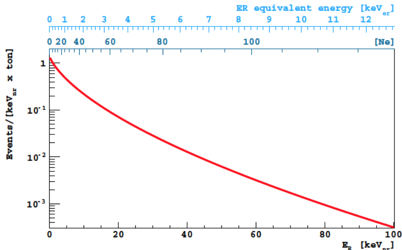
Figure 2. Nuclear recoil energy spectrum from neutrino interactions in LAr via CE \nu NS from a core-collapse 27 M_{\odot} supernova at 10 kpc.
