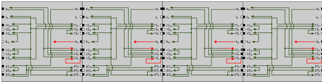
Figure 15 An example which verifies completion of an “off” signal. (a) An off signal is fired from another glue in the STAM tile. Notice that an off signal is denoted by a red arrow. (b) Upon signal execution, the S_{Lglue} turns off. (c) This causes the right STAM tile to detach. (d) A new tile may now attach, sending a signal which confirms that the S_{Lglue} has successfully been turned off.
