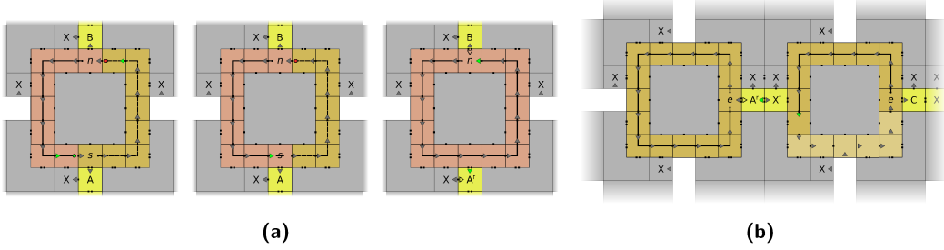
■ Figure 10 (a) Overriding illustration of the transition signal originating from the s state by the signal originating from the n state. This event is then detected by the failed transitioned domino with the fail state A^f . (b) An example of two transition dominoes competing to cycle a macroblock's wire. Given that the middle transition domino's right state tile is the failed state X^f , the left state tile proceeds by representing the replace state A^r .
