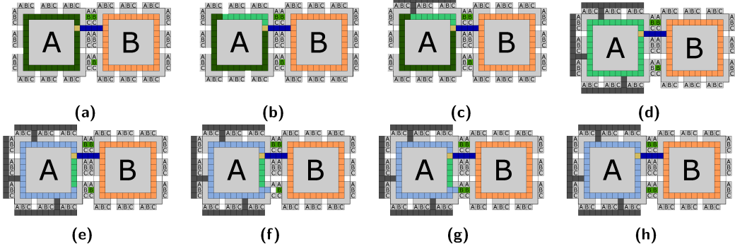
■ Figure 20 (a-d) Phase 1 of the transition process is responsible for attaching dummy polyominoes to ensure no neighbors are currently transitioning. (e-h) Phase 2 of the transition process sends a counterclockwise signal which activates all glues of the state being transitioned to.
