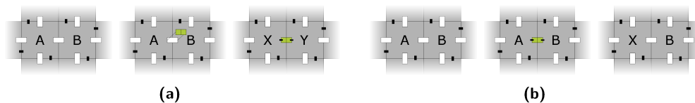
Figure 6 (a) In order for a single-transition system to simulate a double-transition system, we use the attachment of a transition domino. The mapping of both macroblocks can be changed simultaneously with the attachment of such a domino. (b) The key concept behind the bonded portion of the simulation is the transition domino. Adjacent macroblocks (bonded or not) allow for the attachment of a transition domino which may allow communication of transition information.
