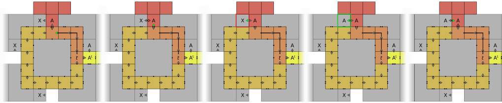
■ Figure 12 Illustration of a t-shape dummy polyomino attaching to the north side of a macroblock, replacing the X glue tile with A glue tile.
