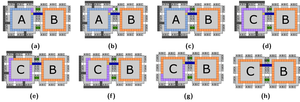
Figure 21 (a-d) Phase 3 of the transition process sends a counterclockwise signal which deactivates all glues of the previous state and replaces them with dummy tiles. (e-h) Phase 4 refreshes the wire for the new state, and detaches all dummy blocks as well as the transition polyomino.
