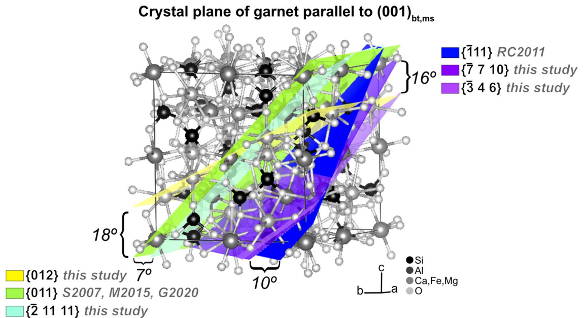
Figure 5. Comparison of crystal planes discussed in this study with others previously described as being preferentially parallel to (001)_{bt,ms} [RC2011 = Ruiz Cruz, (2011), S2007 = Spiess et al., (2007), M2015 = Moore et al., (2015), and G2020 = George and Gaidies, (2020)].
