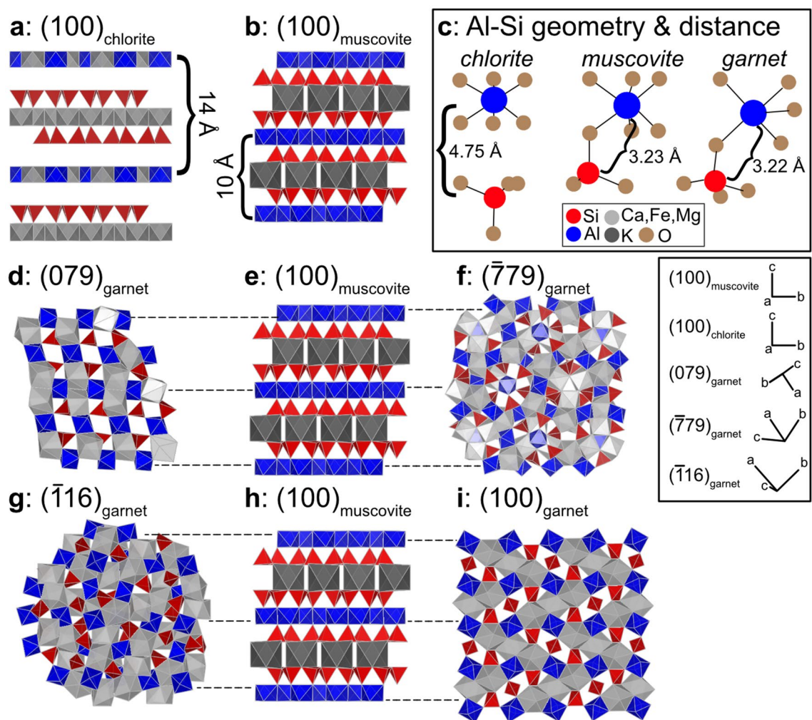
Figure 4. Crystal structure models of (a) chlorite 48 and (b) muscovite 30 . (c) Al octahedra–Si tetrahedra geometries and distances in chlorite, muscovite, and garnet. (d–i) Crystal structure models of (079) gt , (100) ms , (779) gt , (116) gt , (100) ms , and (100) gt , with dashed lines highlighting relationships between Al in each. The inset shows the 3D orientation of all of the crystal planes.
