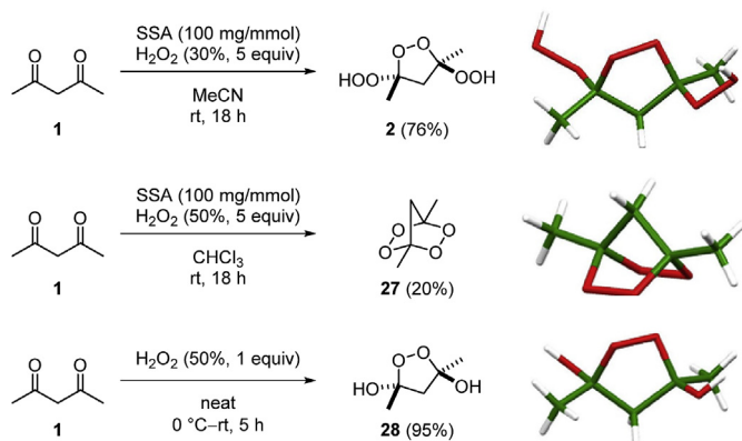
Scheme 3. Preparation and single crystal X-ray structure of potential reactive species.
