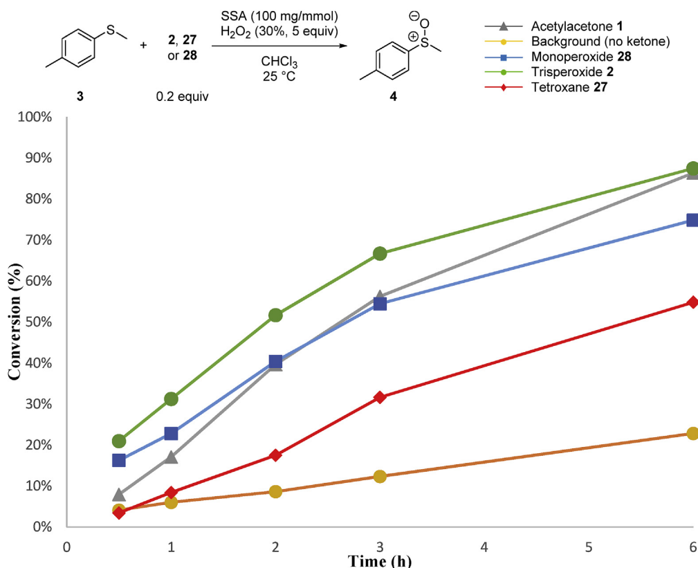
Scheme 4. Relative activity of peroxides 2 , 27 and 28 within the catalytic sulfoxidation process.
