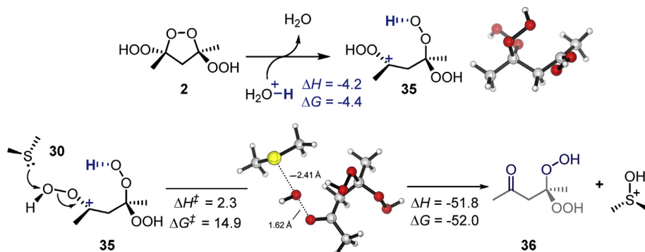
Scheme 7. Protonation of endocyclic oxygen in peroxide 2 leads to a favorable reaction with the sulfide nucleophile.
