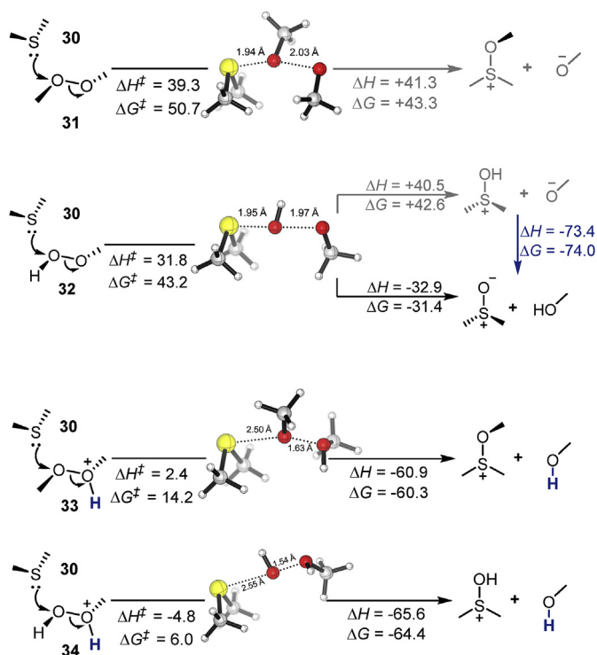
Scheme 6. Reactions of dimethyl sulfide 30 with neutral and protonated parent organic peroxide and hydroperoxide.
