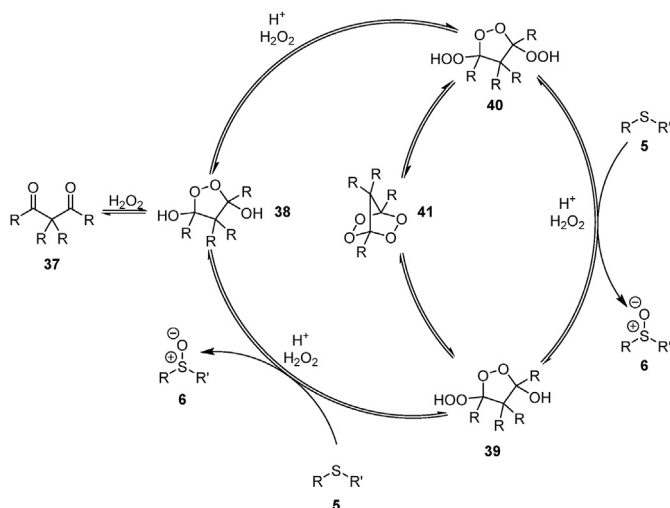
Scheme 8. Proposed catalytic cycle.
