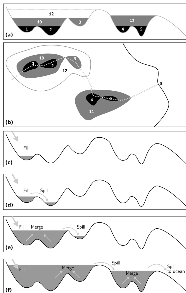
Figure 3. The Fill–Spill–Merge process. Water moves through topographic depressions by filling them, spilling over sills, and merging to form meta-depressions. (a) Topographic cross section with labeled leaf depressions and their parents, following the left-hand side of the depression hierarchy in Fig. 2. The number 0 represents the ocean; other numbers represent leaves and parents that together form depressions and meta-depressions. (b) Map showing this depression structure; the cross section in (a) follows the dotted gray line. (c) A water source to the left begins to fill depression 1. (d) Continued water input causes depression 1 to overflow and spill into depression 2. (e) Depression 2 fills, causing depressions 1 and 2 to fill their parent (10) and merge to form a meta-depression. This meta-depression overflows into depression 3. (f) Depression 3 fills and merges with meta-depression 10 (1 and 2 being implied members based on their position in the hierarchy) to flood their parent, 12. After meta-depression 12 overflows, it enters depression 4, which then fills and spills into depression 5. After depression 5 floods, its waters join with those from depression 4 to fill meta-depression 11, which then spills to the ocean. Figures 4 and 5 describe the algorithm in more specific detail.
