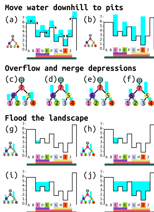
Figure 4. Visual overview of the algorithm. Black outlines represent the elevations of the cells. Blue areas are the heights of water in each cell or depression within the depression hierarchy. Capital letters label cells, and numbers on colored dots label depressions. Colors at the base of each panel match the colored dots and indicate to which depression each cell belongs. The algorithm consists of three major stages (Fig. 5). From its initial distribution (a), water is moved downhill following flow directions in the steepest downslope direction from each cell, as indicated by the arrows. Water continues to move downslope until it reaches the pit cells (b, Sect. 3.1). Water is then moved within the depression hierarchy (c–f, Sect. 3.2). (c) The initial distribution of water within the depression hierarchy based on how much water was in the pit cell of each depression. Water in depressions with insufficient volume overflows first into their sibling depressions and then – if the sibling depression becomes filled – passes to their parents. All of the leaf depressions in (c) are completely filled, so no sibling depressions can accommodate more water. Therefore, depressions 1 and 2 pass their overflowing water up to their parent, depression 6, and depressions 3 and 4 pass their overflowing water up to their parent, depression 5. (d) Depression 6 is now overflowing, but its sibling, depression 5, is not full, so depression 6 passes as much of its overflowing water as it can to depression 5. (e) Once depression 5 is full, some overflowing water still remains, so this is passed to the parent, depression 7. (f) In this case, depression 7 is able to accommodate the remainder of the water. Had depression 7 also overflowed, the leftover water would have overflowed into the ocean and been disregarded. Depressions to be flooded are then identified and flooded (Sect. 3.3). Since depression 7 contains water, we know that all of its descendants must be completely full. Therefore, we can flood these all at the same time on the level of depression 7. Any one of the pit cells within depression 7 is arbitrarily selected as the starting point (g). More cells are added until all of the water has been accommodated. Panels (h–j) are a visual representation of this process, although the algorithm would first locate affected cells C–J and then calculate the final height of water in all of these cells in a single step.
