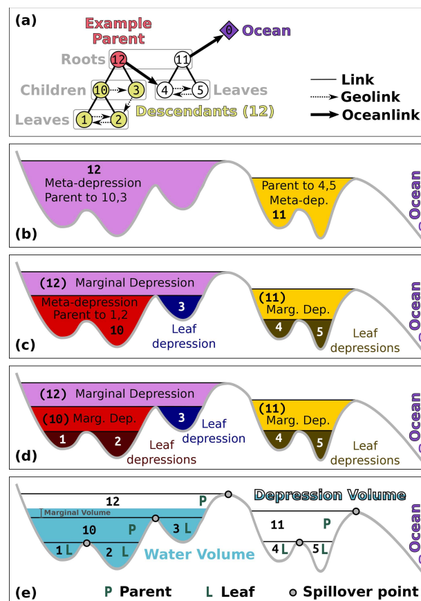
Figure 2. Terminology for the depression hierarchy and water flow through it. The depression hierarchy shown here is drawn from the left-hand side of Fig. 1 from the companion paper by Barnes et al. (2020). (a) Topology. A parent and its descendants are associated with depressions (b–d). Direct descendants are called children . Leaves are the terminal members of the depression hierarchy; they have no children and represent simple depressions (i.e., those that are not meta-depressions). Members of a single binary tree are joined in their hierarchy through links ; directional links that represent water-spillover directions between geospatially adjacent depressions are called geolinks . Flow from one binary tree into another and towards the ocean follows the oceanlinks . Though only one binary tree is shown, the ocean may be the parent to an arbitrarily large forest of binary trees. (b) Parents in the hierarchy form meta-depressions – depressions that encompass other depressions. (c) These meta-depressions contain leaf depressions – depressions that themselves contain no depressions. These are associated with leaves in the depression hierarchy. Meta-depression 12 also contains another meta-depression, 10. The regions of depressions 11 and 12 that lie above their child depressions are termed “marginal depressions”. (d) Meta-depression 10 contains leaf depressions 1 and 2. (e) Using the depression hierarchy to simulate water flow. Water first fills leaf depressions before flooding into neighboring depressions. Once a depression and its neighbor are completely filled, their parent begins to flood. The depression volume is the full geometric volume of the depression. The water volume, naturally, is the volume of water within a given depression. The marginal volume is the volume of water partially filling the top-level meta-depression; appropriately spreading this water across the landscape is the topic of Sect. 3.3.
