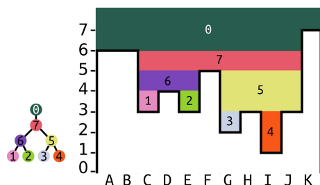
Figure 1. A single subtree of a depression hierarchy and the depression it represents. Depressions 1–4 are leaf depressions. Depression 6 is a parent depression (also termed a meta-depression) that contains depressions 1 and 2. Water from the plateau on the left above cells A and B might fill depression 1 (cell C), causing it to spill into depression 2 (cell E). Only when both depressions are full do they merge and begin filling depression 6 (cells C, D, and E). Modified from Barnes et al. (2020).
