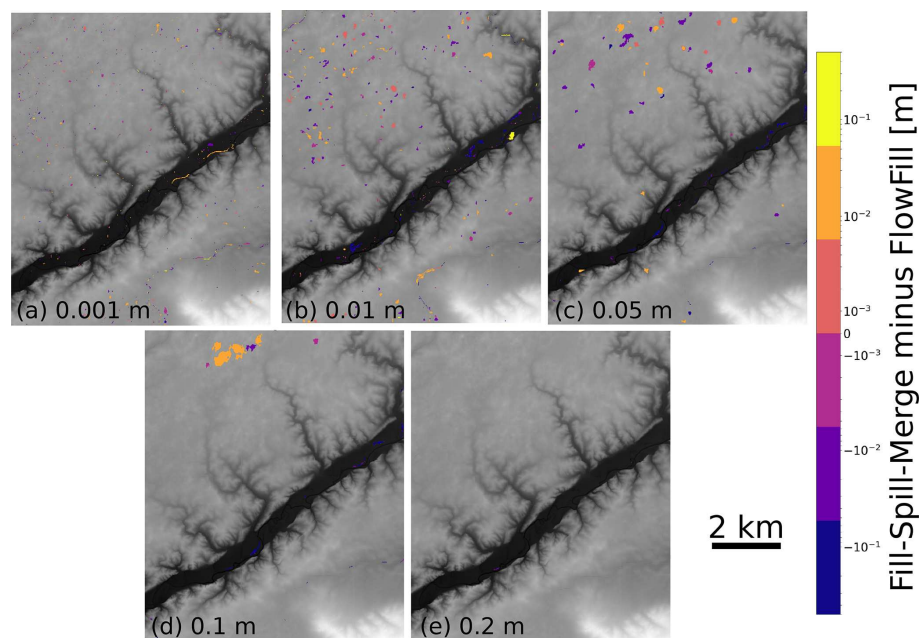
Figure 7. The difference between results of Fill–Spill–Merge and FlowFill at the Sangamon River site. The values for panels (a) to (e) indicate the depth of uniform runoff applied across the landscape for both algorithms. For example, in (a), each cell across the domain starts with 0.001 m of surface water. Orange to yellow indicates locations where Fill–Spill–Merge had more water, and purple to blue indicates locations where FlowFill had more water. Differences of less than 3 mm have been masked out. Differences are generally small and are likely a result of the iterative nature of the FlowFill algorithm, which causes it to asymptotically approach the correct values. In some locations, Fill–Spill–Merge retains slightly more water in depressions than FlowFill does. This could be due to water that has not yet finished moving downslope and into these depressions in the FlowFill algorithm. In other locations, FlowFill has retained more water. One possible reason for this is that some depressions have a narrow outlet through which Fill–Spill–Merge is able to move all water as appropriate, but the cell-by-cell movement of water with FlowFill can produce transient dams that reroute additional water towards these subcatchments. This DEM was prepared by Lai and Anders (2018) and Callaghan and Wickert (2019) from lidar topographic data provided by the Illinois State Geological Survey (Illinois Geospatial Data Clearinghouse, 2020).
