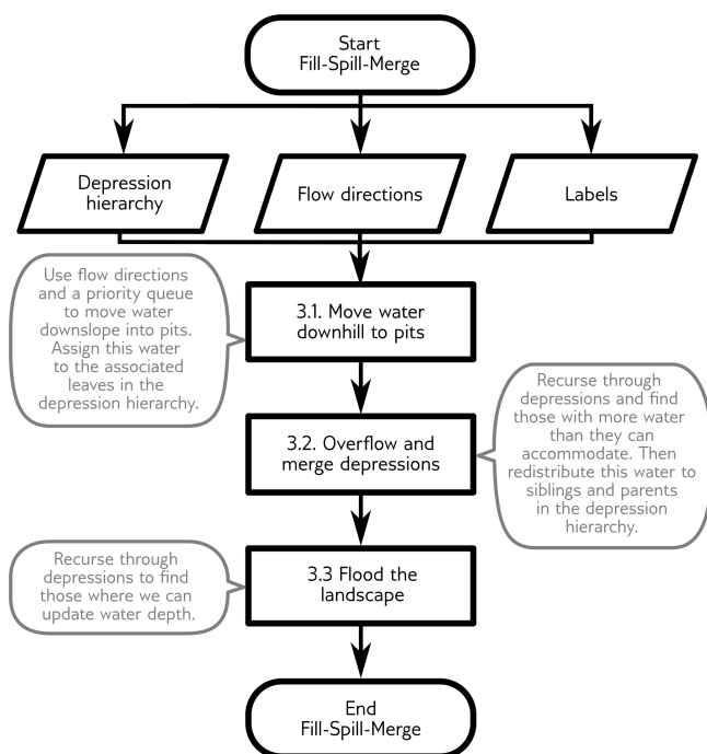
Figure 5. Flowchart showing the main steps taken by the algorithm. These steps are described in more detail in Sect. 3.1 to 3.3.
