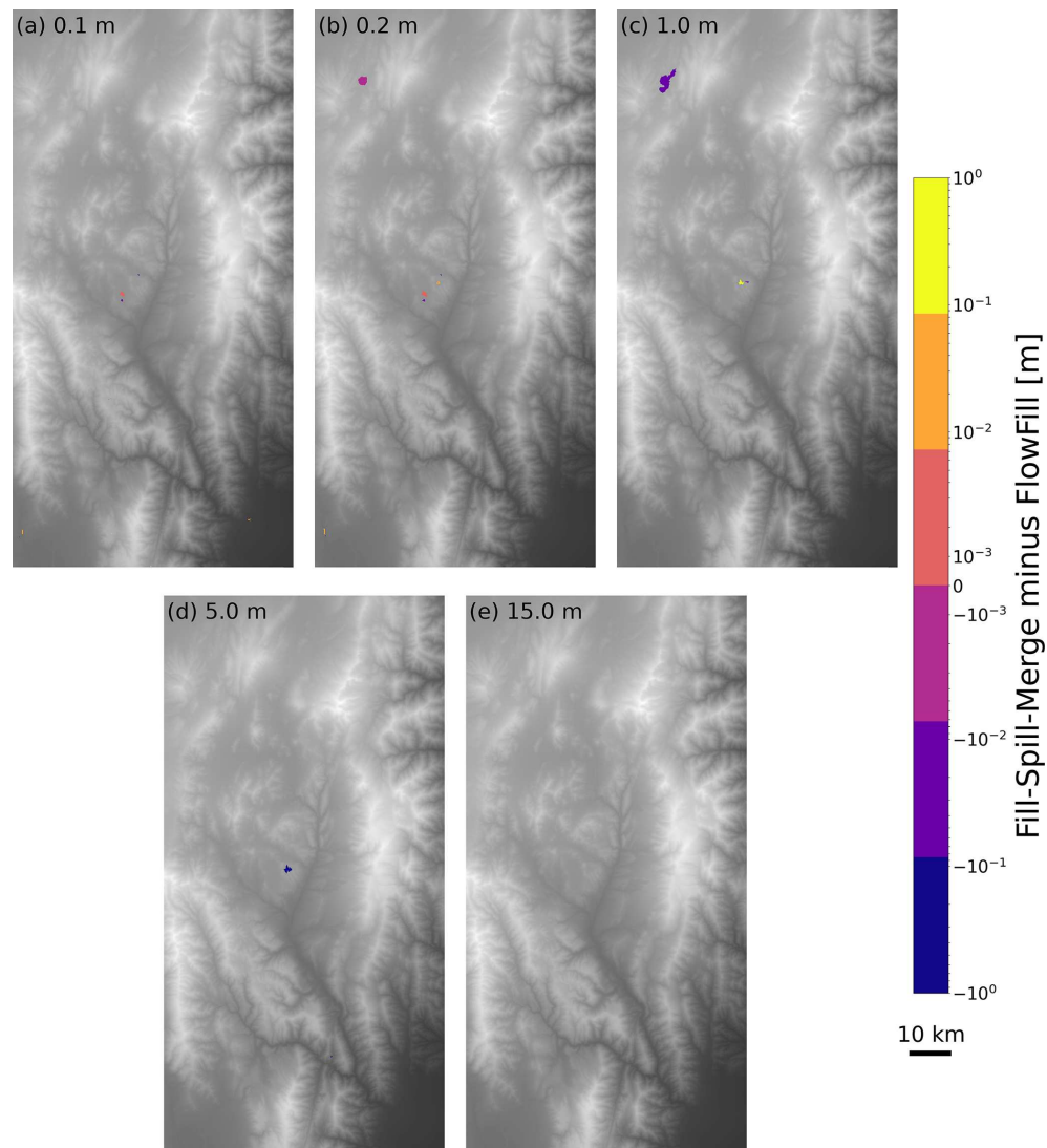
Figure 8. The difference between results of Fill–Spill–Merge and FlowFill at the Río Toro site. The values for panels (a) to (e) indicate the depth of uniform runoff applied across the landscape for both algorithms. For example, in (a), each cell across the domain starts with 0.1 m of surface water. Orange to yellow indicates locations where Fill–Spill–Merge had more water, and purple to blue indicates locations where FlowFill had more water. Differences of less than 3 mm have been masked out. In panel (e), 15 m of water was enough to fill all depressions with both algorithms, so there are no differences between the two. The most significant difference is seen in panel (c), where FlowFill retained additional water in a large depression. This is likely due to transient damming of its narrow inlet in FlowFill’s cell-by-cell method of moving water, which may have prevented the full volume of water from leaving the depression. This DEM was generated with data acquired from the TanDEM-X mission (Krieger et al., 2013; Rizzoli et al., 2017).
