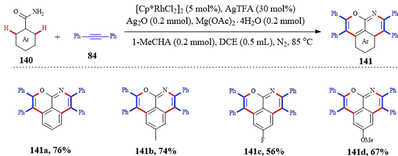
Scheme 85. Rh-Catalyzed Double Ortho -C–H Activation/Annulation of Benzamides with Aryl Alkynes
