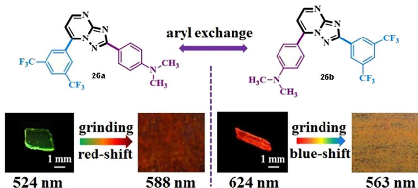
Figure 5. Photographs of Single Crystals and Ground Samples of 26a and 26b under UV Light (365 nm)
