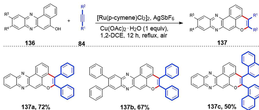
Scheme 80. Ru-Catalyzed Regioselective C–H/O–H Oxidative Annulation Reaction to Synthesis of Isochromeno[8,1-ab]Phenazines
