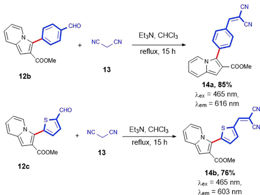
Scheme 9. The Synthesis of Fluorescent Materials 14a and 14b
