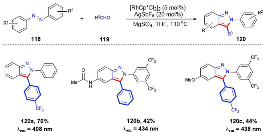
Scheme 66. Rhodium(III)-Catalyzed C–H Bond Addition of Azobenzenes to Aldehydes
