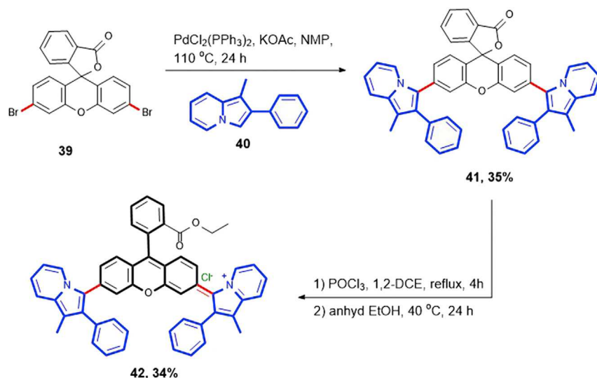
Scheme 23. Synthesis of Fluorescent Molecule 42 from 39
