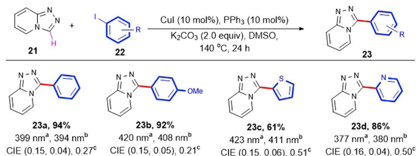
Scheme 13. Cu-Catalyzed Direct C–H (Hetero)arylation of [1,2,4]Triazolo[4,3-a]Pyridine
