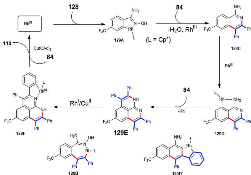
Scheme 76. The Proposed Mechanism for the Formation of 129
