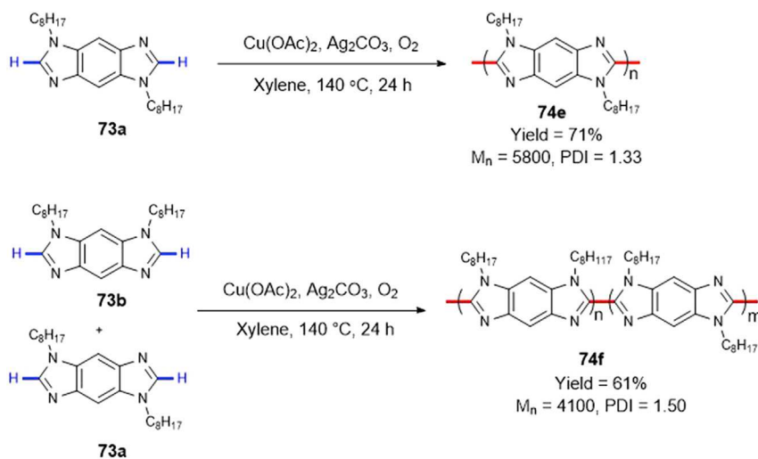
Scheme 43. Cu-Catalyzed Oxidative C–H/C–H Polymerization of 73a and 73b
