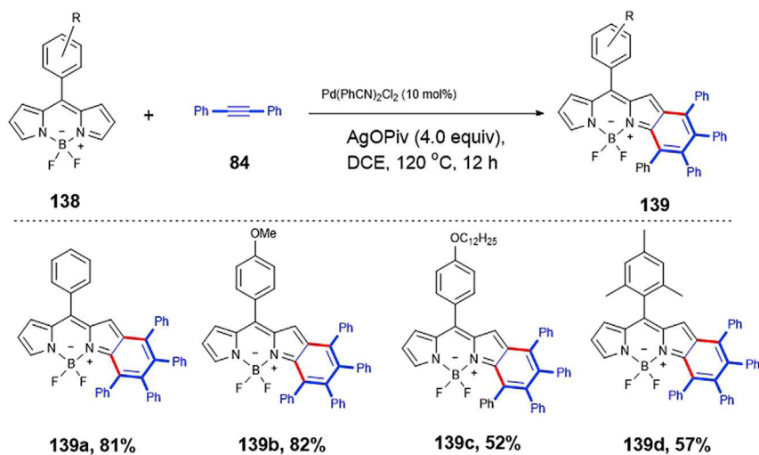
Scheme 82. Palladium-Catalyzed Direct C–H Functionalization or Annulation of BODIPYs with Alkynes
