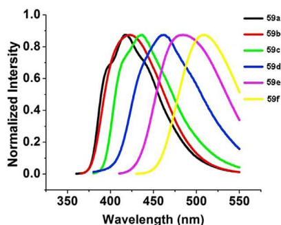
Figure 12. Normalized Emission Spectra of 59a–59f in \text{CH}_2\text{Cl}_2 Adapted from Huang et al. 44 with permission, copyright 2012 Royal Society of Chemistry.
