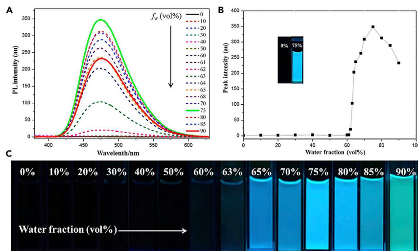
Figure 24. Photophysical Property of 85d
