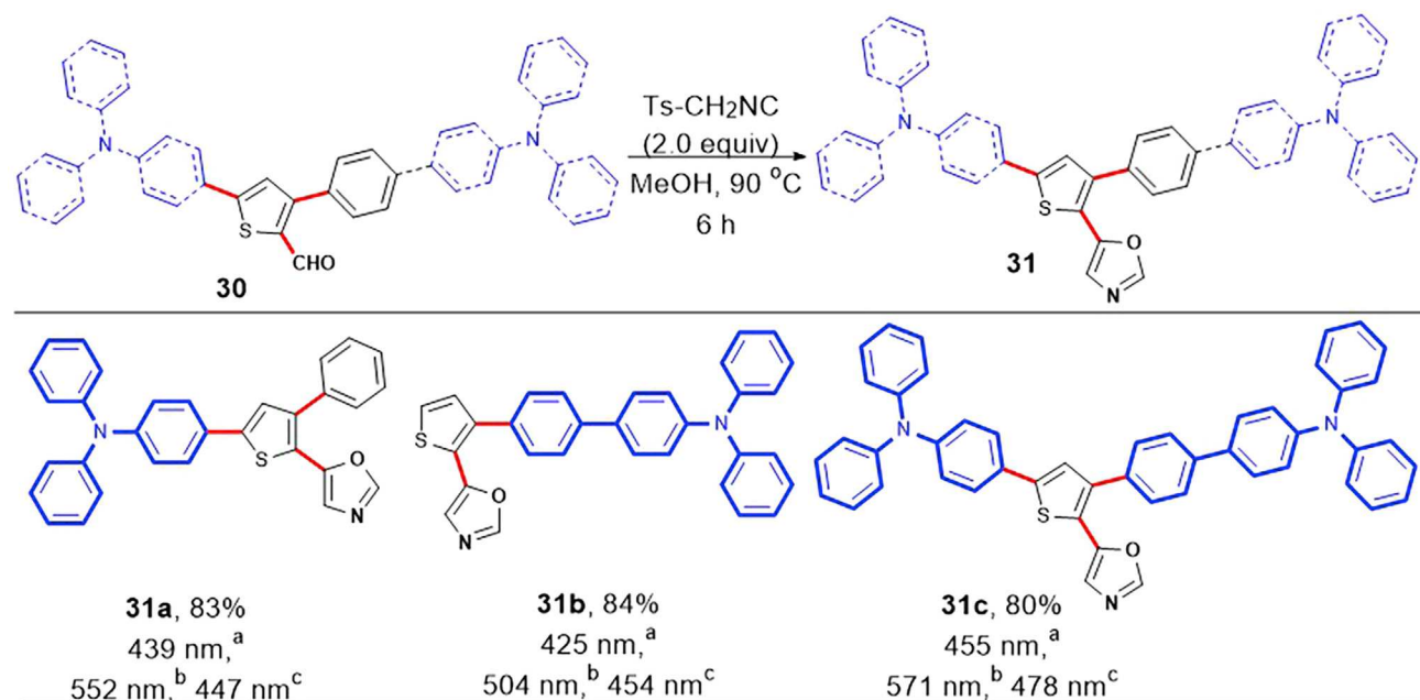
Scheme 19. Synthesis of TPA-Containing 3-Phenyl-(2-Oxazole)Thiophenes
