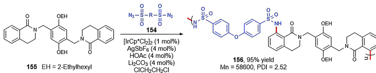
Scheme 90. Synthesis of the Polysulfonamide 156
