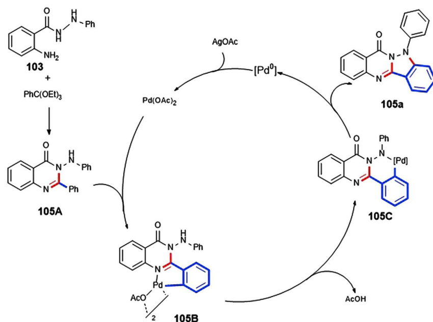
Scheme 57. The Plausible Mechanism for the Formation of Indazolo[3,2-b]Quinazolinones
