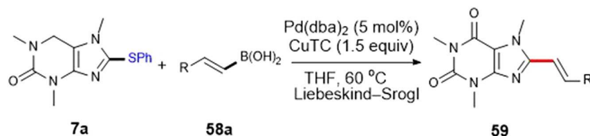
Scheme 29. The Conventional Synthetic Method for 59
