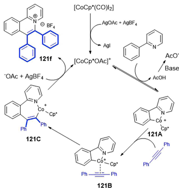
Scheme 70. A Plausible Reaction Mechanism for the Formation of 121
