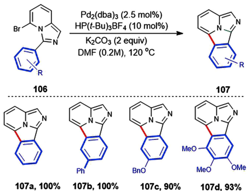
Scheme 58. Synthesis of Benzo[a]imidazo[2,1,5-c,d]indolizines
