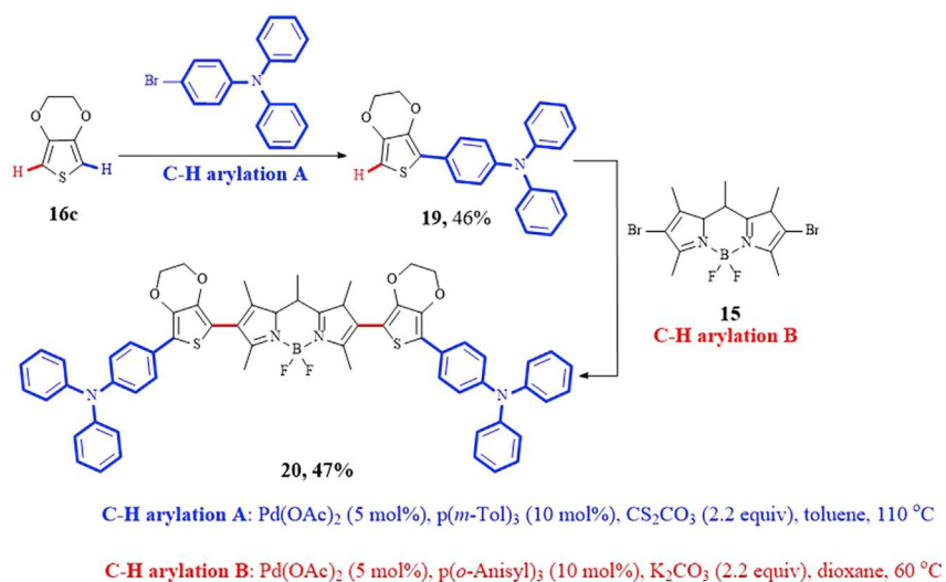
Scheme 12. Synthesis of BODIPY-Based \pi -Conjugated Functional Molecule 20 through Sequential C–H Arylations
