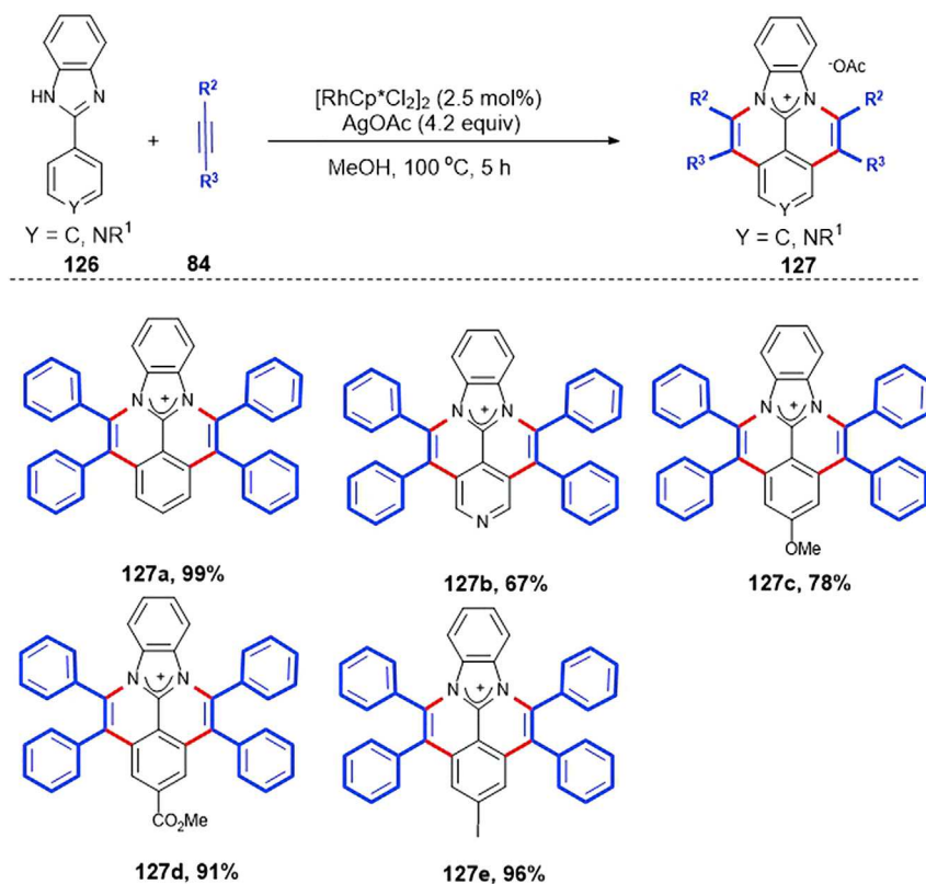
Scheme 74. Synthesis of Fluorophore Dyes 127a–127e via Rh III -Catalyzed Annulation of Pyridine Backbones
