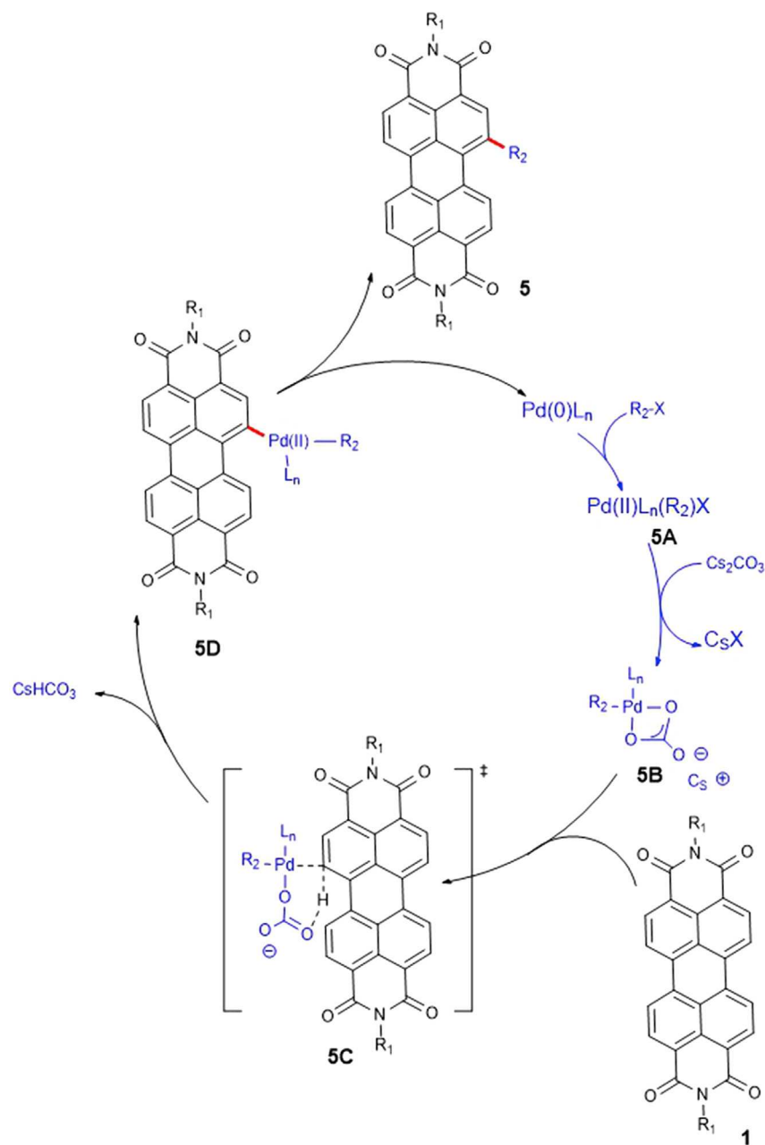
Scheme 4. The Plausible Reaction Mechanism for the Formation of 5
