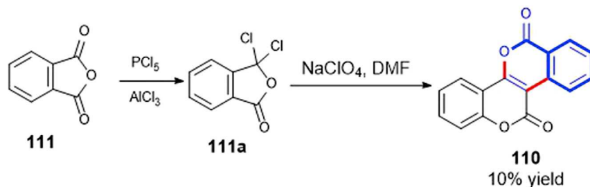
Scheme 61. The Conventional Synthetic Method for 110
