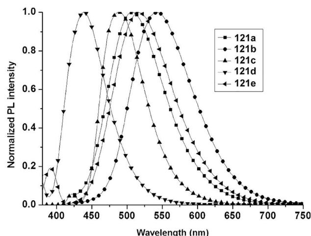
Figure 32. Photoluminescence Spectra of Selected Cinnolinium Salts (121a–121e) in DCM
