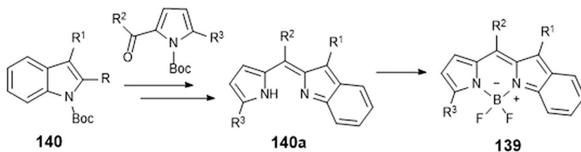
Scheme 83. The Conventional Synthetic Method for 139
