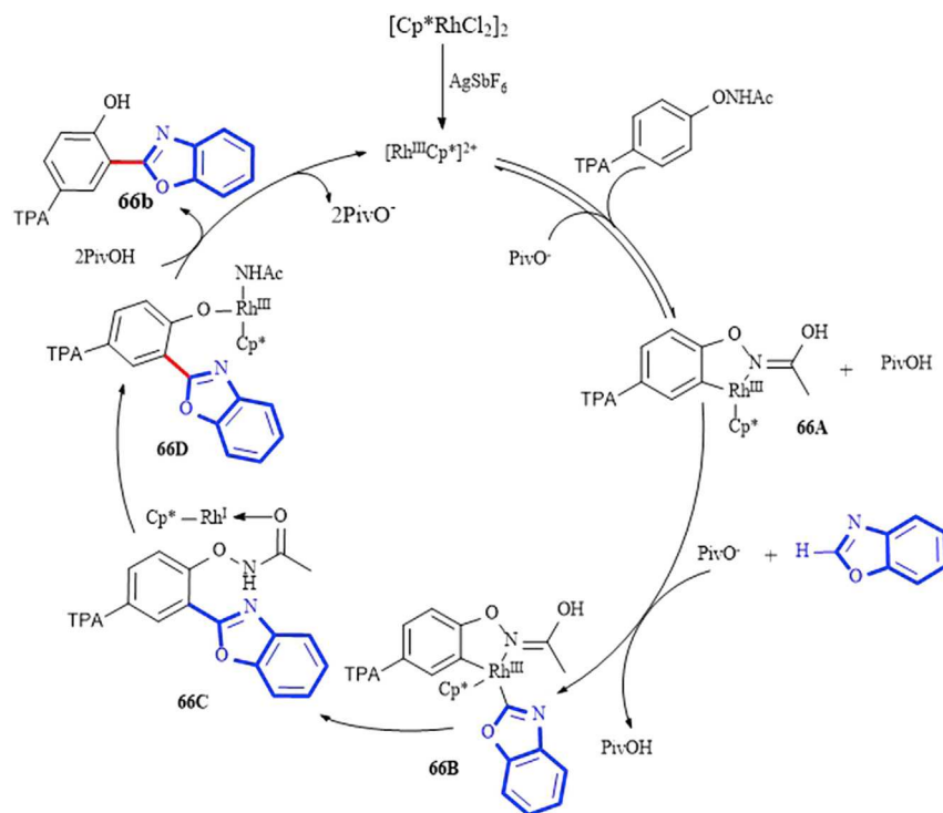
Scheme 35. The Tentative Mechanism for the Cross-Coupling of N -aryloxyacetamide with 1,3-Azole
