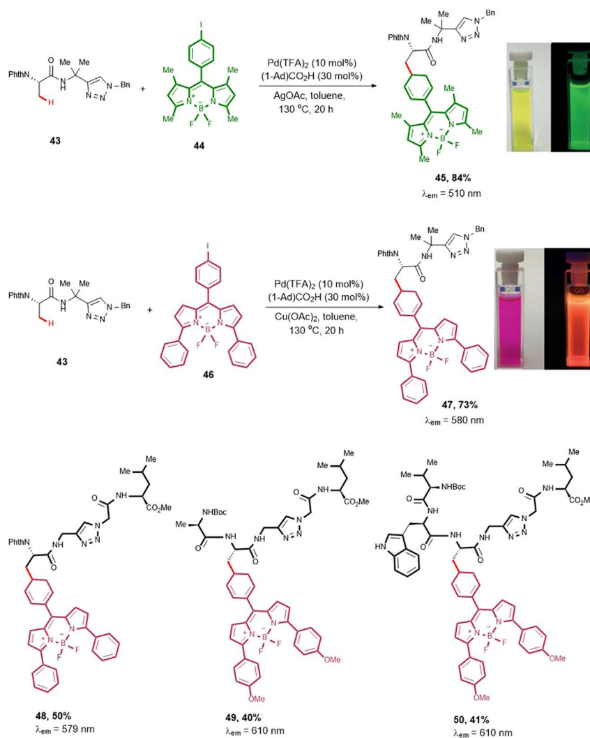
Scheme 24. Palladium-Catalyzed C(sp 3 )-H Activation in Building Novel Peptidomimetic BODIPY Sensors
