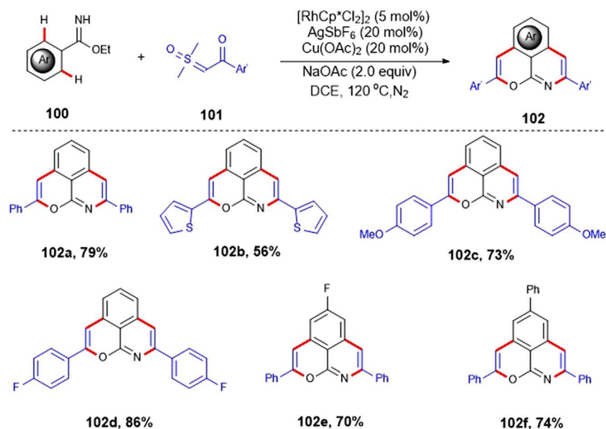
Scheme 55. Rhodium-Catalyzed Annulation between Ethyl Benzimidates and \alpha -Aroyl Sulfur Ylides
