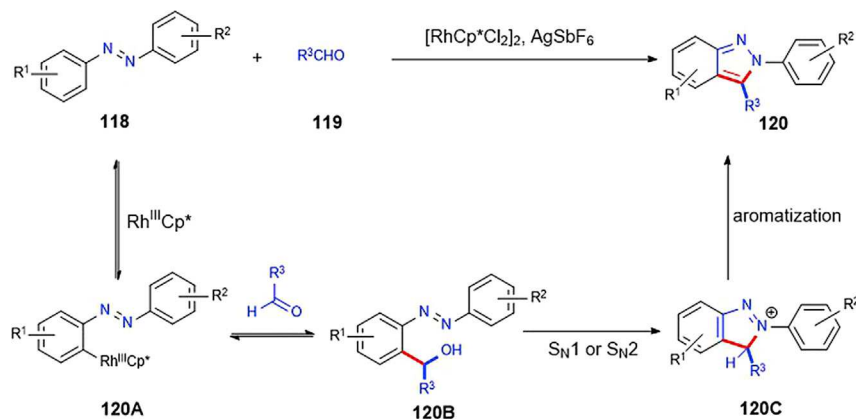
Scheme 68. A Plausible Mechanism for the Formation of 120
