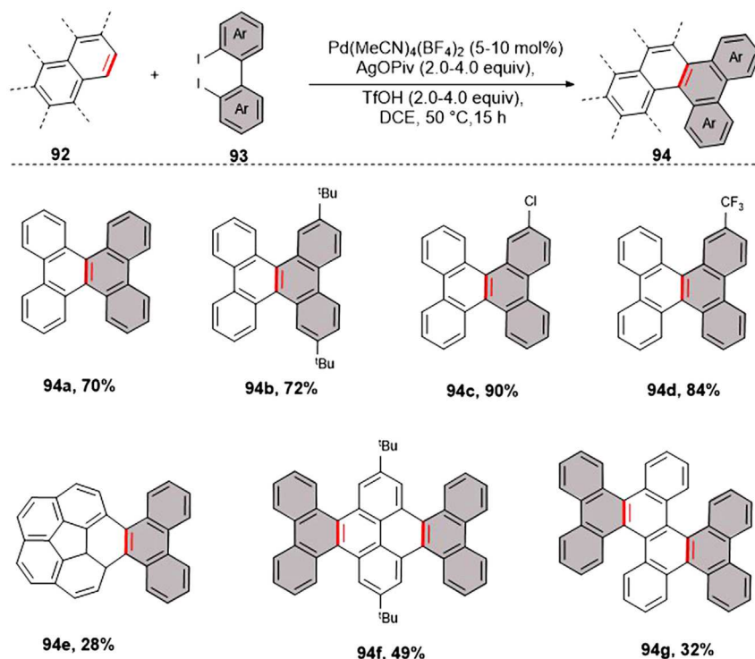
Scheme 52. The Palladium-Catalyzed Annulative \pi -Extension Reaction
