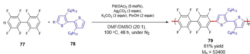
Scheme 45. Pd-Catalyzed Cross-Dehydrogenative Polycondensation
