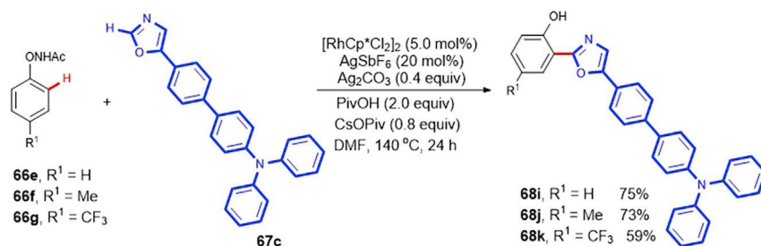
Scheme 38. Synthetic Routes of 68i–68k
