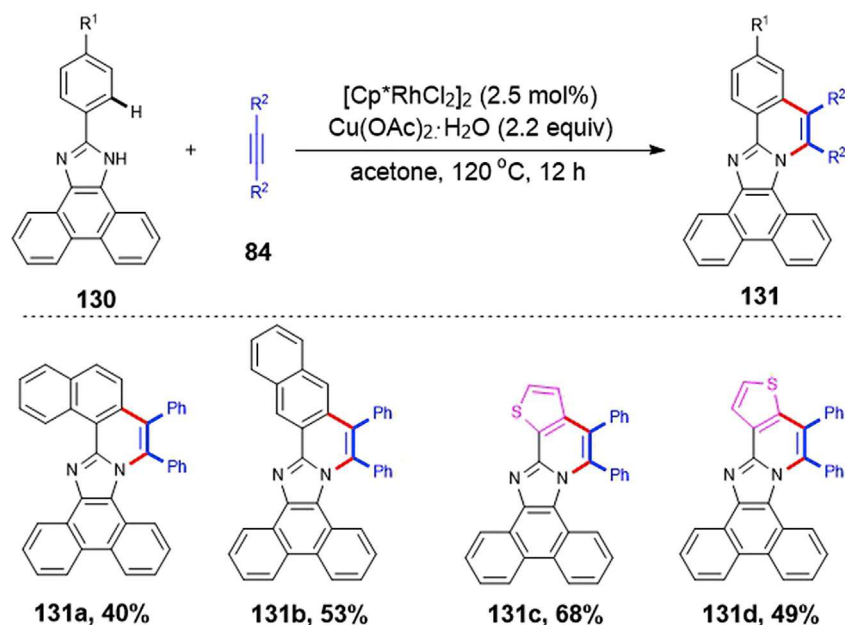
Scheme 77. Rhodium(III)-Catalyzed C–H Activation and Alkyne Annulation
