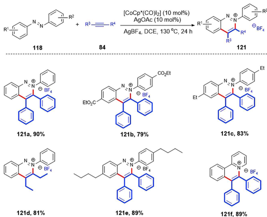
Scheme 69. Synthesis of Cinnolinium Salts 121a–121f
