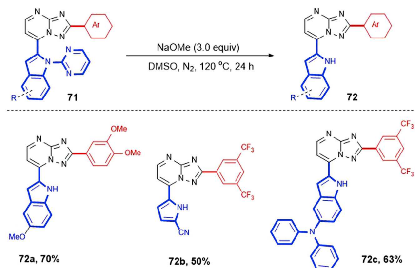
Scheme 41. Removal of the Pyrimidyl Directing Group
