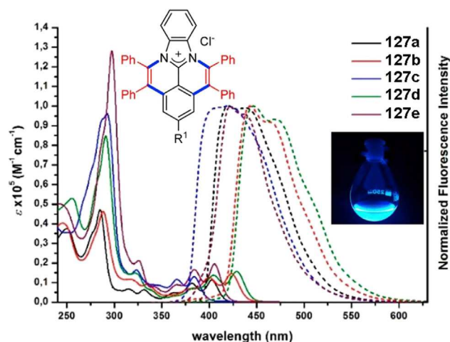
Figure 33. Photoluminescence Spectra of 127a–127e in DCM
