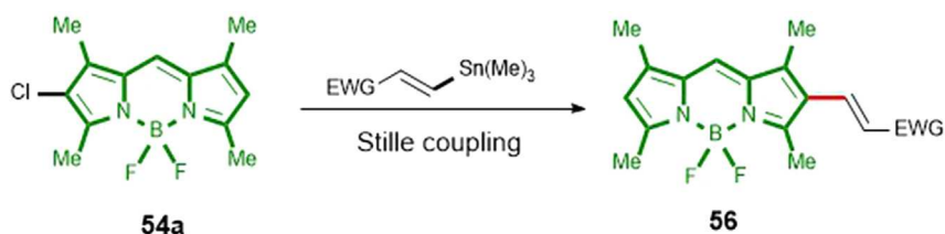
Scheme 27. The Conventional Synthetic Method for 56
