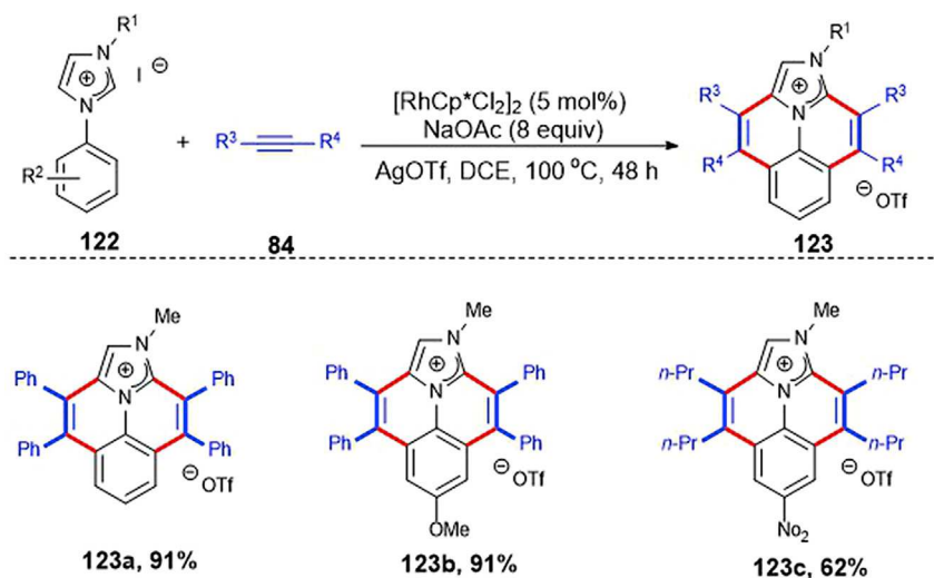
Scheme 71. Rhodium(III)-Catalyzed C–H Activation-Annulation
