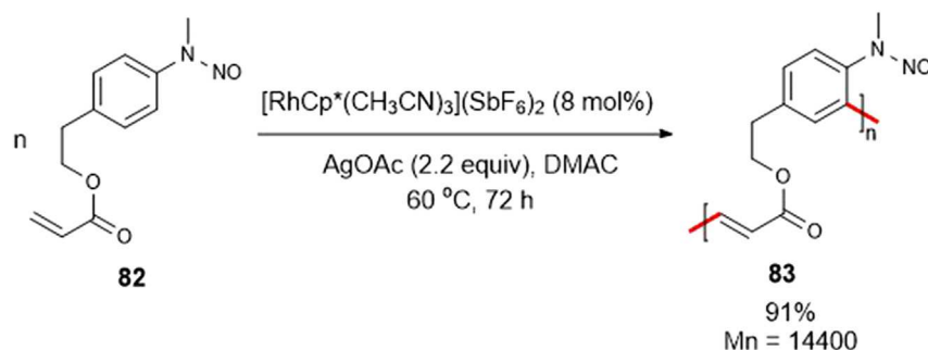
Scheme 47. Synthesis of Poly 83
