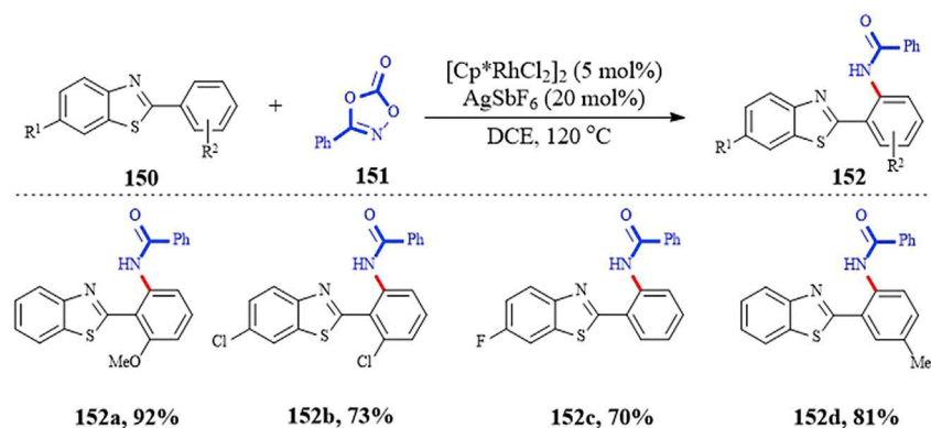
Scheme 88. Rhodium(III)-Catalyzed Direct C–H Amidation of 2-Arylbenzo[d]thiazoles
