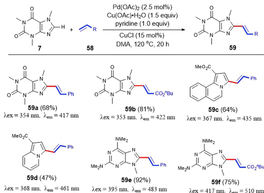
Scheme 28. Palladium-Catalyzed Dehydrogenative Heck Coupling between Various Biologically Relevant N -Heteroarenes and Alkenes
