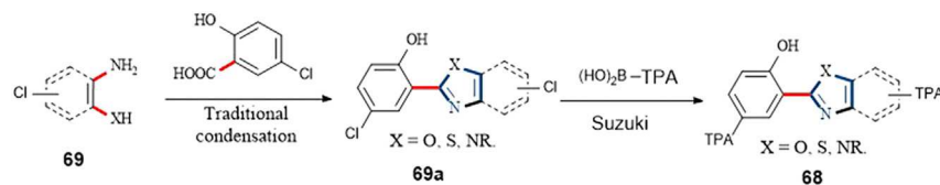
Scheme 36. The Conventional Synthetic Method for 68
