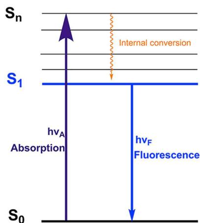
Figure 1. Schemes of Excited-State Relaxation
