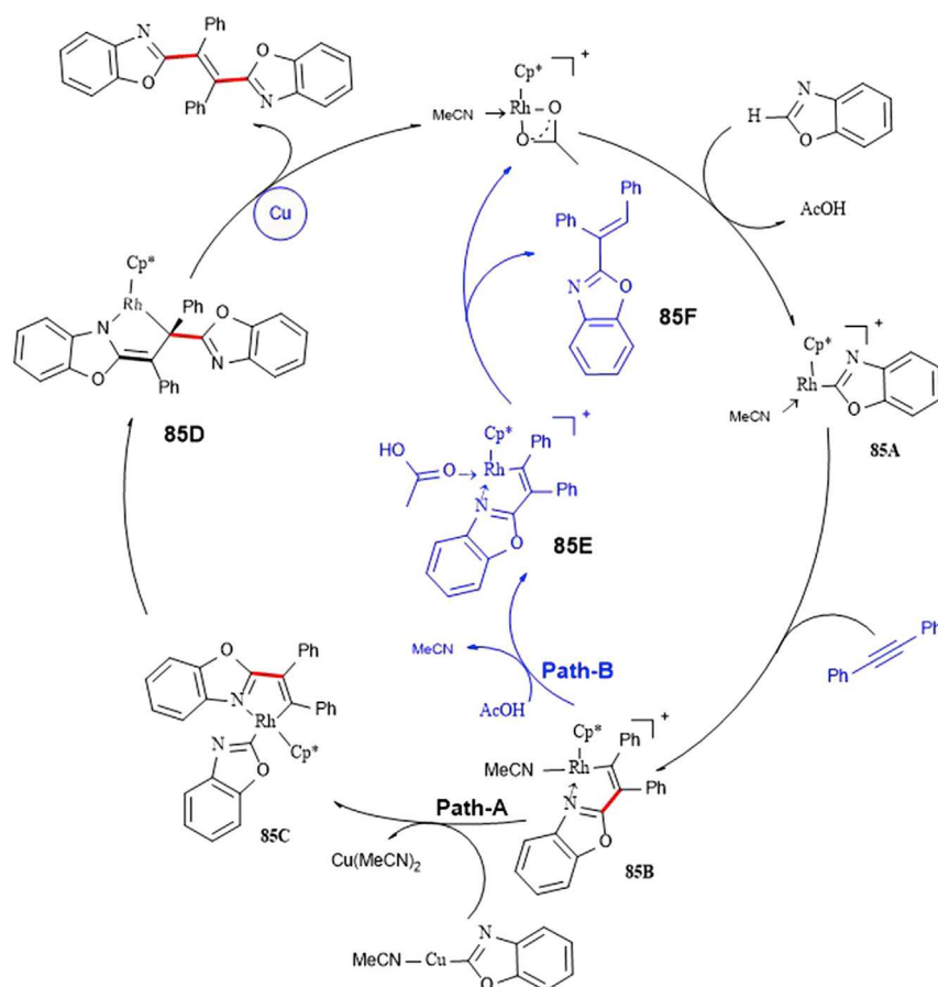
Scheme 49. Proposed Mechanism of Rhodium-Catalyzed Trans-selective C–H Addition/Oxidative Coupling
