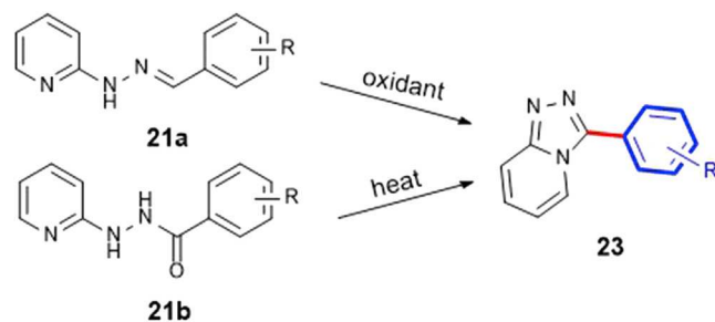
Scheme 14. The Conventional Synthetic Method for 23
