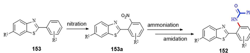
Scheme 89. The Conventional Synthetic Method for 152
