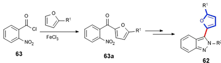
Scheme 31. The Conventional Synthetic Method for 62
