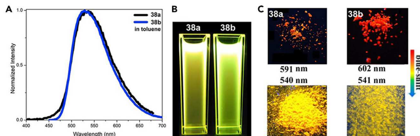
Figure 10. Fluorescence Emission Spectra and Fluorescent Images of 38a and 38b
