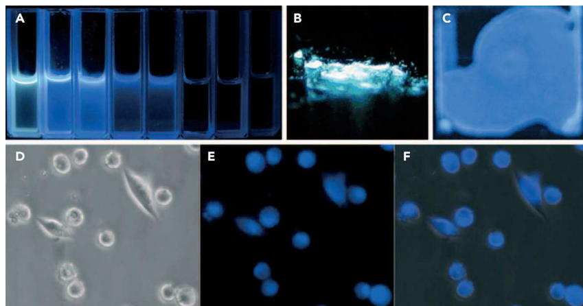
Figure 2. Photophysical Property of 9a–9f
