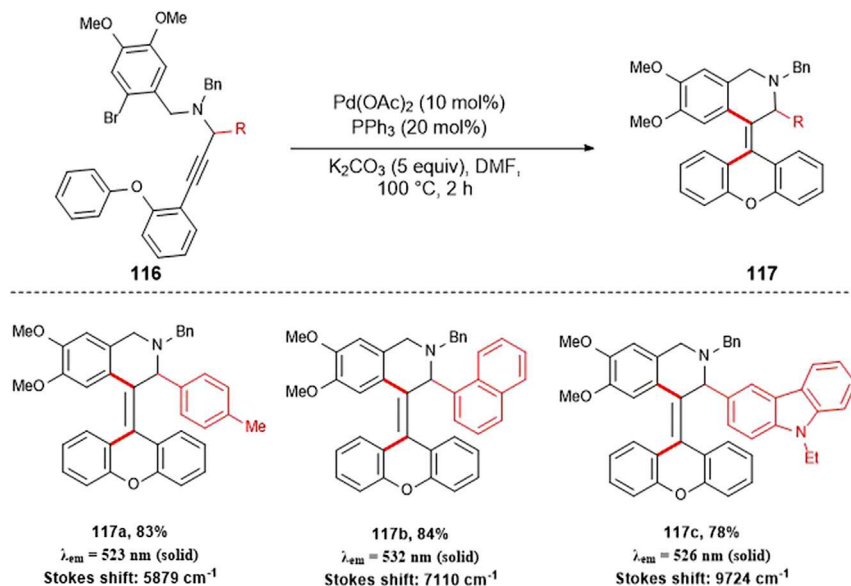
Scheme 64. Palladium-Catalyzed Cyclization/C–H Activation of 2-Bromobenzyl- N -Propargylamine Derivatives
