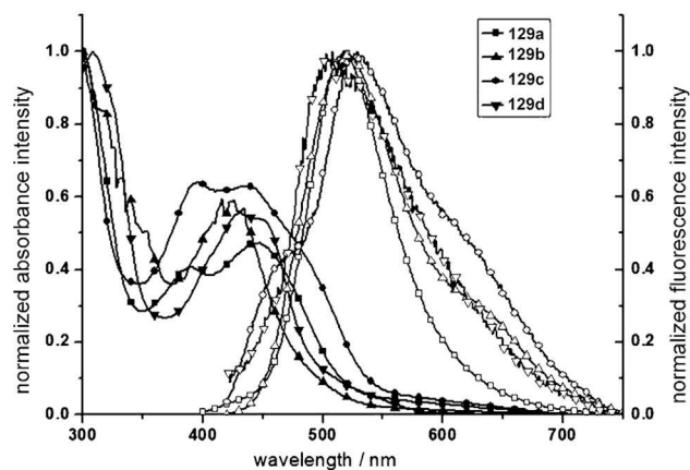
Figure 34. Absorption and Fluorescence Spectra of 129a–129d in Dichloromethane
