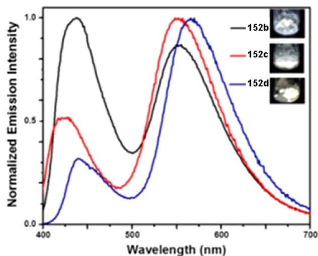
Figure 37. Normalized Emission Spectra of 152b-152d in the Solid State
