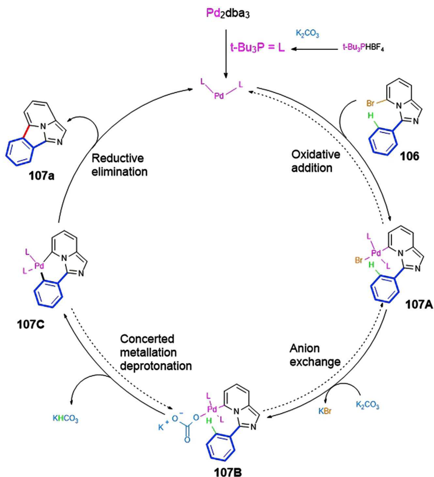
Scheme 59. The Plausible Mechanism for the Intramolecular C–H Arylation of 106
