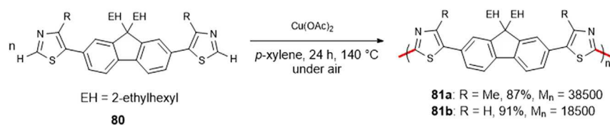
Scheme 46. Cu-Catalyzed Polycondensation Reactions
