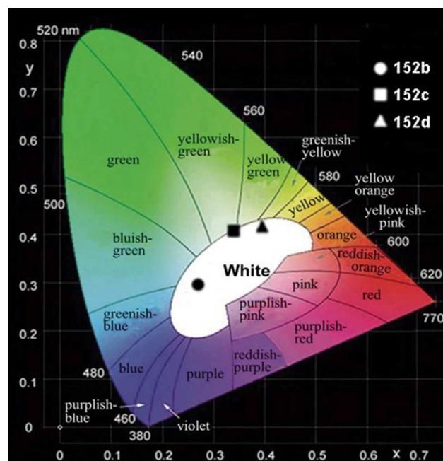
Figure 38. The Emission Color Coordinate of 152b-152d in the CIE 1,931 Chromaticity Diagram
