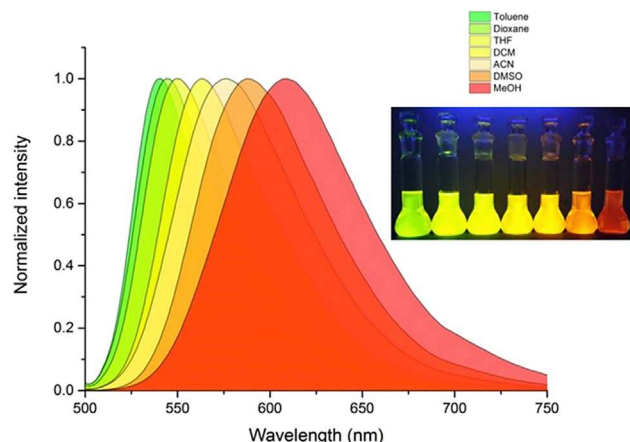
Figure 36. Emission spectra of 137b in Various Solvents
