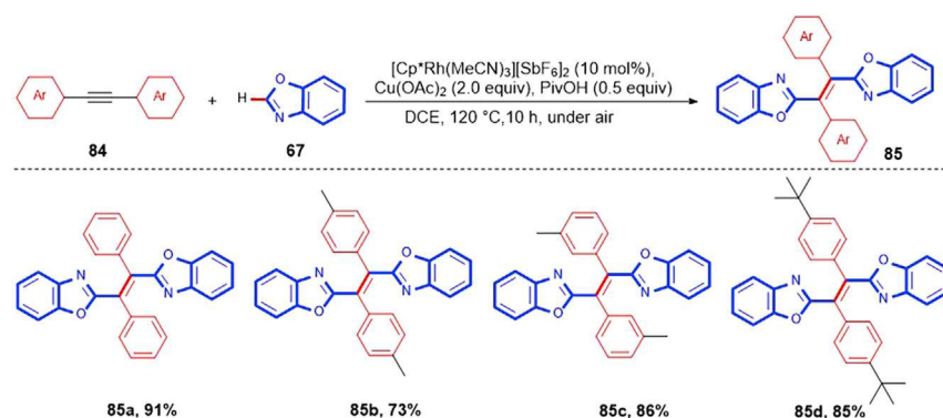
Scheme 48. Rhodium-Catalyzed C–H Addition/Oxidative Coupling of Alkynes with Azoles
