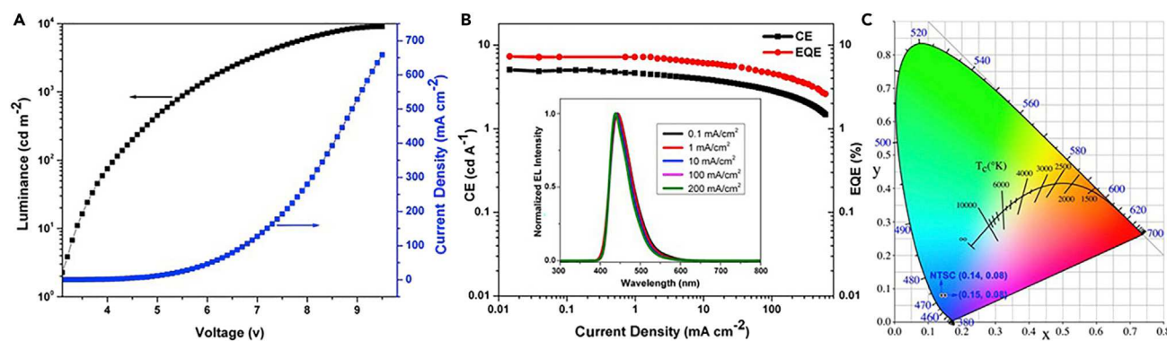
Figure 19. Electroluminescence Property of 68i
