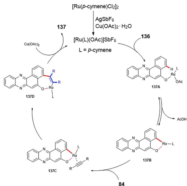
Scheme 81. A Plausible Mechanism for the Formation of 137
