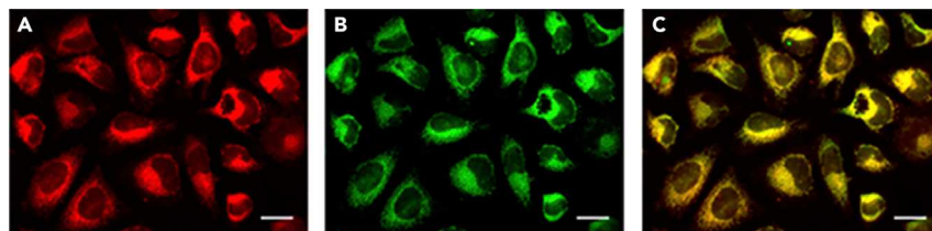
Figure 4. The Fluorescence Bioimaging of Probe 18
