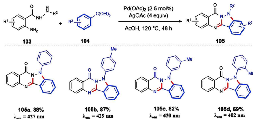
Scheme 56. The Palladium-Catalyzed Cyclization/C–H Activation Cascade Reaction
