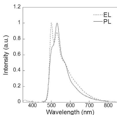
Figure 23. The Photoluminescence Spectrum of a Thin Film of 81b and the Electroluminescent Spectrum of an OLED with 81b at 7 V
