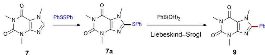
Scheme 5. The Conventional Synthetic Method for 9
