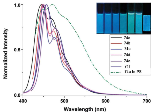
Figure 21. Fluorescence Spectra of Polymers 74a–74f in CHCl 3 and 74a in the PS Film
