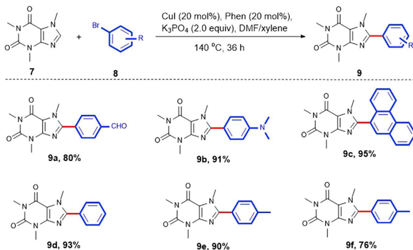
Scheme 6. Copper-Catalyzed Direct C–H/C–Br Cross-Coupling Xanthine with Aryl Bromides
