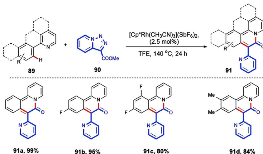
Scheme 51. Rh III -Catalyzed C–H Bond Activation/Annulation
