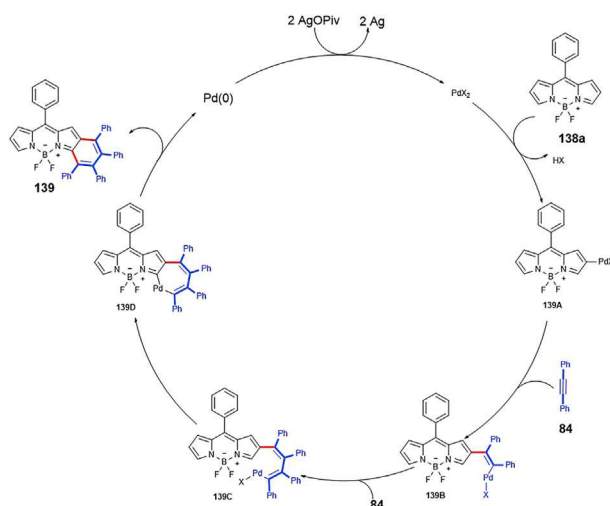
Scheme 84. The Plausible Mechanism for the Formation of 139
