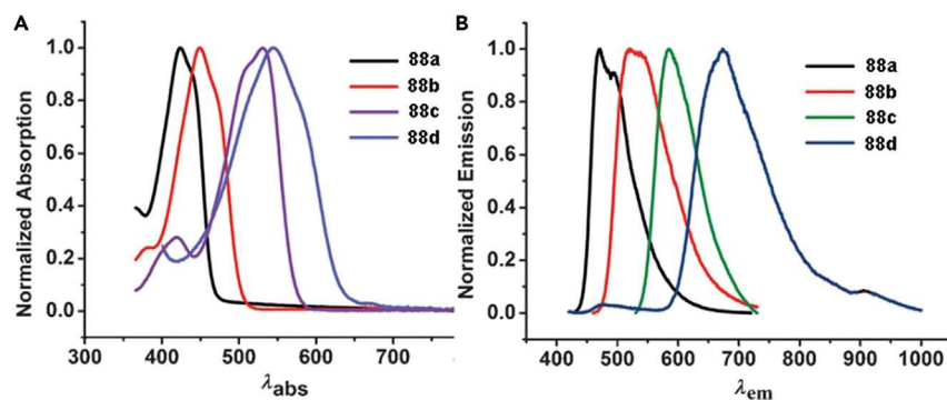
Figure 25. Absorption and Emission Spectra of 88a–88d
