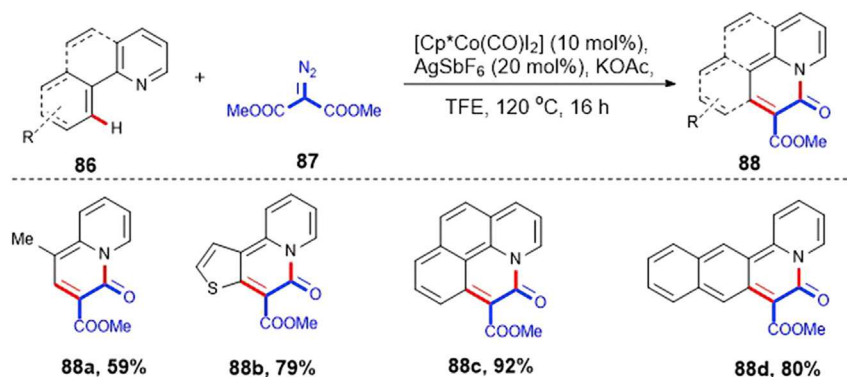
Scheme 50. Cobalt(III)-Catalyzed Coupling of Diazo Compounds with Heteroaromatic Compounds via C–H Activation/Annulation
