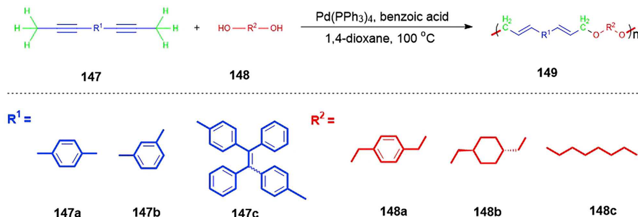
Scheme 87. Palladium/Benzoic Acid-Catalyzed Polymerization of Internal Diynes and Diols
