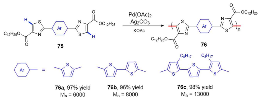
Scheme 44. Synthesis of Polymers 76a–76c through Pd-Catalyzed Oxidative C–H/C–H Coupling
