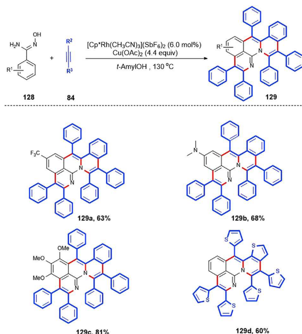
Scheme 75. Synthesis of Fluorophore Dyes 129a–129d via Rhodium-Catalyzed C–H Bond Activation of N -hydroxybenzamides and Alkynes
