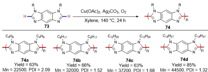
Scheme 42. Cu-Catalyzed Oxidative C–H/C–H Polymerization of 73
