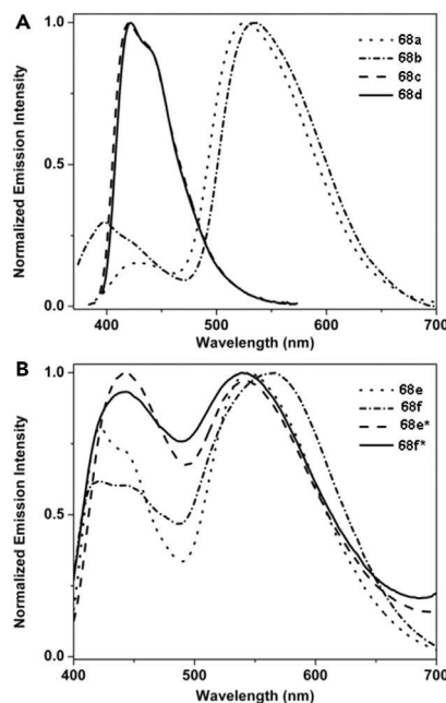
Figure 15. Emission spectra of 68a–68f in Toluene and PS Films
