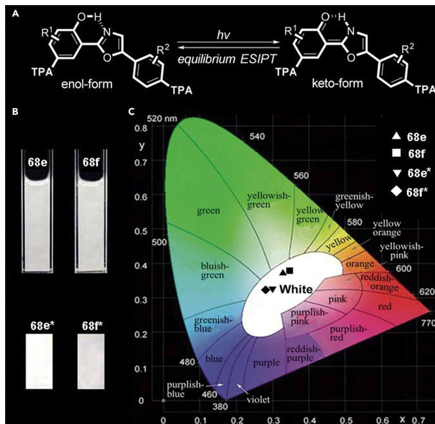
Figure 16. Emission Color Coordinates and Fluorescence Images of 68e and 68f in Toluene and in PS Films
