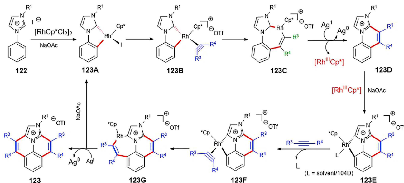
Scheme 72. The Plausible Catalytic Cycle for the Formation of 123
