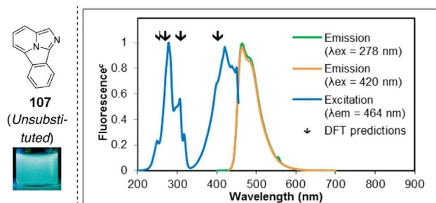
Figure 29. The Emission and Excitation Spectra of 107a
