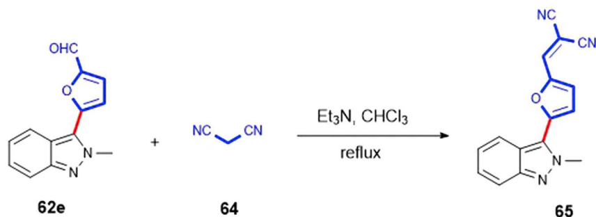
Scheme 32. Synthesis of Near-Infrared Fluorophore Dye 65
