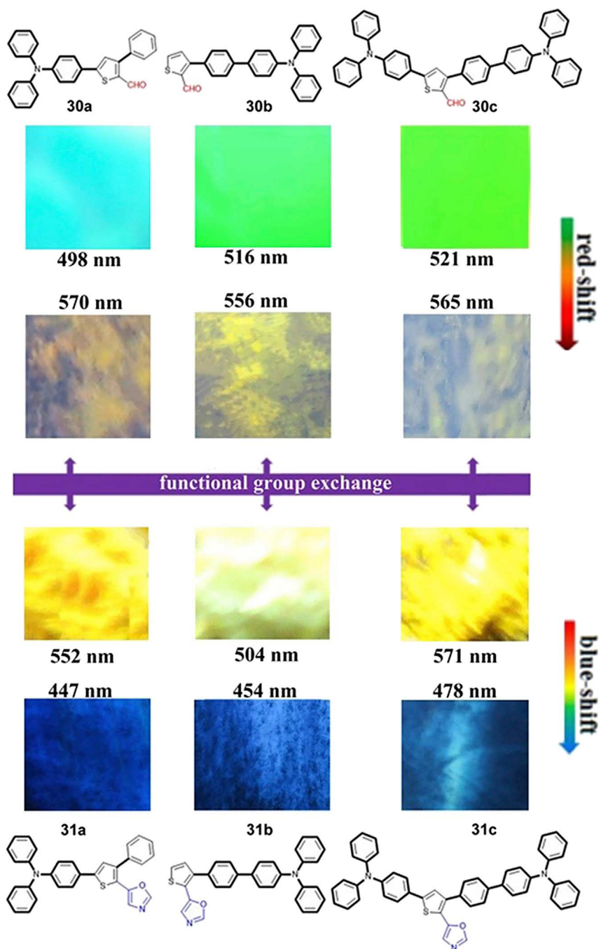
Figure 7. Fluorescent Images of 30 and 31 before and after Grinding
