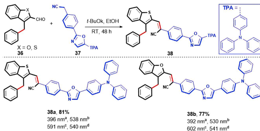
Scheme 22. Synthesis of TPA-Containing 2-(4-(Oxazol-2-yl)Phenyl)Acetonitrile-3-Benzylbenzothio/Fur-Anphens
