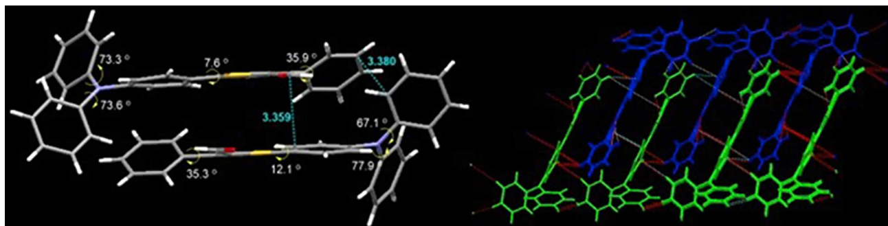
Figure 8. The Crystal Packing Structure of 30a
