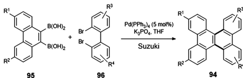
Scheme 53. The Conventional Synthetic Method for 94
