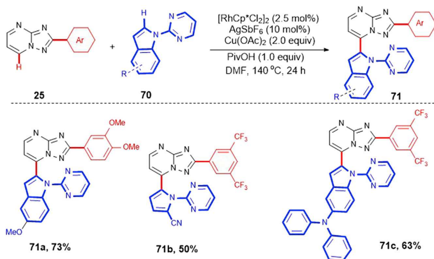
Scheme 40. Rh(III)-Catalyzed Oxidative C–H/C–H Cross-Coupling
