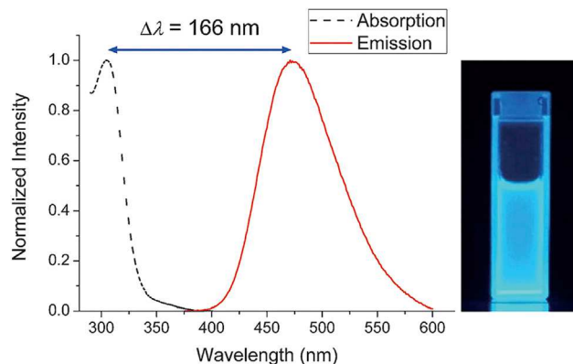
Figure 39. Absorption and Emission Spectra of 156 in THF Solution
