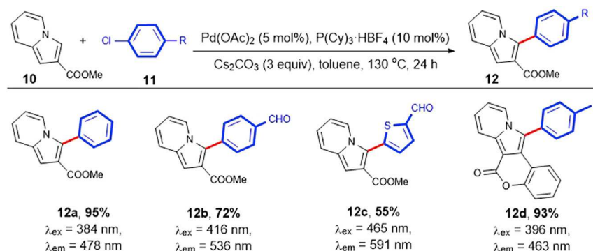
Scheme 7. Palladium-Catalyzed Direct C–H Bond (Hetero)Arylation of N -Heteroarenes with Aryl Chlorides
