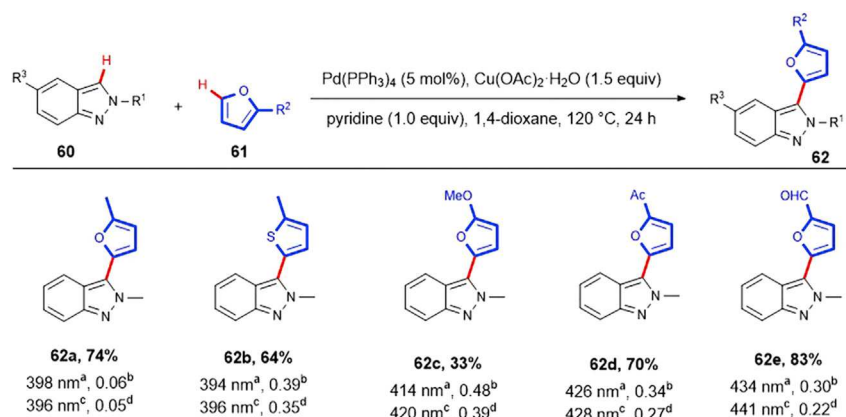
Scheme 30. Direct Oxidative C–H/C–H Cross-Coupling of 2H-Indazoles with Various Heteroarenes and Photophysical Data of the Resulting Catalytic Products
