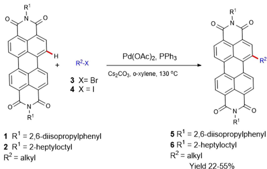
Scheme 2. Pd-Catalyzed Alkylation of PBIs with Alkyl Halides
