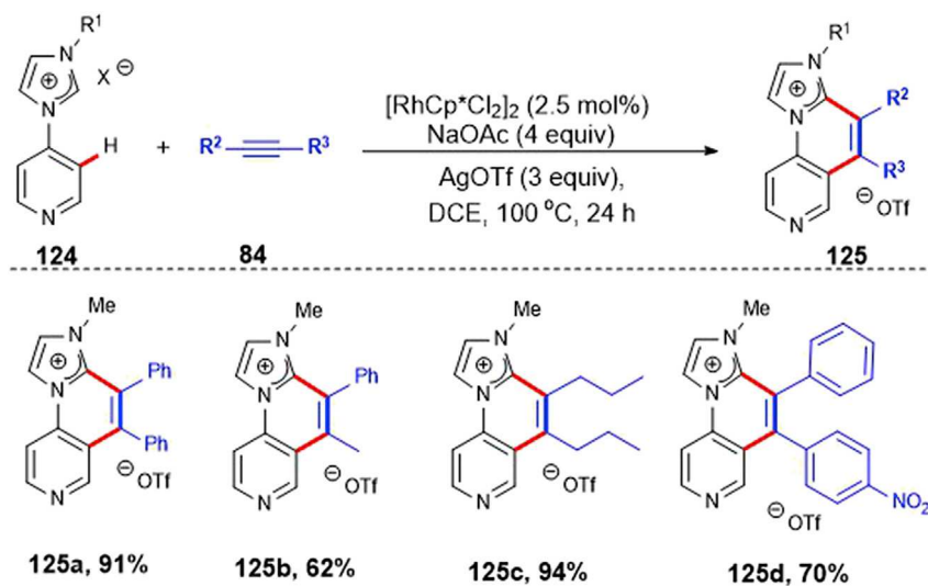
Scheme 73. Rh III -Catalyzed NHC-Directed Annulation of Pyridine Backbones
