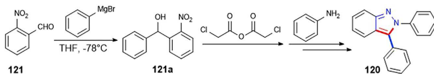
Scheme 67. The Conventional Synthetic Method for 120
