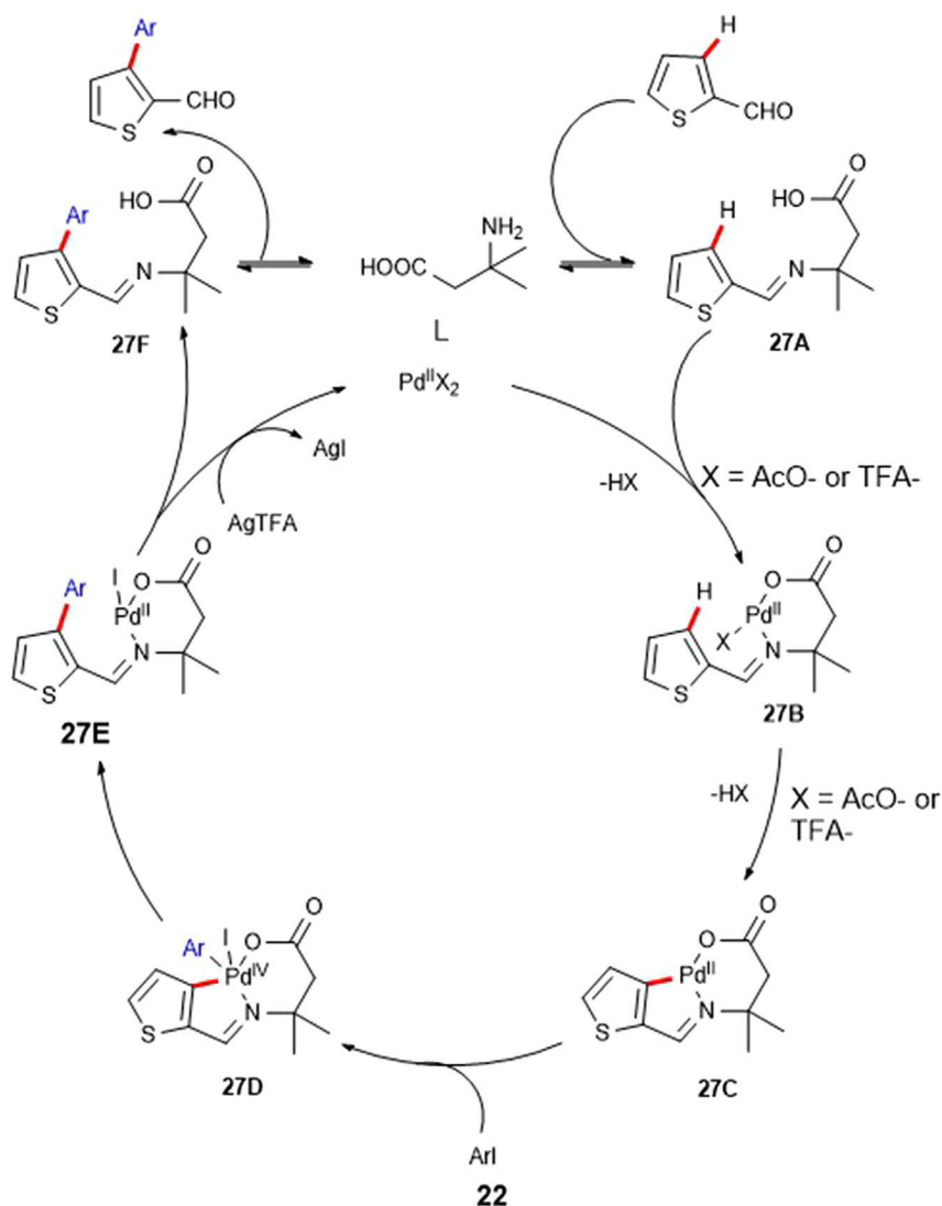
Scheme 17. The Plausible Mechanism for the Formation of 28
