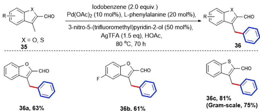
Scheme 21. Synthesis of 3-Benzylbenzothiofuran-2-Carbaldehyde and 3-Benzylbenzofuran-2-Carbaldehyde by Transient Ligand-Enabled Palladium Catalyzed C–H Functionalization
