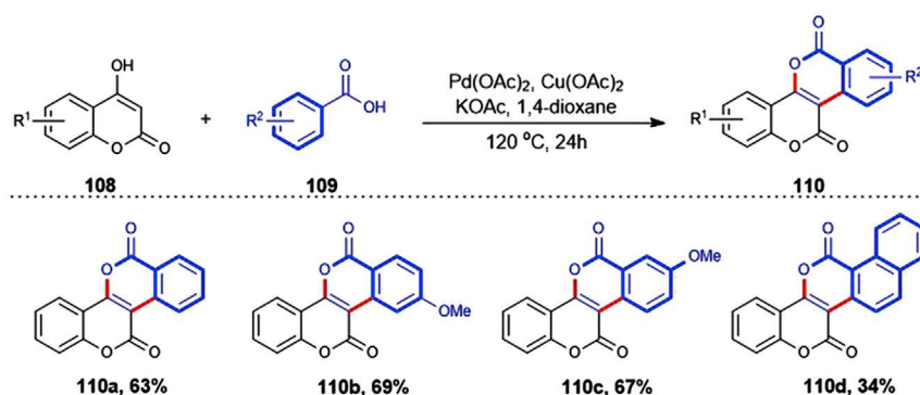
Scheme 60. Synthesis of 110
