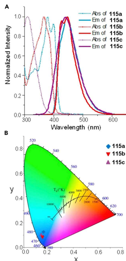
Figure 31. Photophysical Property of 115a–115c
