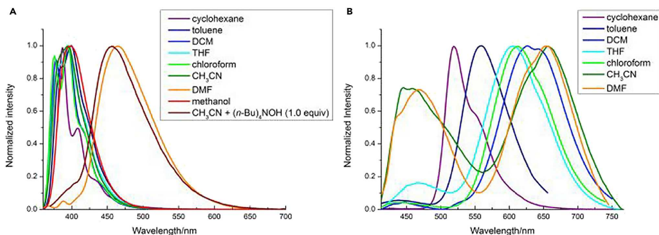
Figure 20. Normalized Emission Spectra of 71b and 71c
