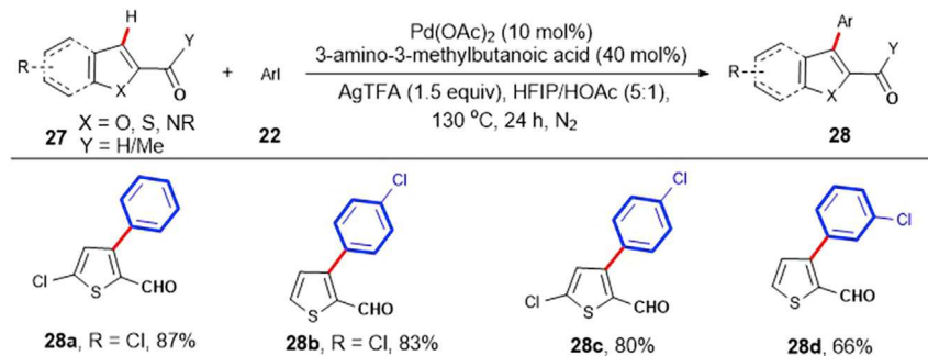
Scheme 16. Synthesis of 3-aryl-(2-Aldehyde)Thiophenes 28a–28d
