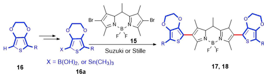
Scheme 10. The Conventional Synthetic Method for 17 and 18
