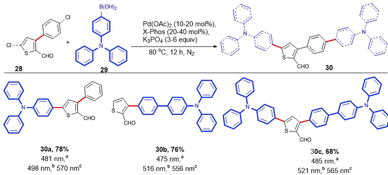
Scheme 18. Synthesis of TPA-Bearing 3-Phenyl-(2-Carbaldehyde)Thiophenes
