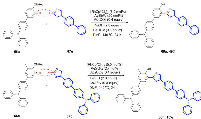
Scheme 37. Synthetic Routes of 68g and 68h
