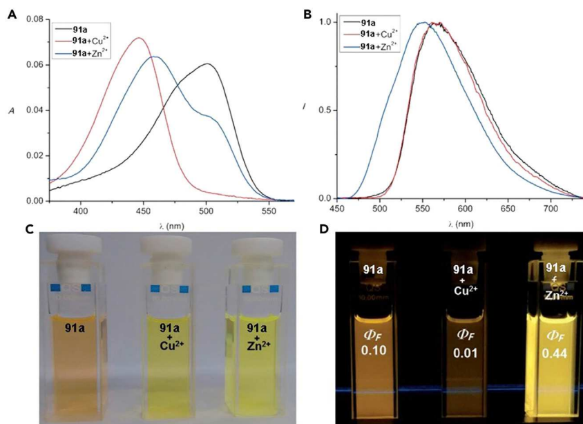
Figure 26. Photophysical Property and Photos of 91a
