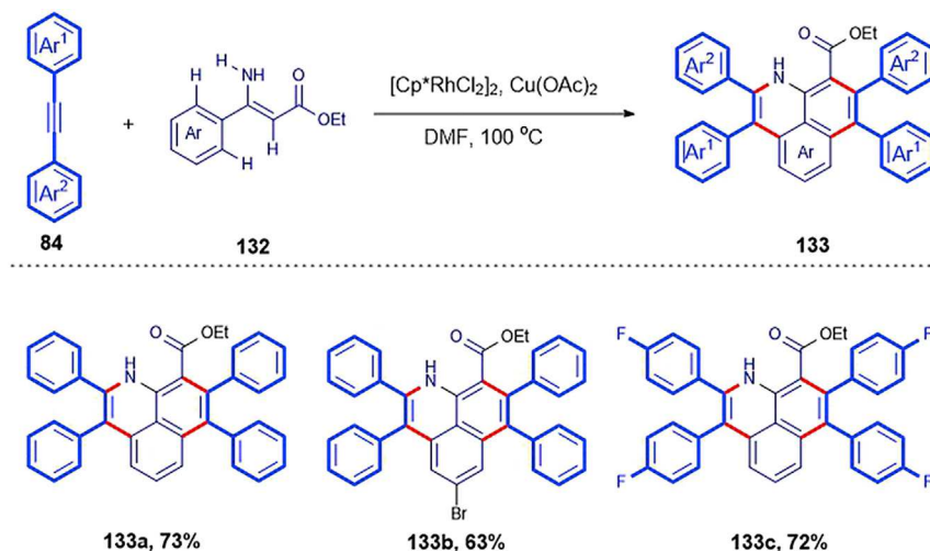
Scheme 78. Rh-Catalyzed Tandem Oxidative Annulation of \beta -Enamino Esters with Alkynes
