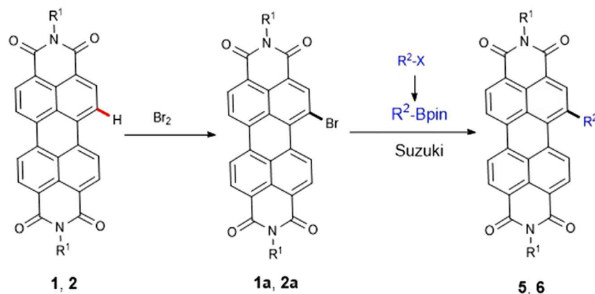
Scheme 3. The Conventional Synthetic Method for 5–6
