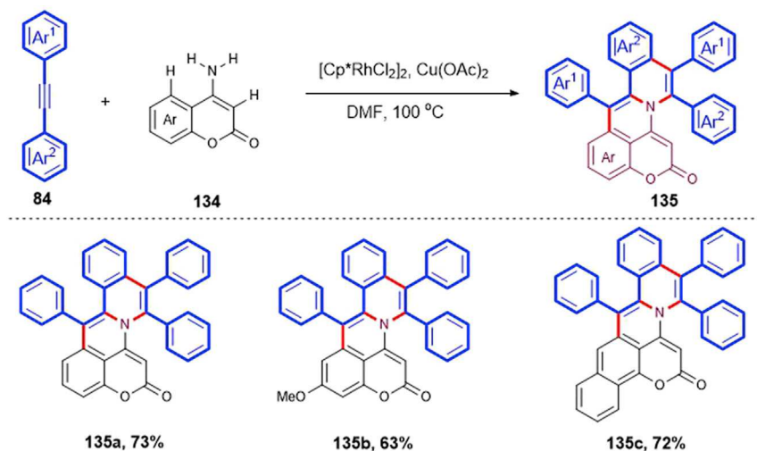
Scheme 79. Rh-Catalyzed Tandem Oxidative Annulation of 4-Aminocoumarins with Alkynes
