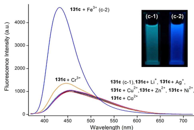
Figure 35. Fluorescence Emission Spectra of 131c in Acetone Solvent (50 \mu\text{M} ) with Different Metal Ions (50 \mu\text{M} )
