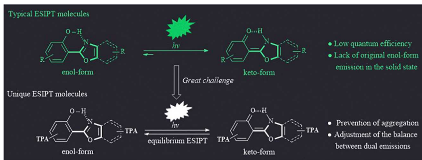
Scheme 33. Structures and ESIPT Mechanism of 2-(2-Hydroxyphenyl)azoles
