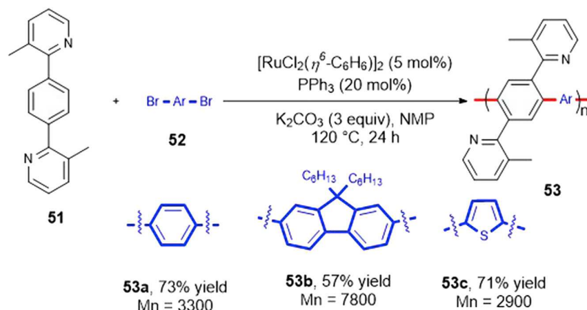
Scheme 25. Polycondensation of 51 and 52 .
