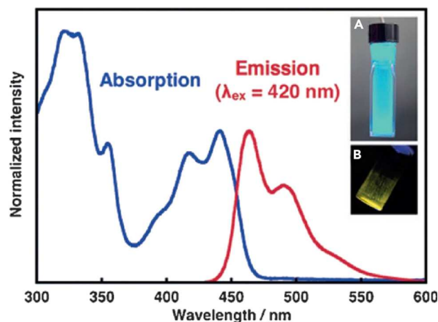
Figure 27. Normalized UV-Vis Absorption and Emission Spectra of 94g in CH 2 Cl 2
