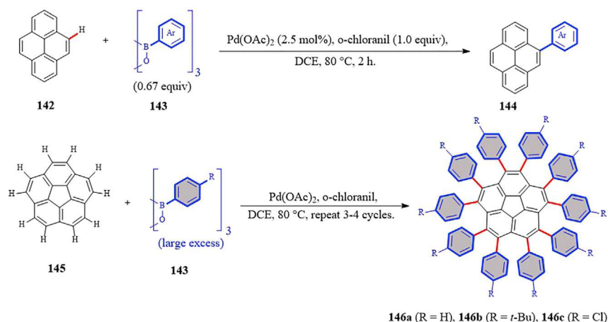
Scheme 86. Palladium-Catalyzed Direct C–H Functionalization to Synthesize Decaphenylcorannulenes
