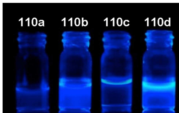
Figure 30. Photos of Compounds 110a–110d under UV Irradiation
