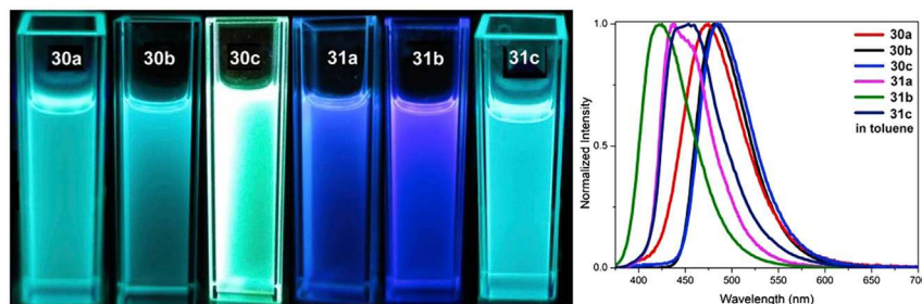
Figure 6. Fluorescence Images and Normalized Emission Spectra of 30a–30c and 31a–31c in Toluene ( 5.0 \times 10^{-5} M)
