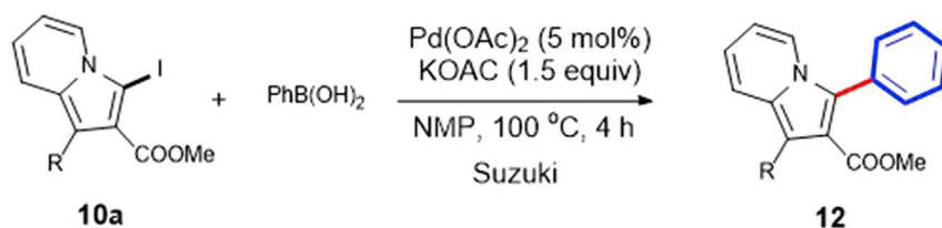
Scheme 8. The Conventional Synthetic Method for 12
