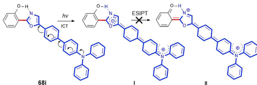
Scheme 39. The ICT and ESIPT Mechanism of 68i
