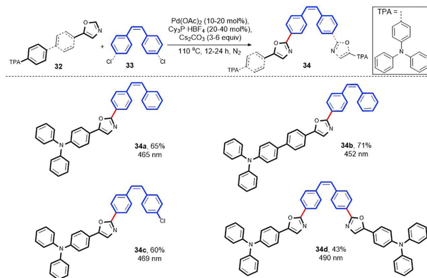
Scheme 20. Synthesis of TPA-Containing (z)-2-(4-Styrylphenyl)Oxazoles
