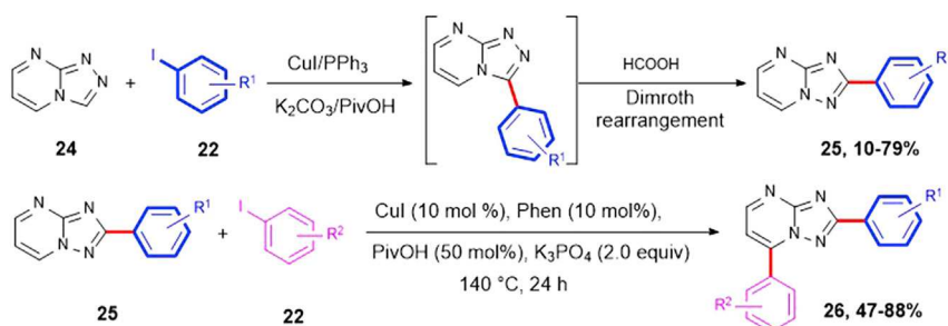
Scheme 15. Synthesis of 2,7-Diaryl-TAPs by a Programmed C–H/C–X Reaction
