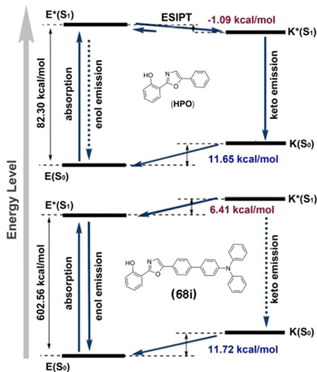
Figure 18. Diagrams of the ESIPT Processes and Calculated Energy Levels of HPO and 68i
