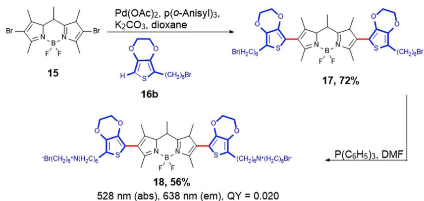
Scheme 11. Synthesis of the Bio-Imaging probe 18
