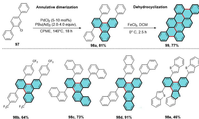
Scheme 54. Palladium-Catalyzed Annulative Dimerization of Aryl Halides
