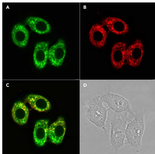
Figure 14. Co-staining of HepG2 Cells with 65 and a Commercially Available Mitochondria-Specific Tracker MTG (A–D) (A) fluorescent image of HepG2 cells stained with MTG ( \lambda_{\text{ex}} = 488 \text{ nm} , \lambda_{\text{em}} = 500\text{--}540 \text{ nm} ), (B) fluorescent image of HepG2 cells stained with 65 ( 20.0 \mu\text{M} , \lambda_{\text{ex}} = 552 \text{ nm} , \lambda_{\text{em}} = 650\text{--}750 \text{ nm} ), (C) merged image of (A and B), and (D) bright-field image. Adapted from Cheng et al. 45 with permission, copyright 2016 American Chemical Society.
