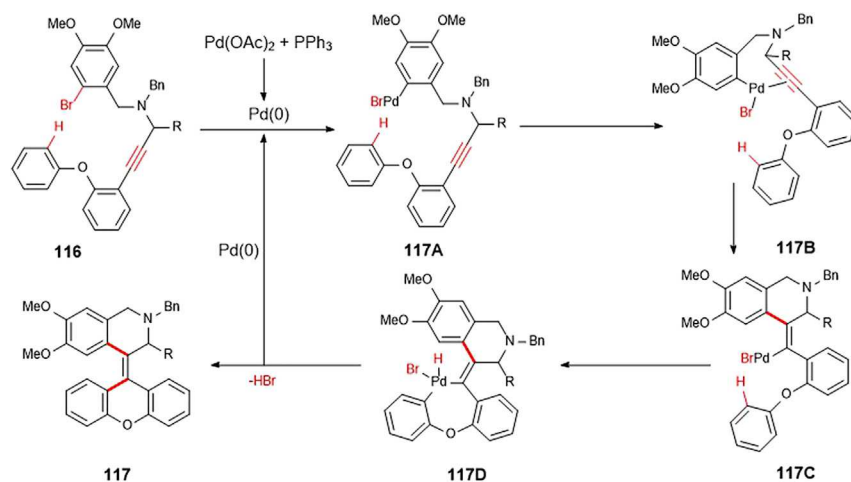
Scheme 65. The Plausible Mechanism for Formation of Tetrasubstituted Olefins
