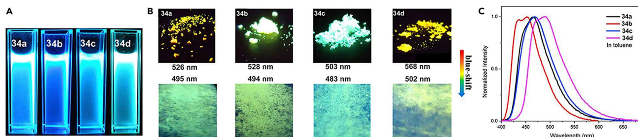
Figure 9. Fluorescence Images and Emission Spectra of 34a–34d
