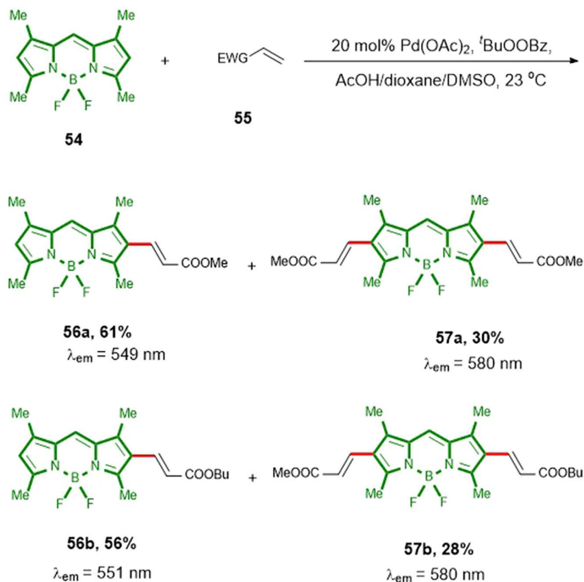
Scheme 26. Palladium-Mediated Heck-Type Cross-Coupling between 54 and Alkenes
