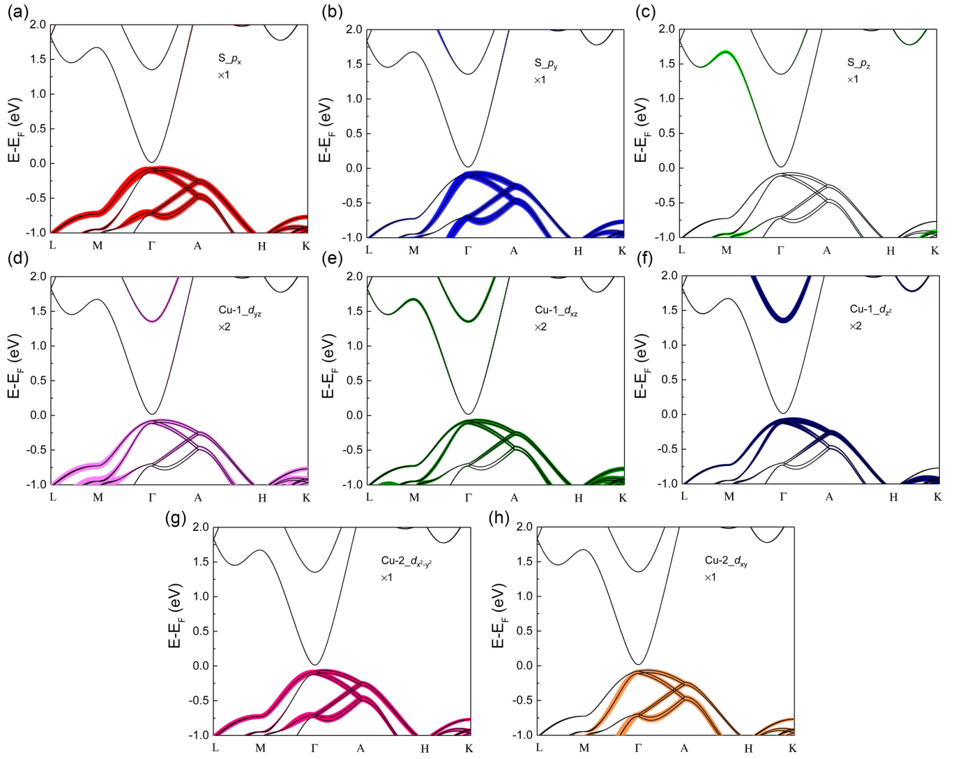
FIG. 12. Atomic and orbital projected band structures (a)–(h) of \text{NaCu}_5\text{S}_3 with P6_322 symmetry calculated at the DFT + U + SOC level.
