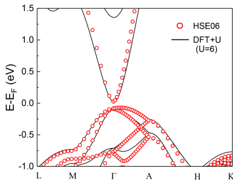
FIG. 9. Comparison of band structures of \text{NaCu}_5\text{S}_3 with P6_322 symmetry from HSE06 and DFT + U ( U = 6 eV), without SOC.
