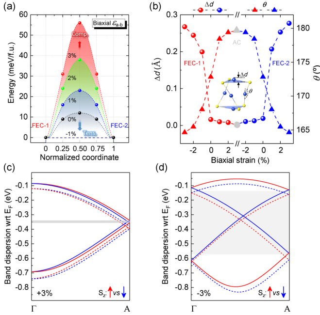
FIG. 17. Tunable ferri-chiral phase transition and spin splitting in NaCu 5 S 3 . (a) Transition barrier between the two ferri-chiral phases of NaCu 5 S 3 . The black dashed curve corresponds to the unstrained case, and other curves correspond to different strain values. (b) Detailed crystallographic information including the movement of Cu-2 away from the center of the CuS 3 planar triangle along [001] lattice direction ( \Delta d ), the movement of Cu-1 away from the center of the CuS 2 linear chain as represented by the S-Cu-S angle ( \theta ), and along the transition between FEC-1/2 and AC states under external biaxial strain in the ab plane. The \pm signs represent tensile and compressive strain. (c), (d) Low-energy valence bands in the \Gamma – A direction for the FEC-1 ferri-chiral phase of NaCu 5 S 3 under uniaxial strain along the c lattice direction. Red/blue colors indicate the spin projection, with the spin polarization axis along the z direction. The gray background indicates the magnitude of the spin-splitting energy. Similar tunability of spin-splitting energy under a/b/c uniaxial/biaxial strains is demonstrated in Fig. 18, in the Appendixes.
