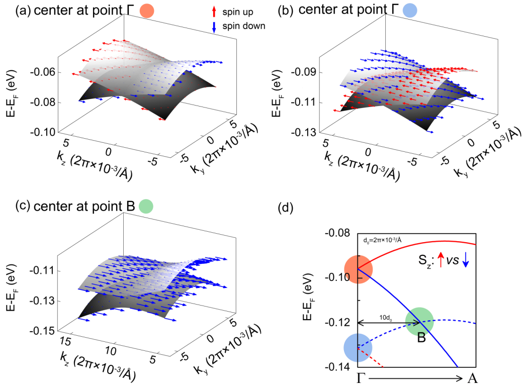
FIG. 15. Spin textures on the (k_y, k_z) plane ( k_x = 0 ) for the top valence bands of \text{NaCu}_5\text{S}_3 ( P6_322 ) at the DFT + U + SOC level. (a)–(c) Spin textures for different ranges of valence bands. (d) Zoom-in band structure showing the three chosen ranges of valence bands to illustrate the spin texture.
