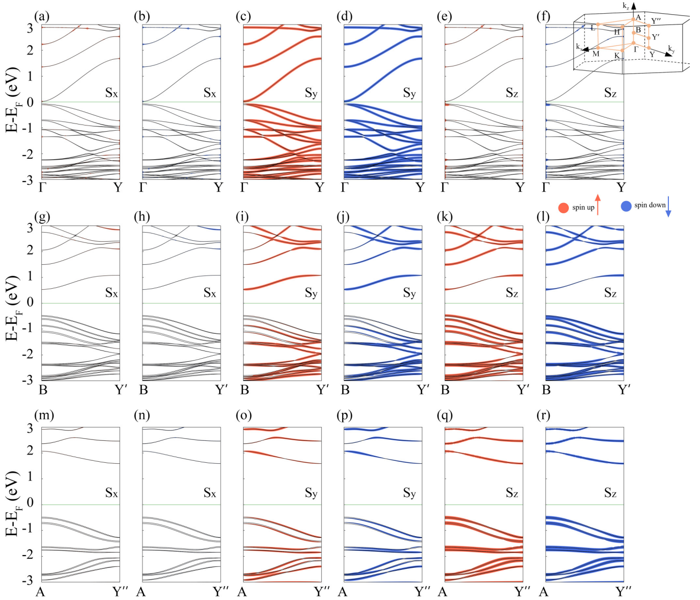
FIG. 16. Spin components of the energy bands in the FEC-1 structure of \text{NaCu}_5\text{S}_3 along \Gamma - Y , B - Y' , and A - Y'' k paths. Inset: Brillouin zone of \text{NaCu}_5\text{S}_3 illustrating the \Gamma - Y , B - Y' , and A - Y'' k paths.
