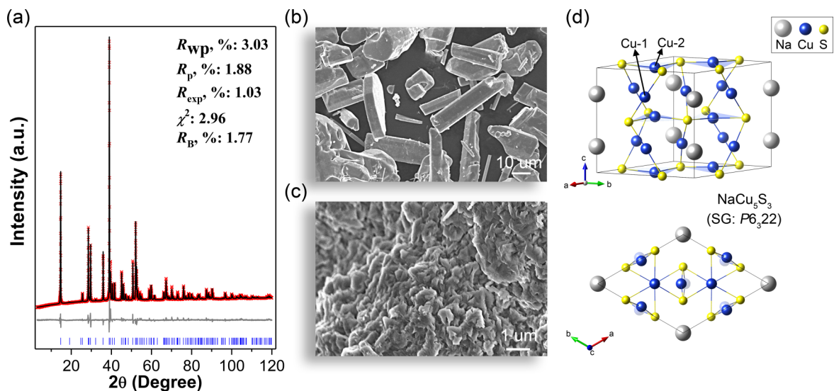
FIG. 3. Experimentally synthesized \text{NaCu}_5\text{S}_3 . (a) Rietveld fit to PXRD data. (b) Typical SEM image of as-prepared \text{NaCu}_5\text{S}_3 microcrystals. (c) SEM image of bulk \text{NaCu}_5\text{S}_3 obtained by the SPS sintering at 500 °C with high relative density of 96%. (d) Crystal structure of \text{NaCu}_5\text{S}_3 ( P6_322 ) with two unique Cu atoms (Cu-1 and Cu-2). One Cu-1 (Cu-2) atom becomes another under the C_3 ( C_2 ) symmetry operation with the rotation axis coinciding with the Cu-2 (Cu-1) sites.
