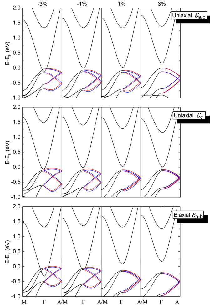
FIG. 18. Band structure evolution of NaCu 5 S 3 (FEC-1) with uniaxial/biaxial strain along a/b/c lattice directions from DFT + U ( U = 6 eV) with SOC. The applied strain from left to right is -3\% , -1\% , 1\% , and 3\% , respectively, where positive and negative values indicate tensile and compressive strain.
