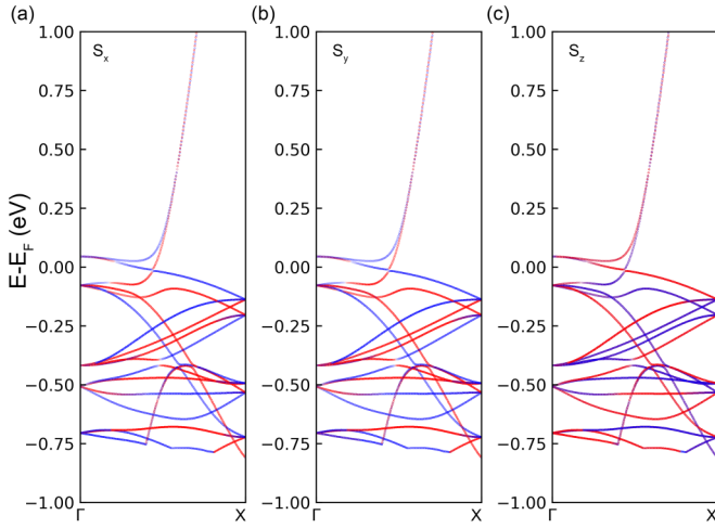
FIG. 14. Band structure of zinc-blende CuF with spin projections.
