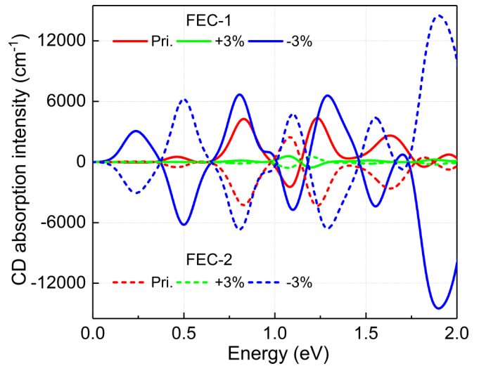
FIG. 5. Simulated circular dichroism absorption spectrum of the pristine and strained FEC-1 and FEC-2 orientations of NaCu 5 S 3 .
