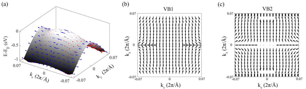
FIG. 13. Spin texture of the FEC-1 structure of \text{NaCu}_5\text{S}_3 in a wide k range around the \Gamma point for VB1 and VB2 (in comparison to Fig. 15(a) in a narrow k range).
