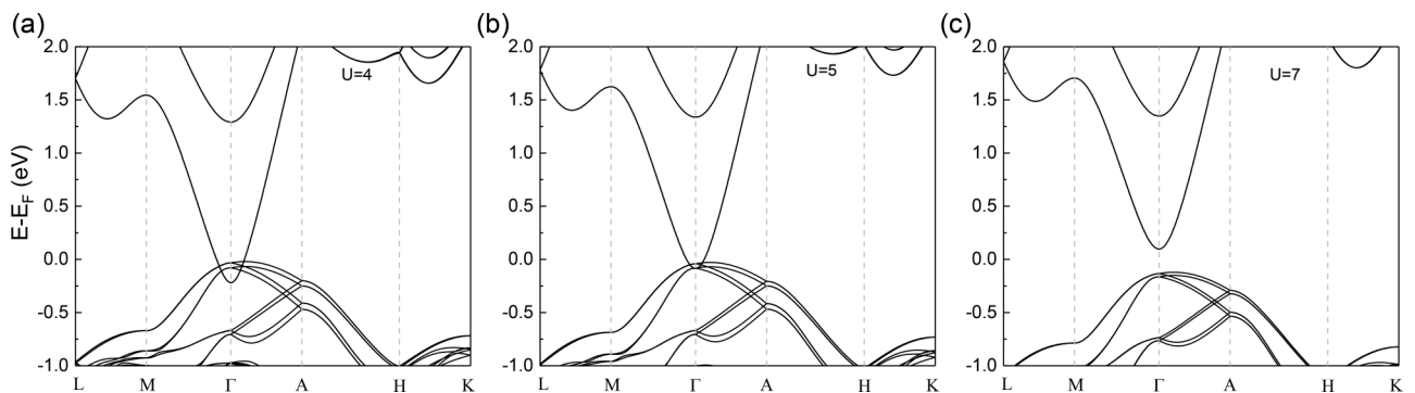
FIG. 11. Band structures of \text{NaCu}_5\text{S}_3 with P6_322 symmetry from DFT + U without SOC with different U values: (a) U = 4 \text{ eV} , (b) U = 5 \text{ eV} , and (c) U = 7 \text{ eV} .
