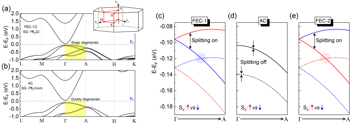
FIG. 6. D-1B Dresselhaus spin splitting in \text{NaCu}_5\text{S}_3 . (a), (b) Band structures for \text{NaCu}_5\text{S}_3 with P6_322 and P6_3/mcm symmetries calculated by DFT + U + SOC. Inset: The Brillouin zone of the hexagonal structures. (c)–(e) Detailed band structure information near the VBM along the \Gamma - A k line for the antichiral (AC) and ferri-chiral (FEC-1 and FEC-2) orientations of \text{NaCu}_5\text{S}_3 . Red/blue colors in (c) and (e) indicate the spin projection with the spin polarization axis along the z direction.
