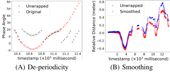
Fig. 2. RF phase signal preprocessing and the relative distance trajectory where \phi_L represents the corresponding phase change over the signal travel distance, c is the speed of light and f is the signal frequency (equals to 920MHz for our reader). Note that with the current COTS devices, we can not calculate the exact distance of the tag. There are two reasons. One is that in addition to the phase \phi_L over distance, both the reader and tag's circuits will introduce some additional phase rotations to the received phase \phi , i.e., \phi = (\phi_L + \phi_R + \phi_T) \bmod 2\pi , where \phi_R and \phi_T are the additional phases of the reader and tag respectively [13], [19]. Another reason is that our commercial RFID reader (Impinj R420) also introduces \pi radians of ambiguity. In other words, the reported phase can either be the true phase or the true phase plus \pi radians [19]. Hence for our reader, \phi_L = n\pi + \phi - (\phi_R + \phi_T) , where n is a non-negative integer. Since \phi_R and \phi_T are constant over the whole reading period, to estimate the motion of the tag over time, we only consider the relative distance changes of the tag, i.e.,
