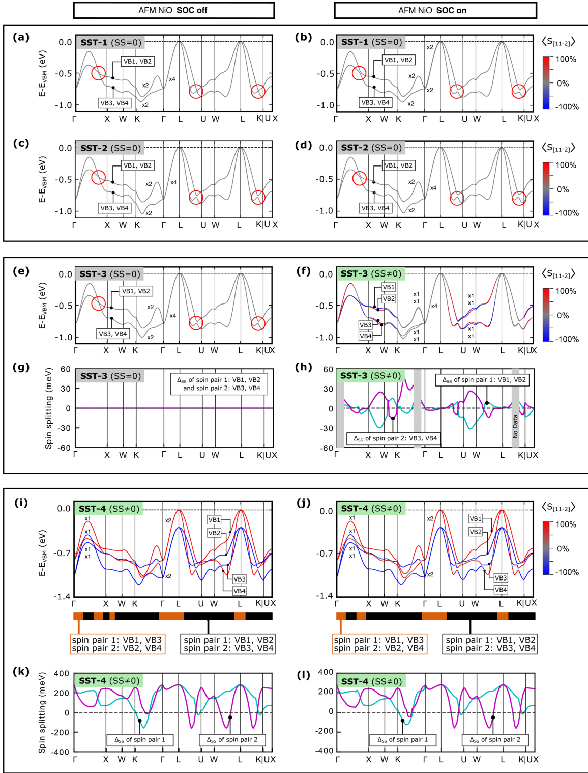
FIG. 3. DFT-calculated spin-polarized band structures and spin splitting of the top four valence bands in AFM NiO prototypes (SSTs) defined in Fig. 1: (a), (b) for SST-1 (no-spin-splitting case) with SOC off (a) and SOC on (b); (c), (d) for SST-2 (no-spin-splitting case) with SOC off (c) and SOC on (d); (e), (f), (g), (h) for SST-3 (SOC-induced spin-splitting case) of the four spin-polarized bands with SOC off (e) and SOC on (f); and the spin splitting with SOC off (g) and SOC on (h); and (i), (j), (k), (l) SST-4 (AFM-induced spin splitting) of the four spin-polarized bands with SOC off (i) and SOC on (j); and the spin splitting with SOC off (k) and SOC on (l). The top four valence bands of NiO prototypes are labeled in the order of decreasing band energy as VB1, VB2, VB3, and VB4, regardless of band crossing or anticrossing (red circles). These bands are grouped into two spin pairs (1 and 2) of neighboring bands with opposite spin polarization (see Appendix D for details). The grouping can be either spin pair 1 consisting of VB1 and VB2 and spin pair 2 consisting of VB3 and VB4, indicated by black regions in panels (k) and (l), or spin pair 1 consisting of VB1 and VB3 and spin pair 2 consisting of VB2 and VB4, indicated by orange regions in panels (k) and (l). The color bars on the right-hand side provide the spin projection on the magnetization direction [11\bar{2}] .
