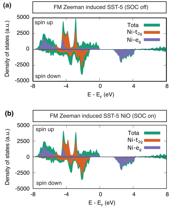
FIG. 4. DFT results of spin and orbital-projected density of states showing Zeeman splitting in FM SST-5. The spin-projected (up and down; identified by the spin projection on the magnetization direction [11\bar{2}] ) and orbital-projected ( \text{Ni-}t_{2g} and \text{Ni-}e_g ) density of states of FM SST-5 (a) when SOC is off and (b) when SOC is on.
