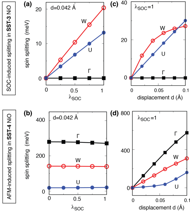
FIG. 2. Spin splitting of valence bands (the first spin pair) as a function of spin-orbit coupling strength \lambda_{\text{SOC}} for (a) relativistic SOC-induced splitting in the presence of AFM (SST-3) and (b) nonrelativistic AFM-induced splitting (SST-4) using a fixed displacement d = 0.042 \text{ \AA} along [111] direction, and as a function of displacement d for (c) relativistic SOC-induced splitting in the presence of AFM (SST-3) and (b) nonrelativistic AFM-induced splitting (SST-4) with fixed SOC strength \lambda_{\text{SOC}} = 1 .
