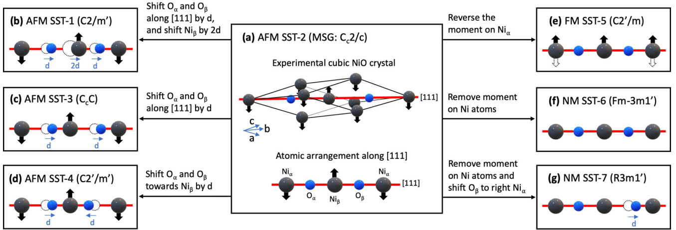
FIG. 1. Schematic diagrams of NiO atomic and magnetic structures for the seven spin-splitting prototypes. The models are uniquely represented by the atomic arrangement along the [111] direction (indicated by the red line) and the magnetic ordering on Ni (indicated by black arrows) in the unit cell. Here we have used the observed magnetization direction [112̄]. Ni α and Ni β (black circles) are the two Ni sites, and O α and O β (blue circles) are the two oxygen sites. Open and solid circles indicate, respectively, atomic positions before and after displacements d . (a) The experimentally observed AFM cubic phase of NiO belongs to spin-splitting prototype 2 (SST-2). The other six prototypes (b)–(g) are derived from the AFM rocksalt NiO experimental magnetic structure (AFM SST-2) by local distortions and flip/removal of magnetic moments.
