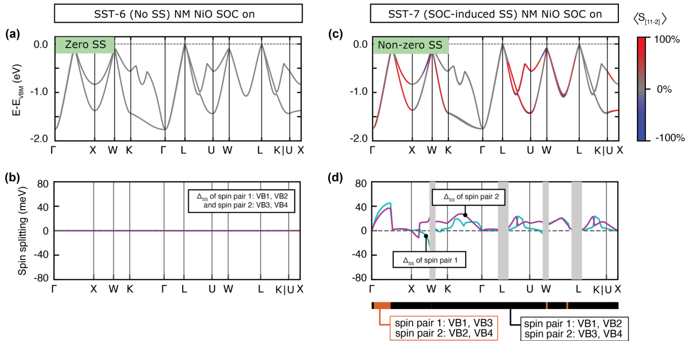
FIG. 5. Spin-polarized energy bands and spin splitting of the top four valence bands in nonmagnetic NiO prototype structures: (a) spin-polarized bands and (b) spin splitting for centrosymmetric SST-6 with SOC on; (c) spin-polarized bands and (d) spin splitting for noncentrosymmetric SST-7 with SOC on.
