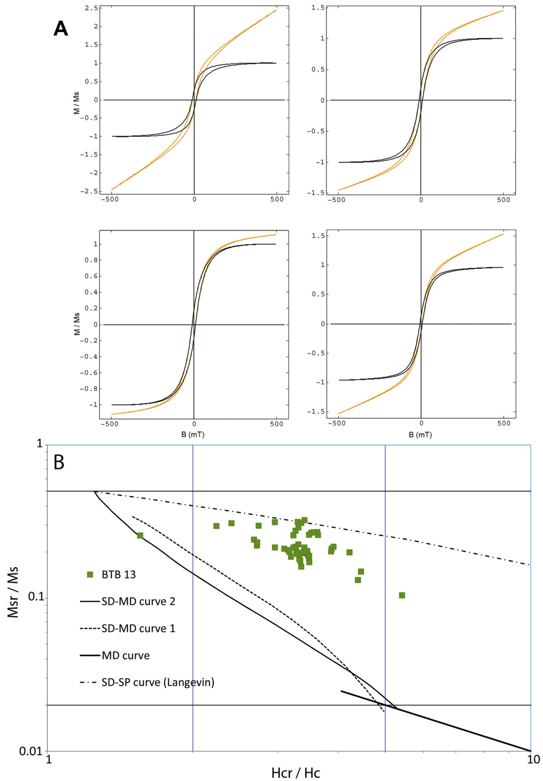
Fig. 3. A) Hysteresis curves before (light brown) and after (black) correction of paramagnetic contribution for samples BTB13-1A-50Q-3-2 (146.64 mbs), BTB13-1A-68Q-3-2 (196.17 mbs) and BTB13-1A-43Q-1-102 (123.44 mbs), BTB13-1A-7Q-2-58 (23.86 mbs). B) Day plot of M_{sr}/M_s and H_{cr}/H_c ratios. Data points from the BTB13 core are indicated by green squares. The solid and dashed lines represent mixing curves of Dunlop (2002a, 2002b), with SD = single domain, SP = superparamagnetic, and MD = multidomain. The data points (green squares) are from the BTB13 core. SD range: M_{sr}/M_s 0.5 to 1 and H_{cr}/H_c 1 to 2, PSD range: M_{sr}/M_s 0.5 to 0.04 and H_{cr}/H_c 2 to 5, MD range: M_{sr}/M_s 0 to 0.04 and H_{cr}/H_c > 5 . (For interpretation of the references to colour in this figure legend, the reader is referred to the web version of this article.)
