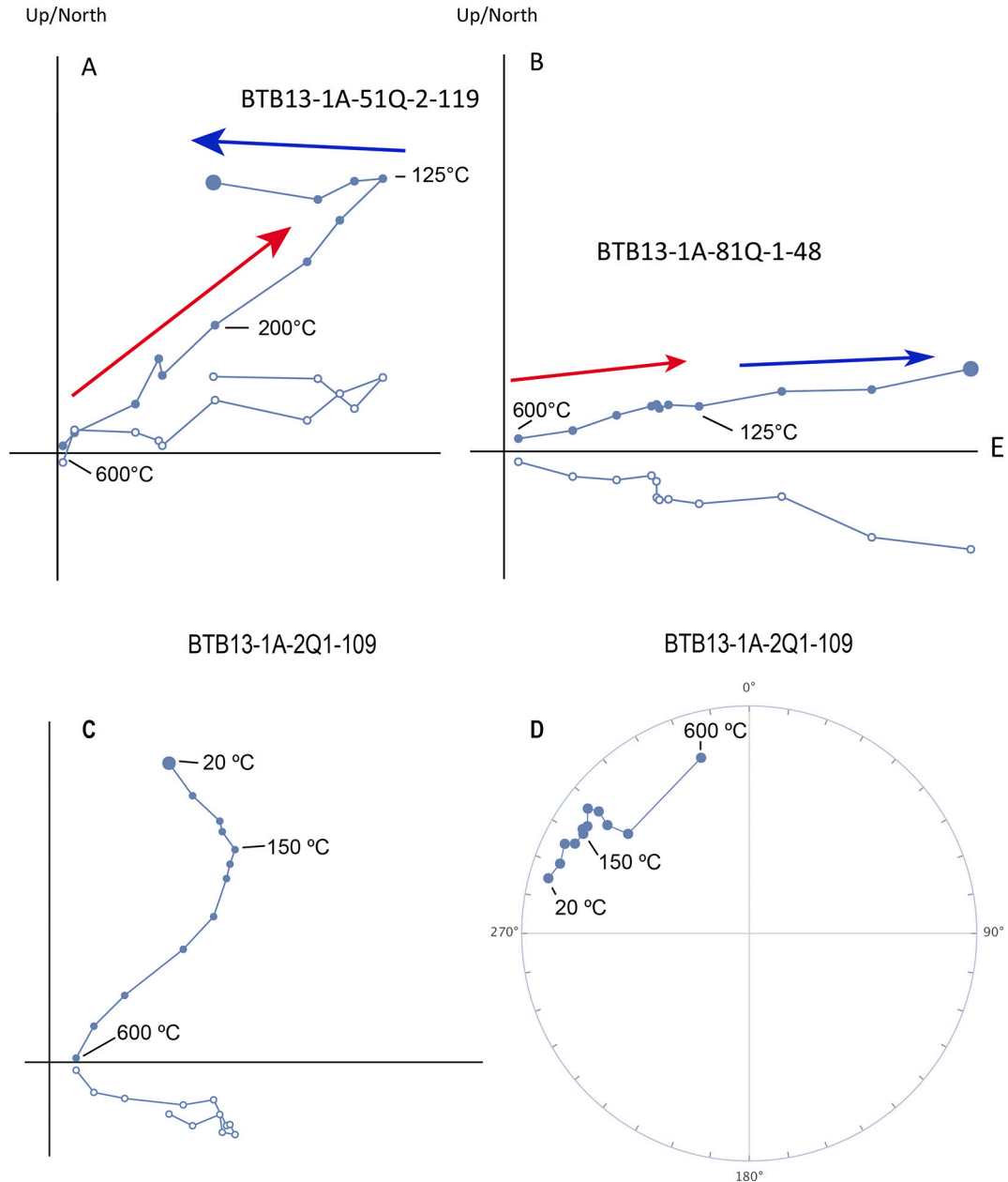
Fig. 5. A) and B) Typical Zijderveld (1967) diagrams (closed/open circles denote projection on a horizontal/vertical plane) of thermal demagnetizations showing the low temperature component (blue arrow) interpreted as a secondary component in a normal polarity direction and the higher temperature component (red arrow) interpreted as a primary component in either reversed (A) or normal (B) polarity. C) and D) One example of a sample for which the low temperature and higher temperature components were overlapping and not fully separated upon thermal demagnetization. In this case a great circle analyses was performed on stereographic projection (D). (For interpretation of the references to colour in this figure legend, the reader is referred to the web version of this article.)
