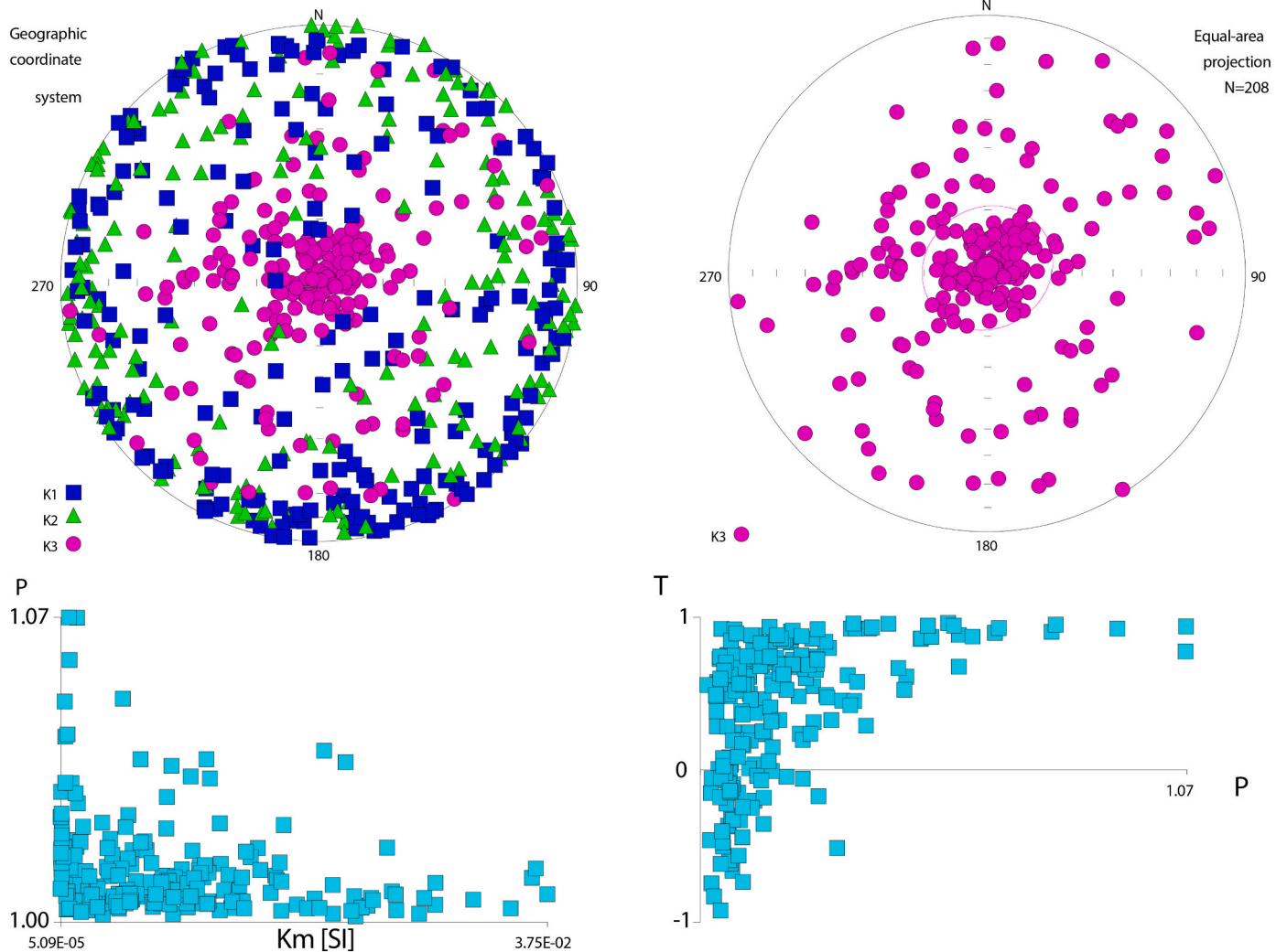
Fig. 4. A) Anisotropy of Magnetic Susceptibility (AMS) results from BTB13 samples showing maximum (K1), intermediate (K2) and minimum (K3) axes directions. B) Minimum K3 axis only. C) P, the degree of AMS (K1/K3) plotted against Km, the mean susceptibility. D) Shape parameter T plotted against P the degree of AMS (K1/K3). Figure made using Anisofort42 software.
