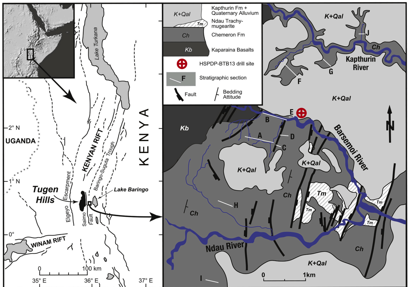
Fig. 1. Map of the Baringo area with geological setting, top left insert shows topographic map of East Africa. Location of BTB13 site (latitude 0.5546 N, longitude 35.9375E). Stratigraphy of this figure is described in Deino et al., 2006 and Kingston et al., 2007.
