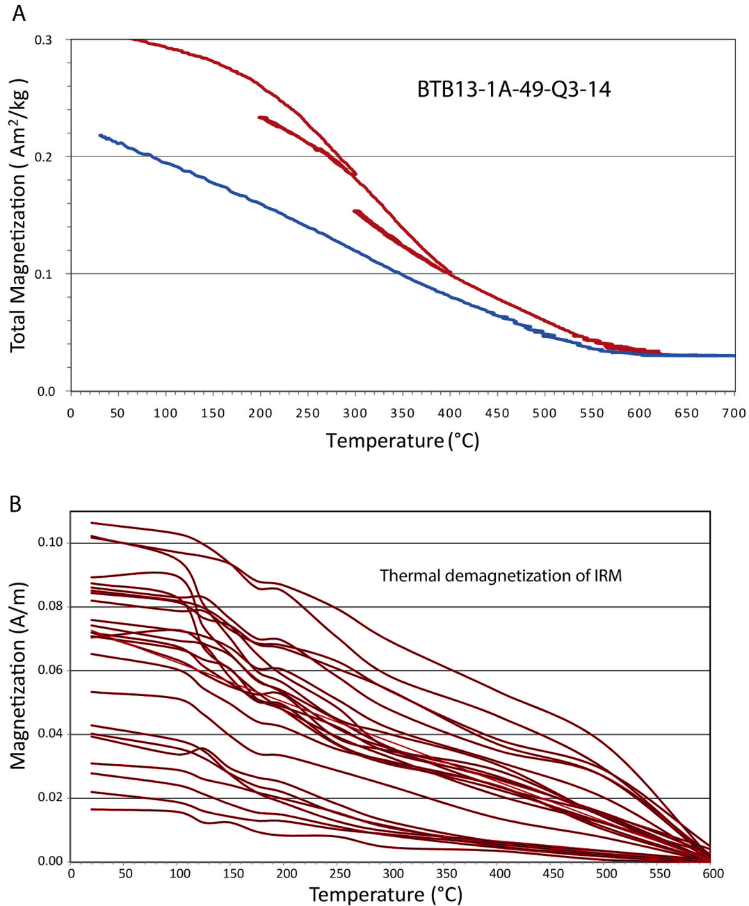
Fig. 2. A) Thermomagnetic experiment showing the typical high-field magnetic moment upon heating (red) and subsequent (blue) cooling in successive temperature ranges measured on Curie balance. Sample BTB13-1A-49Q-3-14 has a depth of 142.99 mbs. B) Thermal demagnetizations of Isothermal Remanent Magnetizations acquired by applying 1T in one direction and then 0.3T in the opposite direction. (For interpretation of the references to colour in this figure legend, the reader is referred to the web version of this article.)
