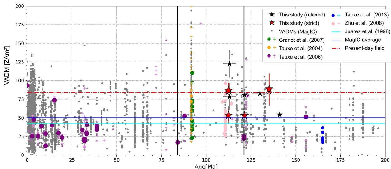
Figure 6. VADM (in \text{ZAm}^2 ) versus age (Ma). The black and red stars are the results of this Costa Rica study obtained using the CCRIT-relaxed and -strict selection criteria, respectively, with 1\sigma error bars and ^{40}\text{Ar} - ^{39}\text{Ar} ages with 2\sigma error bars. Gray dots represent the virtual (axial) dipole moments ( V[A]DM ) available from the MagIC database spanning the last 200 Ma. The bounds of the Cretaceous Normal Superchron (CNS) are indicated with vertical black lines. The strength of the present dipole field is shown as a dashed red line, the solid blue line represents the average of all the MagIC data, and the long-term average from Juarez and Tauxe (2000), and Tauxe et al. (2013) is shown as a solid aquamarine line. Circles represent the data from SBGs that we re-analyzed using the same CCRIT criteria as employed in our study, while the original literature data as presented by the authors are marked as crosses. SBG, submarine basaltic glass; VADM, Virtual Axial Dipole Moment.
