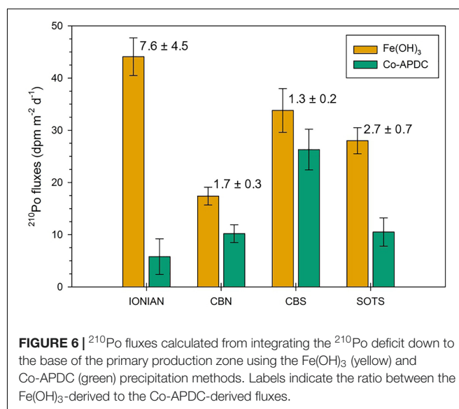
FIGURE 6 | ^{210}\text{Po} fluxes calculated from integrating the ^{210}\text{Po} deficit down to the base of the primary production zone using the \text{Fe}(\text{OH})_3 (yellow) and Co-APDC (green) precipitation methods. Labels indicate the ratio between the \text{Fe}(\text{OH})_3 -derived to the Co-APDC-derived fluxes.
