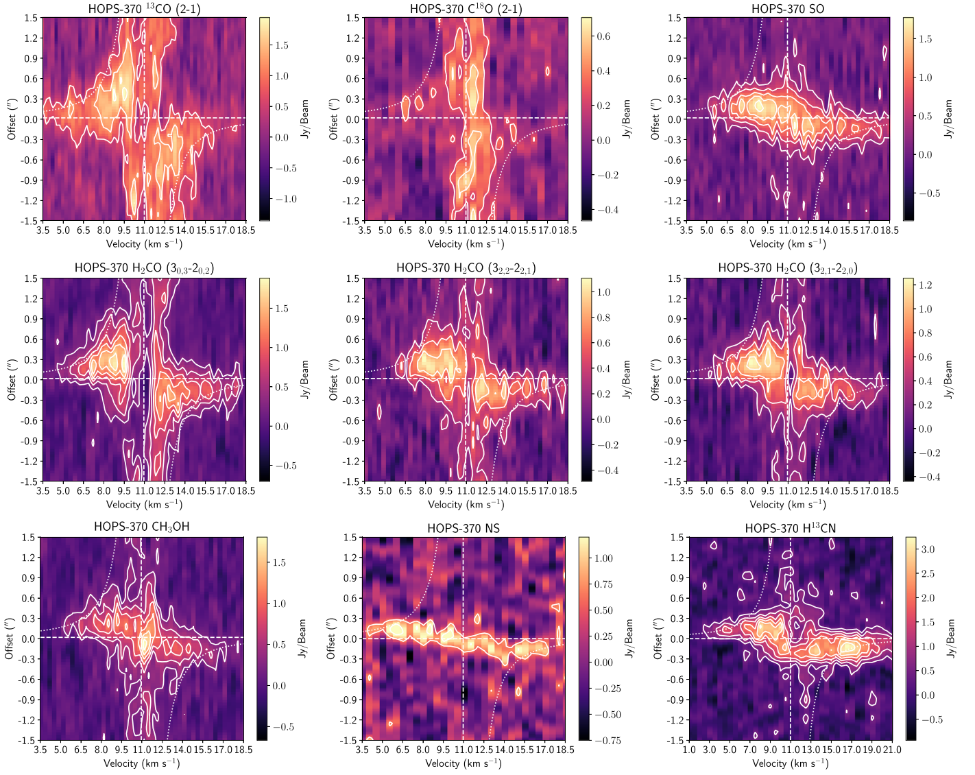
Figure 6. PV diagrams of the molecular line emission taken across the major axis of the disk, summed within a 0''.6 strip. The rotation signature of the disk is evident on scales less than \pm 1'' at blue- and redshifted velocities. The emission on scales > 1'' between velocities of \sim 9.5 and 13 \text{ km s}^{-1} corresponds to emission from the cloud/envelope that is not well recovered in these observations. The \text{C}^{18}\text{O} emission, however, is dominated by an extended, low-velocity component, and the higher-velocity disk emission is only marginally detected. The white dashed line shows the source velocity at \sim 11 \text{ km s}^{-1} , and the white dotted line is the Keplerian velocity curve for a 2.5 M_{\odot} protostar drawn for comparison. The contours drawn start at and increase on 5\sigma intervals, where \sigma is \sim 4\times the image rms from Table 1.
