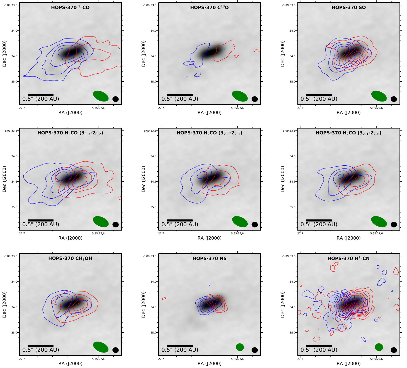
Figure 5. ALMA integrated intensity images of the molecular lines at blue- and redshifted velocities overlaid with their corresponding contour colors and overlaid on the 0.87 mm continuum (gray scale). The red- and blueshifted emission shows a clear rotation pattern in the disk that is consistent for all molecules. The integrated intensity maps for many molecules have their emission peaks spatially located above and below the continuum emission, which could be related to continuum or line opacity. The NS molecule, in contrast, does not seem to avoid the disk midplane. The blueshifted images are typically integrated between 4 and 11 km s -1 , while the redshifted images are typically integrated between 11 and 18 km s -1 . The contours plotted start at 5σ and increase on 5σ intervals for the three H 2 CO transitions, SO, and CH 3 OH, where σ = 24 mJy beam -1 . The contour levels for the other transitions are as follows: NS starts at 3σ and increases on 2σ intervals, where σ = 38 mJy beam -1 ; 13 CO starts at 3σ and increases on 2σ intervals, where σ = 61 mJy beam -1 ; C 18 O starts at 2σ and increases on 1σ intervals, where σ = 36 mJy beam -1 ; and H 13 CN starts at 4σ and increases on 4σ intervals, where σ = 33 mJy beam -1 . The green ellipse denotes the beam for the molecular line data, which is ~0''.23 × ~0''.13 (90 au × 51 au) for all but NS and H 13 CN, whose beams are 0''.15 × 0''.14 (59 au × 55 au). The black ellipse denotes the beam for the 0.87 mm continuum data 0''.11 × 0''.10 (43 au × 39 au).
