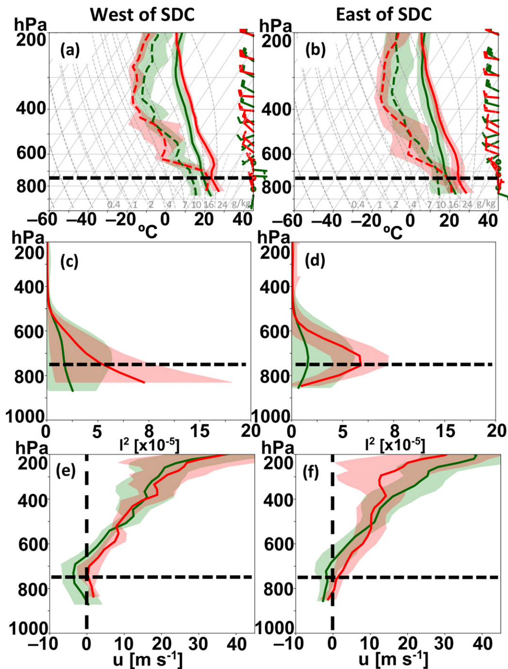
FIG. 12. Mean Null (red) and CI + Fail (dark green) (a),(b) soundings; (c),(d) Scorer parameter profiles; and (e),(f) zonal wind profiles (a),(c),(e) west of the SDC and (b),(d),(f) east of the SDC. The horizontal dashed line in all panels denotes the approximate peak terrain height. The vertical dashed line in (e) and (f) denote u = 0 \text{ m s}^{-1} . The standard deviations are shaded. Due to relatively few soundings for the Null category, the standard deviation for the Scorer parameter in (c) and (d) do not include highly erroneous outlier data greater than 40 \times 10^{-5} \text{ m}^{-2} (less than 2% of the data).
