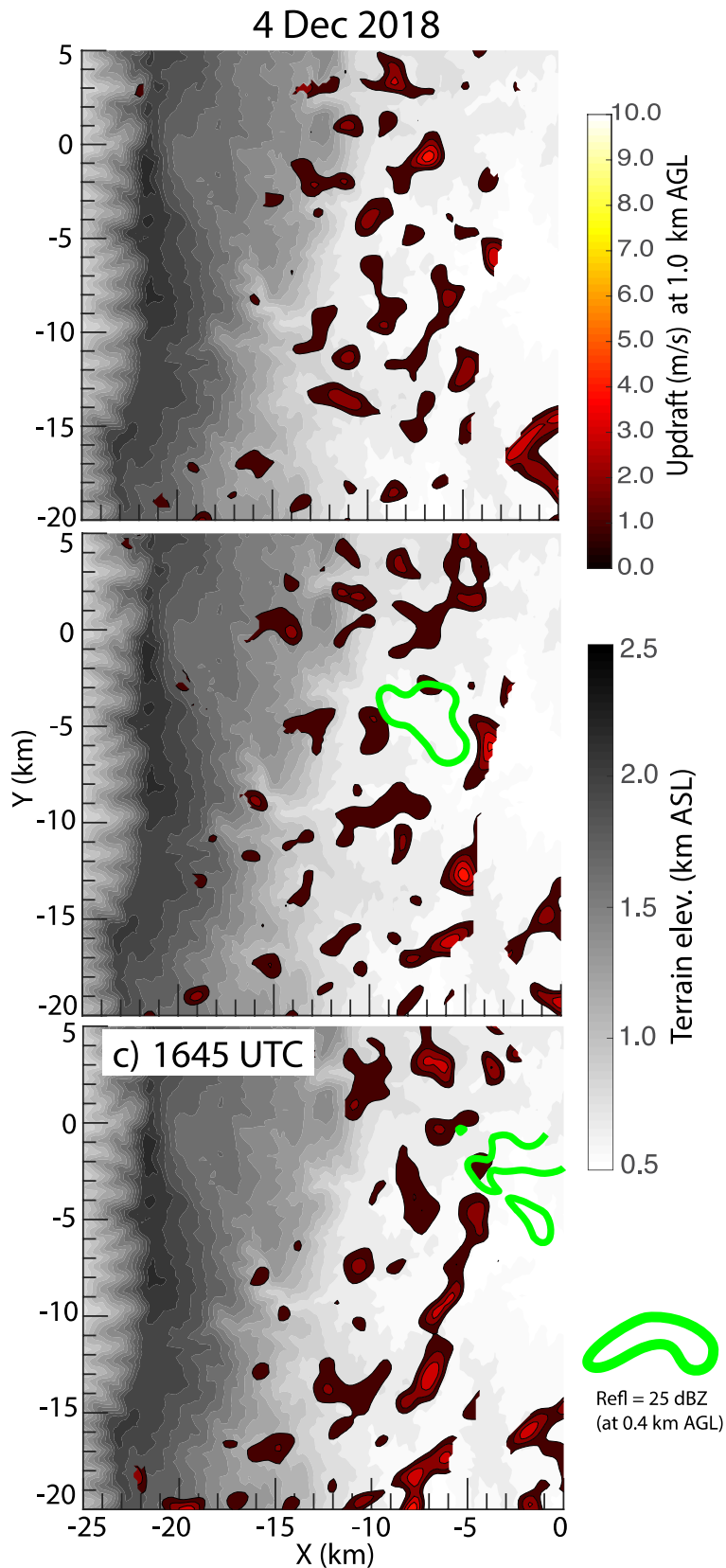
Figure 12: Same as Fig. 11 except valid between 1615-1645 UTC on 4 December 2018. Updrafts are shown at z = 1.0 km AGL because of the vertical coverage of available dual-Doppler data.
