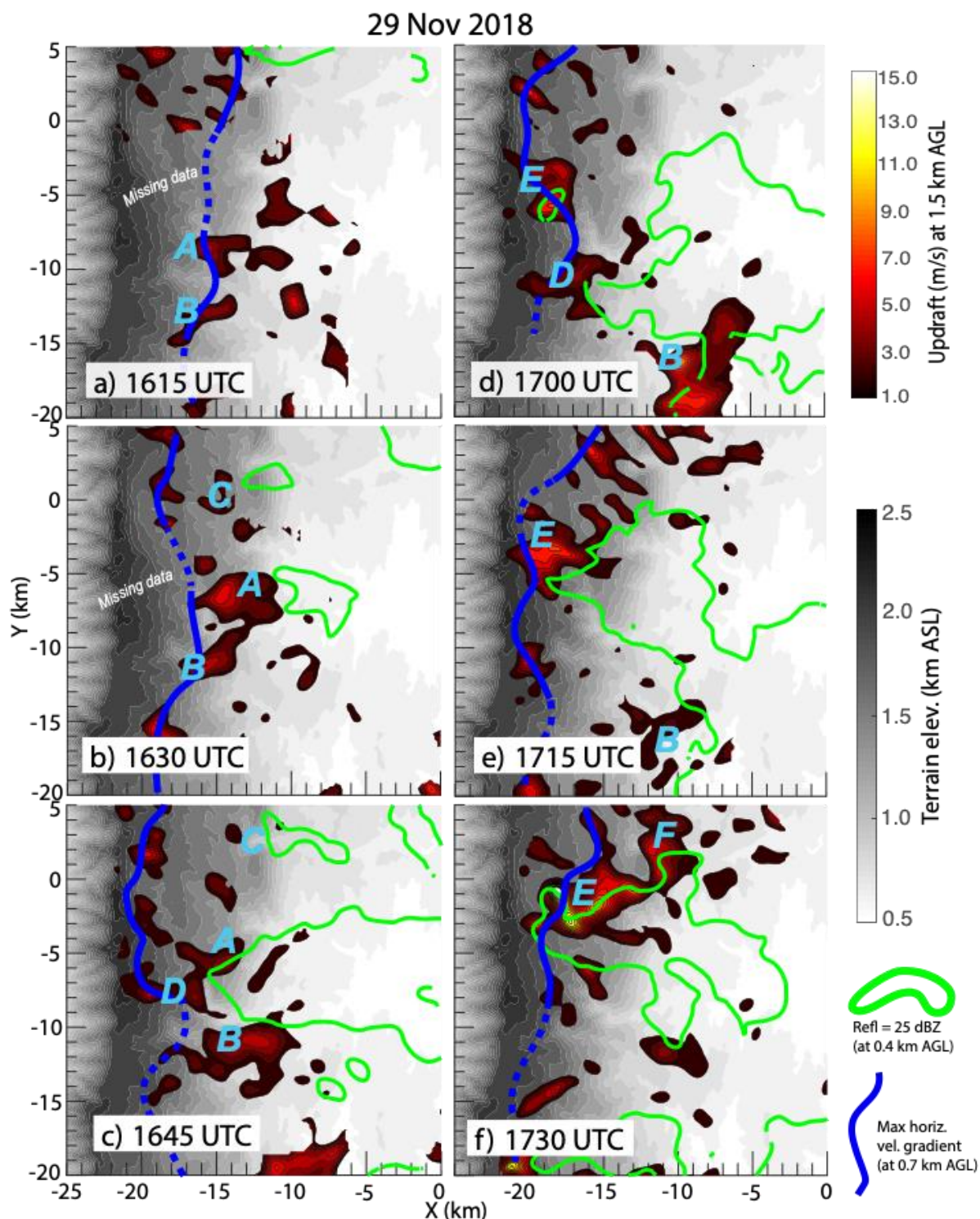
Figure 11. Dual-Doppler-retrieved vertical velocity at z = 1.5 km AGL (red-yellow shaded) and DOW radar reflectivity at z = 400 m AGL (25 dBZ; green contour) between 1615-1730 UTC on 29 November 2018. Terrain elevation is gray shaded. Subjectively tracked precipitating updrafts described in section 4 are labeled 'A'-'F'. Subjective trace of the maximum horizontal velocity gradient tensor at z = 700 m
