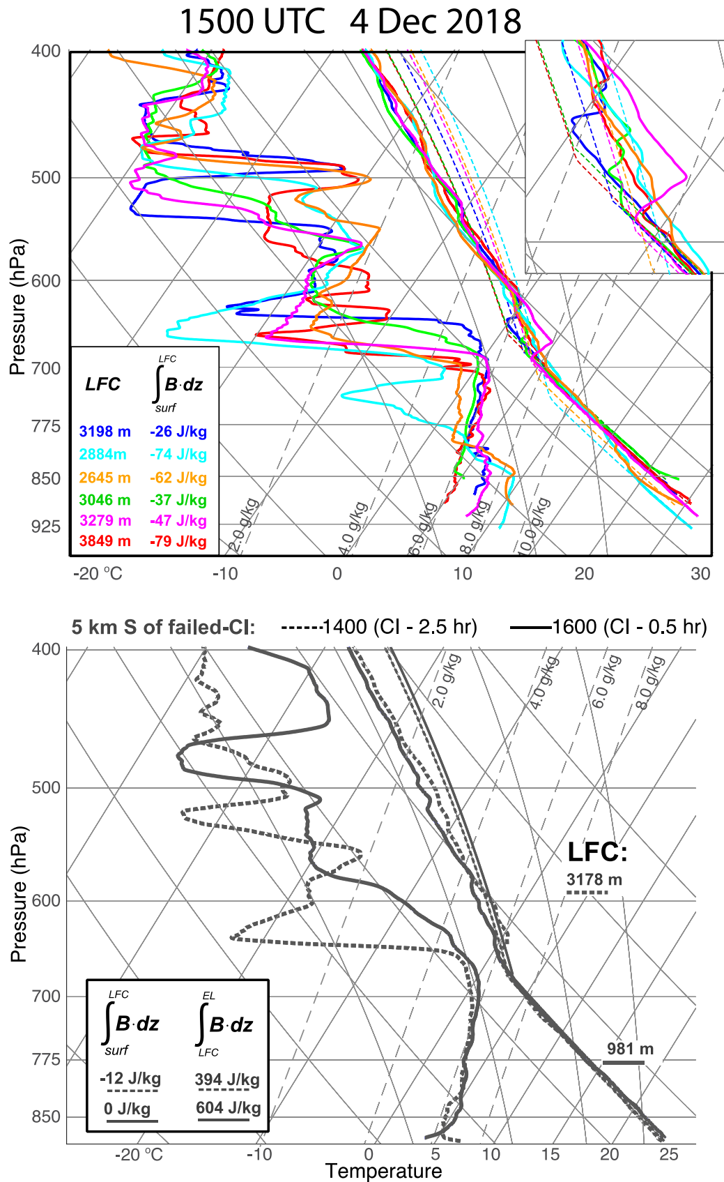
Figure 7. (a) Same as Fig. 6, except for the 4 December 2018 case. Soundings are colored to match launch sites shown in Fig. 1b. The area of the soundings between the LCL and LFC is enlarged in an
