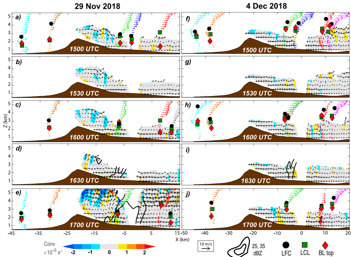
Figure 5. Cross sections of dual-Doppler meridional-mean zonal and vertical wind (vectors), horizontal convergence (shaded), and DOW radar reflectivity (25 and 35 dBZ, thick black contours) between 1500-1700 UTC on 29 November 2018 (a-e) and 4 December 2018 (f-j). Radiosonde-measured horizontal winds (vector profiles colored to match launch sites shown in Fig. 1), boundary layer depth (red diamonds; measured as in Liu and Liang 2010 and Nelson et al. 2020), ML LCL (green boxes) and ML LFC (black circles) measured from hourly radiosondes are projected into the cross section. The meridional-mean terrain profile of the SDC is shown in brown.
