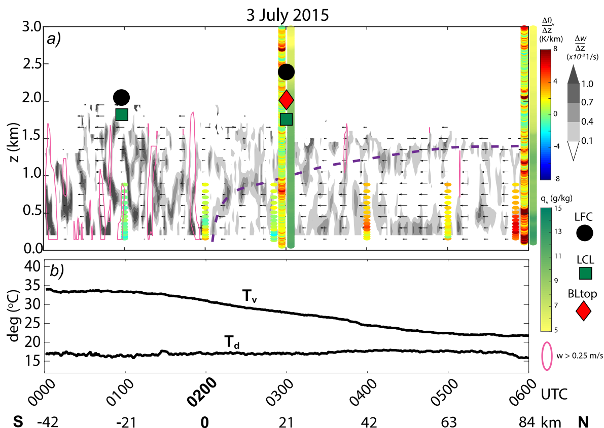
Figure 9. (a) Lidar-retrieved boundary-relative meridional wind profiles (vectors), the vertical gradient of lidar-measured vertical velocity approximating horizontal wind convergence (shaded), lidar-measured updraft ( > 0.25 \text{ m s}^{-1} ; magenta contour), AERI static stability profiles below z = 850 \text{ m} (shown hourly), and radiosonde static stability and q_v profiles from the 0300 and 0600 UTC radiosondes located at Ellis, Kansas. Radiosonde-estimated (and combined radiosonde-AERI-estimated at 0100 UTC) ML LCL (green boxes), ML LFCs (black circles), and the 0300 UTC boundary layer top (red diamond; calculated with the Liu and Liang 2010 method) are overlaid. (b) Surface virtual temperature and dew point temperature observations. Boundary-relative winds are calculated and meridional distance (horizontal axis) is time-space converted using the mean meridional motion of the boundary, v = -3.5 \text{ m s}^{-1} . Depth and slope of the wind shift boundary (purple dashed line) is subjectively estimated using wind, convergence, and radiosonde stability profiles.
