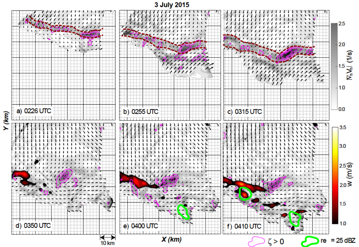
Figure 13: Radar reflectivity at z = 1 km AGL (25 dBZ; green contour), positive vertical vorticity (purple contours; outermost is 0.001 \text{ s}^{-1} , incremented by 0.001 \text{ s}^{-1} ), and updraft (red-yellow shading in panels d-f) at z = 1.25 km AGL, using dual-Doppler wind retrievals between 0226-0410 UTC on 3 July 2015. Horizontal velocity gradient tensor (gray shading) produced using quasi-2D dual-Doppler wind syntheses (as in Fig. 8). Subjective width of the boundary is highlighted with dashed purple contours in panels a-c.
