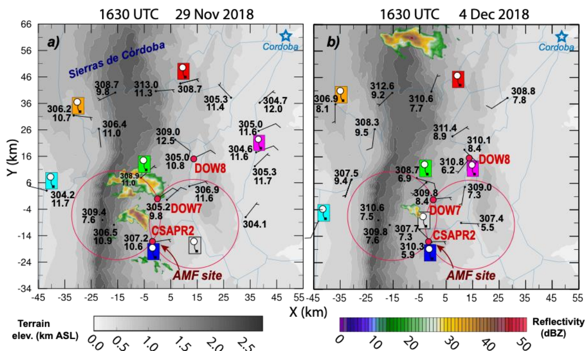
Figure 1. Instrument deployment maps for the 29 November 2018 (a) and 4 December 2018 (b) cases. Locations of the DOW 7, DOW 8, CSAPR2 radars, and dual-Doppler lobes are labelled in red. An array of surface observations from radiosondes, ARM surface stations (Kyrouac and Holdridge 2018), Pod surface stations (1 m height), mobile mesonets (3 m height) (Wurman and Kosiba 2021c,d) are shown in black ( \theta_v (K) and q_v (g/kg)) and DOW 7 radar reflectivity from the 3.5° beam elevation angle is shaded. Radiosonde launch locations are marked. Location of the ARM AMF site is annotated.
