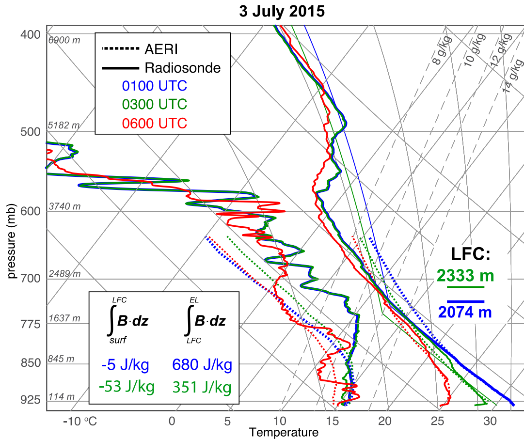
Figure 10. Skew-T/log-p diagrams from radiosonde and AERI measurements between 0100 – 0600 UTC on 3 July 2015. Radiosonde profiles are shown with solid lines and AERI profiles are shown with dashed lines. The solid blue profile is a combination of low-level AERI data valid at 0100 UTC and the 0300 UTC radiosonde aloft (described in the text). ML CIN and CAPE from 0100 and 0300 UTC are shown in the lower-left offset. ML LFC (AGL) is labeled on the right. For reference, the altitude above ground level (mean of each sounding) is shown along each potted pressure level.
